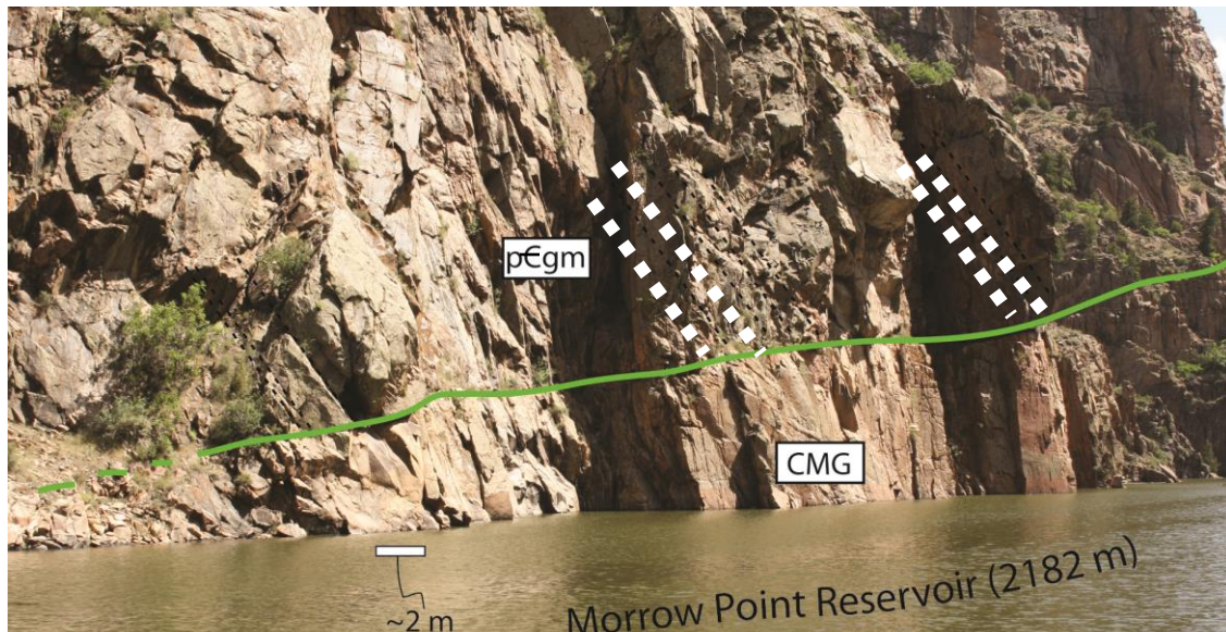
Figure 5-7. View to the southeast of Curecanti pluton roof (green line) as it dips beneath the Morrow Point Reservoir ~1 km east of Chipeta Falls. Note discordance of roof with respect to the foliation in the host rock (dashed white lines) and lack of xenoliths in the Curecanti pluton near the roof at this location.
