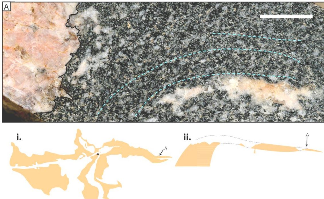
Figure 5-5. (A) Photograph (view to the east) of aplite veinlet (orientation: 271^{\circ} , 85^{\circ} N), near Chipeta Falls, cross cutting the host gneisses foliation (dashed blue lines), which is gently folded. This photograph was taken 10 m above the Curecanti pluton roof. Insets i. and ii. show location of A.
