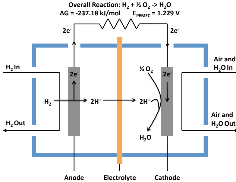
Figure 19. Schematic of Basic Fuel Cell Design
