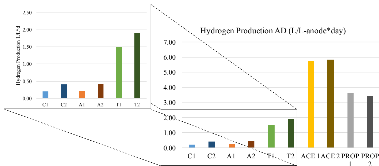
Figure 12. Hydrogen production rates in MECs fed with AD effluent and Control Runs. ACE and Propionate groups are control runs with 0.2 gCOD-eq/L.
