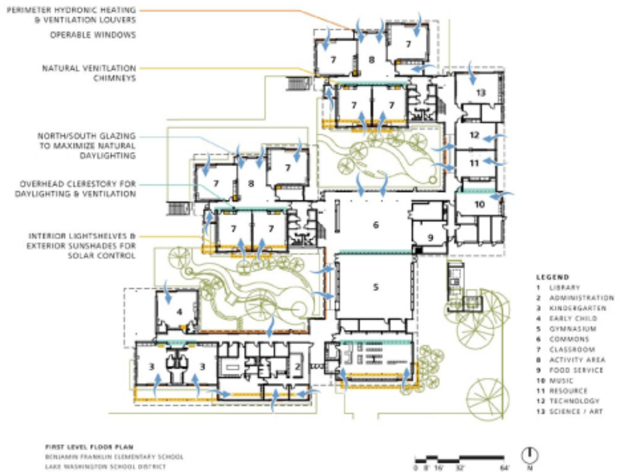
Figure 12: First Floor Plan of Ben Franklin Elementary School (Archinnovations.com, 2010)
