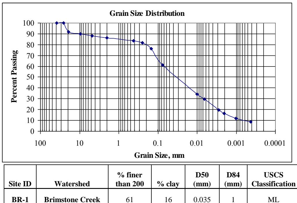
Figure B.2 Grain Size Distribution BR-1
