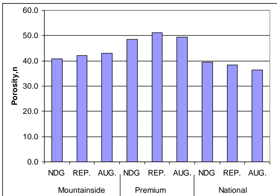
Figure IV.9 Porosity Calculations
