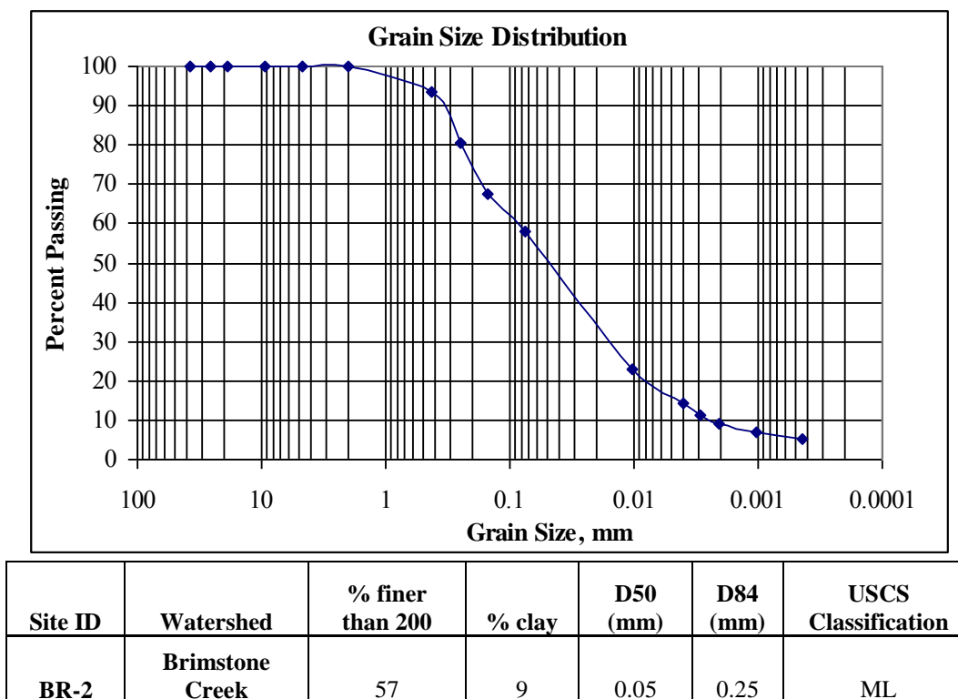
Figure B.3 Grain Size Distribution BR-2
