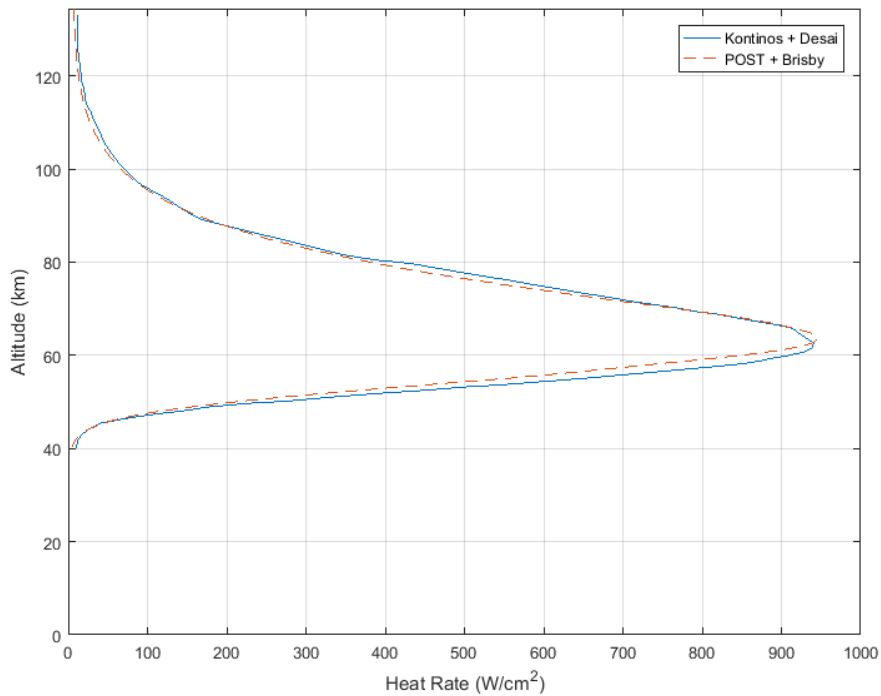
Figure 5: POST/Brisby Cross Validation with Kontinos/Desai, Altitude Versus Heat Rate
