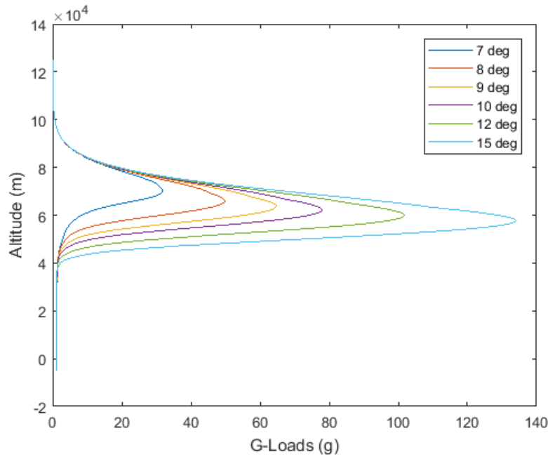
Figure 12: 20 cm Stardust Scale Acceleration at Altitude for Varying Entry Angles
