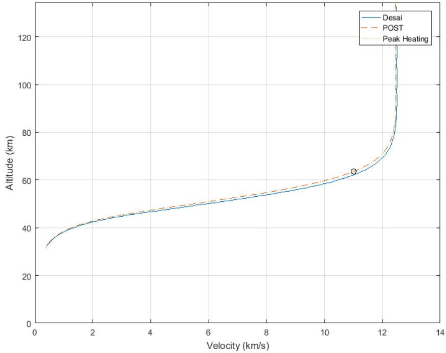
Figure 3: POST Validation Against Desai's Reconstruction, Altitude Versus Velocity
