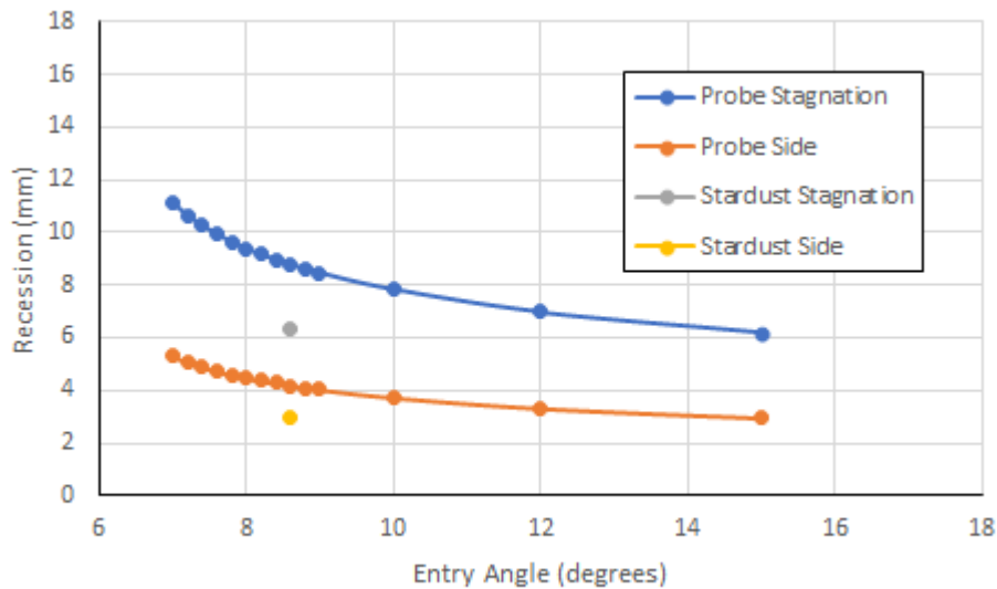
Figure 13: 20 cm Probe Heat Shield Recession Versus Entry Angle for Stardust Shape
