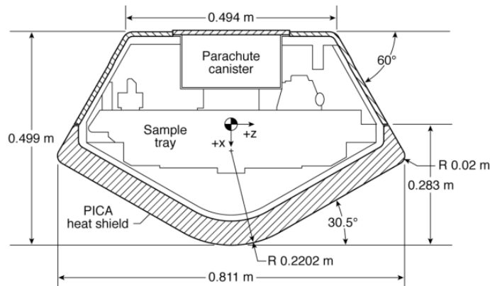
Figure 1: Diagram of the Stardust Entry Capsule
