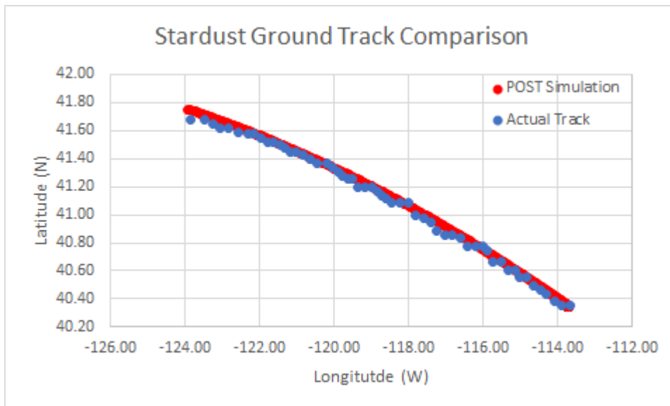
Figure 4: Stardust Simulated Versus Actual Ground Track
