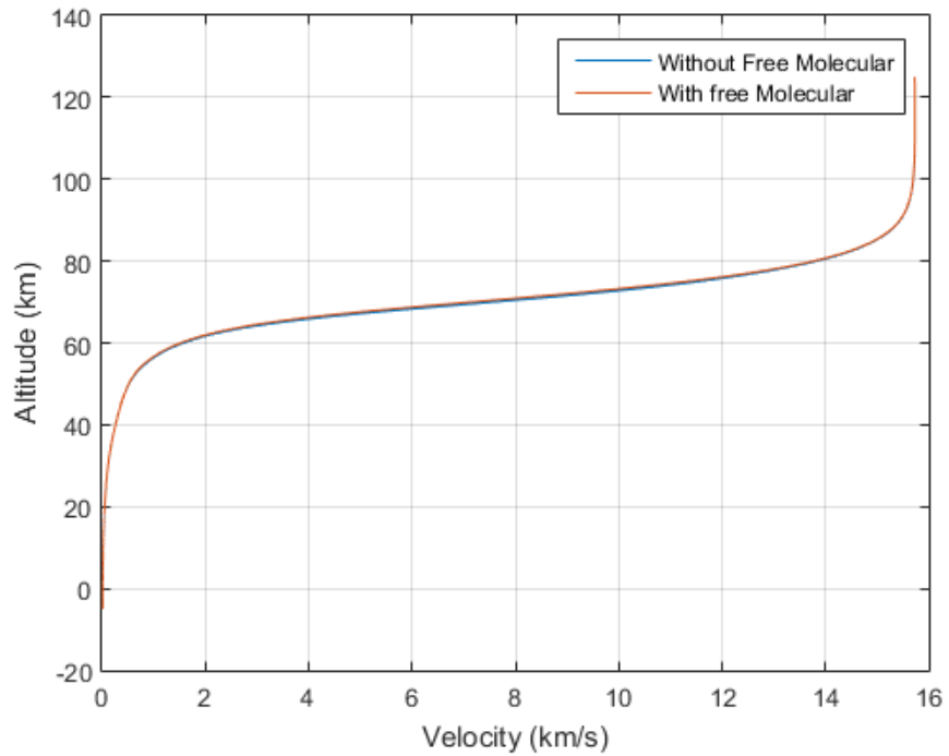
Figure 7: Comparison With and Without Free Molecular Regime Aerodynamics for a 10cm Diameter Body
