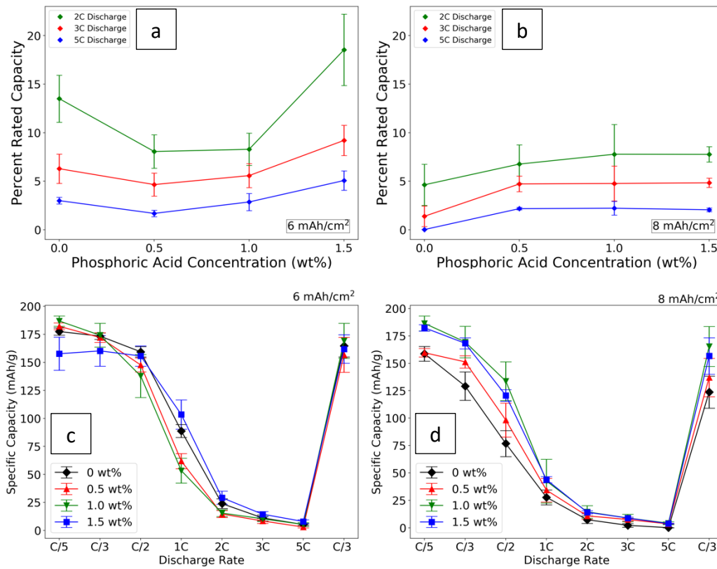
Figure 2. Percent of rated discharge capacity for various phosphoric acid (PA) concentrations for a) 6 mAh/cm 2 cathodes and b) 8 mAh/cm 2 cathodes; discharge rates of 2C, 3C, and 5C are shown in green, red, and blue traces respectively. Rate capability for c) 6 mAh/cm 2 cathodes and d) 8 mAh/cm 2 cathodes.
