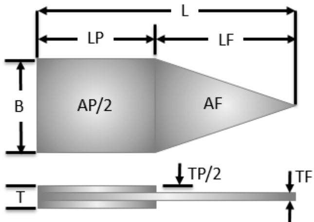
Figure 8. Actuator dimensions.
