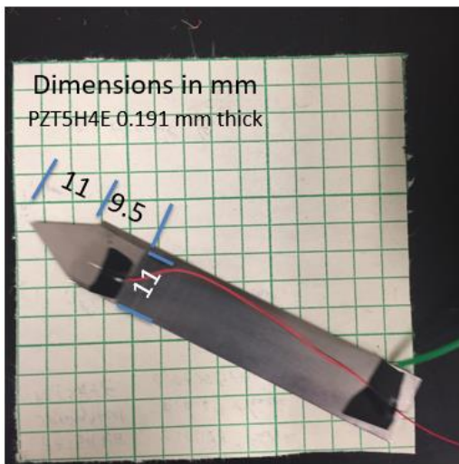
Figure 10. Unimorph actuator test articles.
