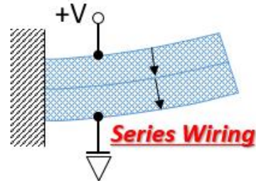
Figure 12. Bimorph actuator test articles with additional tunability.
