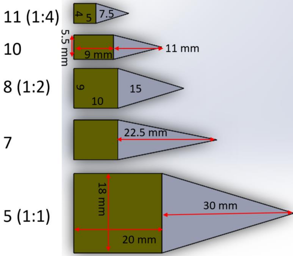
Figure 17. Variations in the shape of test article 5.
