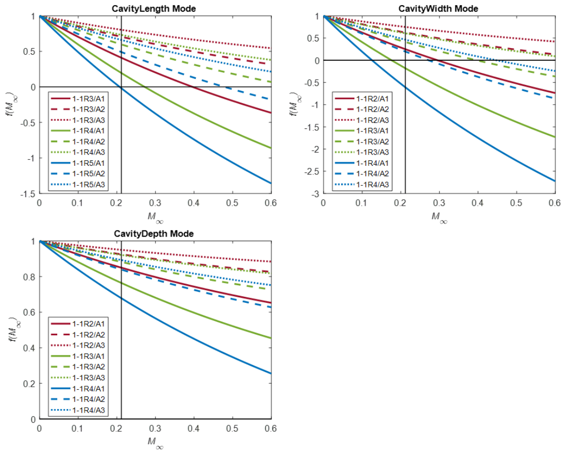
Figure 79. Coupling of cavity acoustic and cavity Rossiter tones near actuator frequency at Mach 0.2 test conditions.
