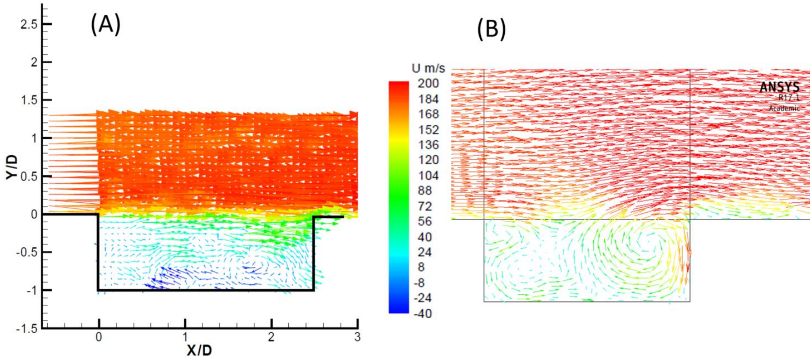
Figure 50. Qualitative comparison of instantaneous velocity vectors from Radhakrishnan’s experiment to CFD validation case. A) Sample of Radhakrishnan’s experimental data shown as velocity vectors colored by velocity magnitude at an instant in time. Two vortex regions can be seen inside the cavity. B) Sample from time-accurate CFD solutions from validation check cases showing velocity vectors colored by velocity magnitude at an instant in time. Two vortex regions of greater extent and higher velocity can be seen inside the cavity.
