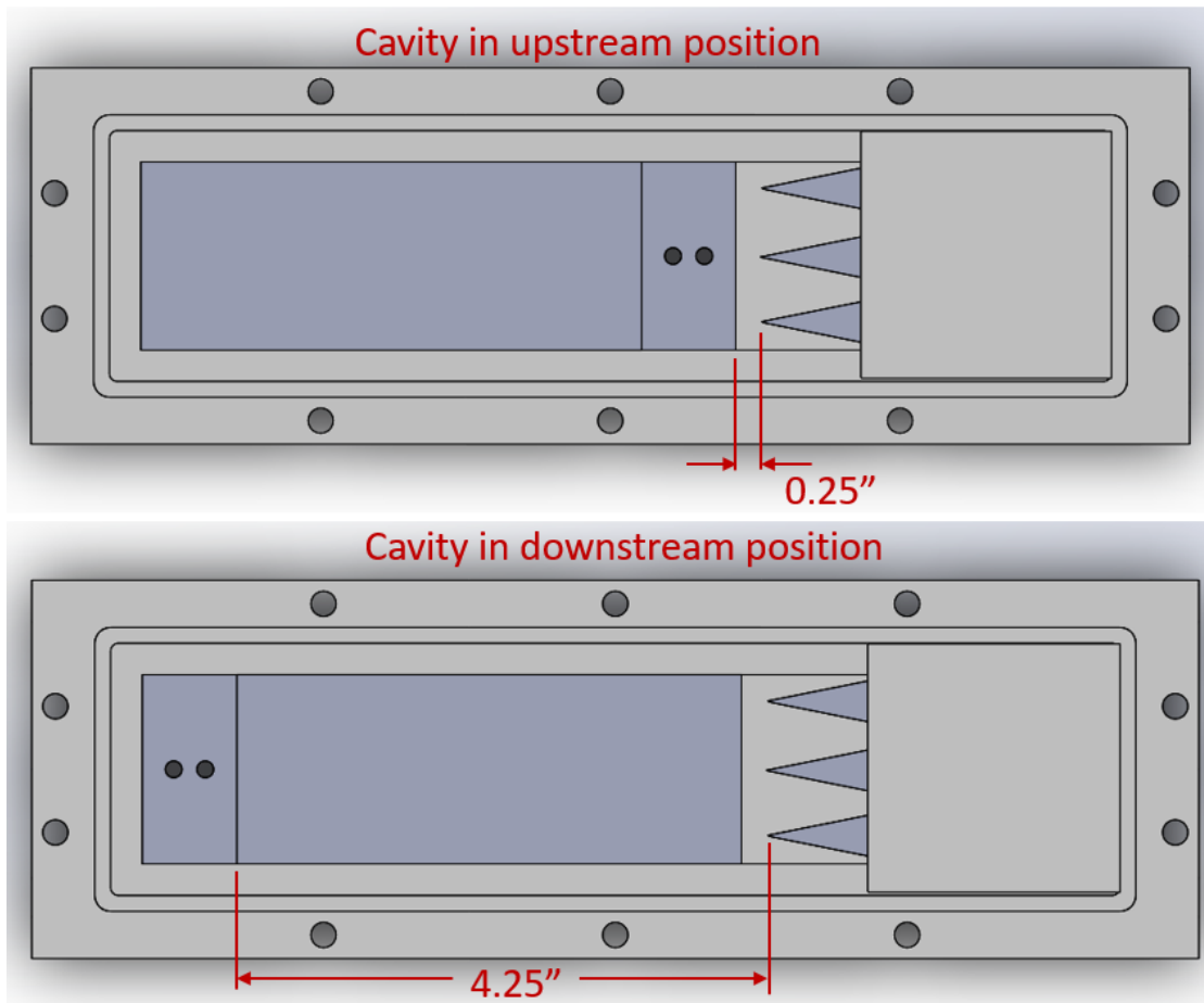
Figure 63. Test section cavity insert in the upstream and downstream positions. Upper – cavity placed in the upstream position. Lower – cavity placed in the downstream position. Flow is from right to left.
