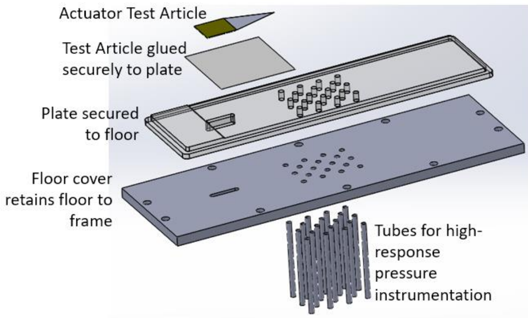
Figure 21. Exploded view of test section floor assembly.
