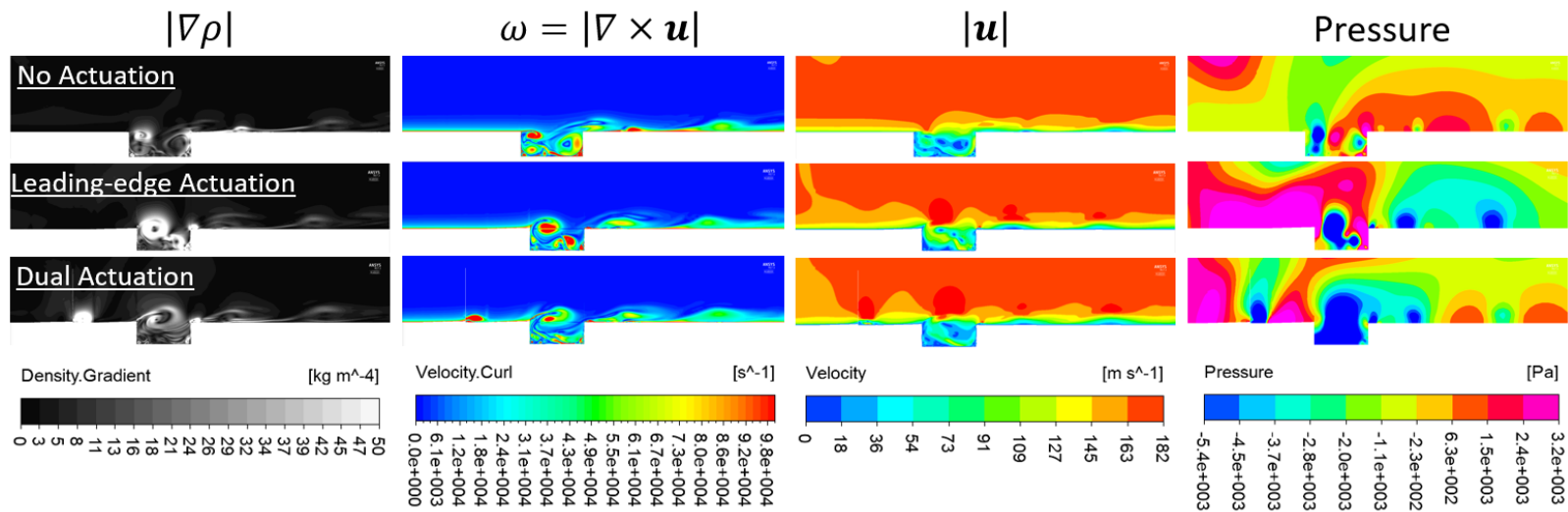
Figure 58. Comparison of cavity flow fields with and without actuation using various flow field parameters.
