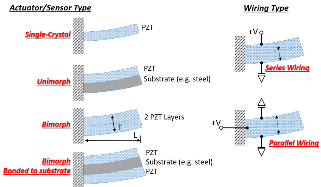
Figure 1. Example piezoelectric actuator/sensor types.
