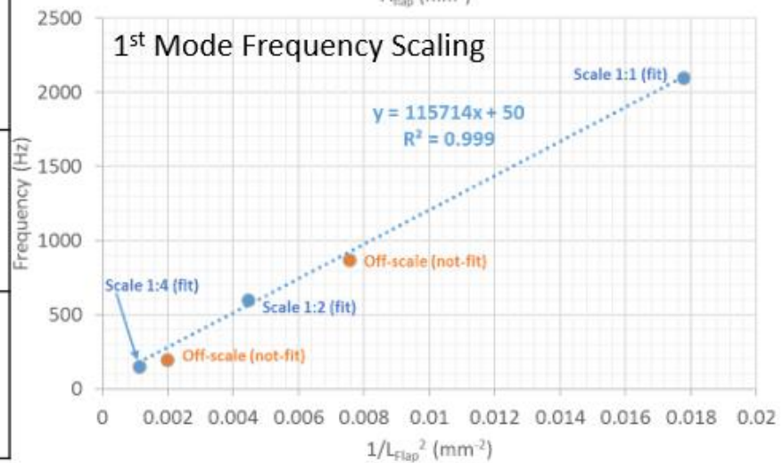
Figure 18. Numerical model for actuator scaling.
