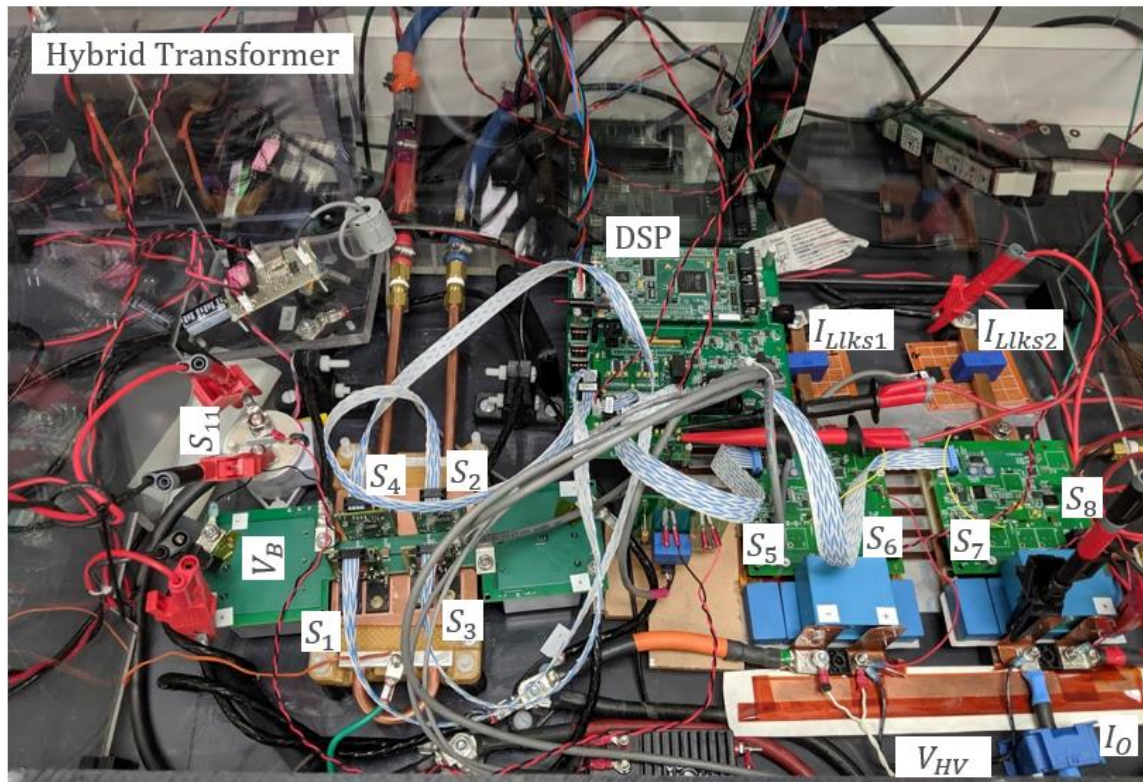
Figure 7.5. Integrated converter with controller and sensors.
