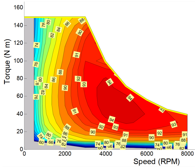
Figure 6.5. Combined motor inverter efficiency contours of 2010 Toyota Prius at 500 V [13].
