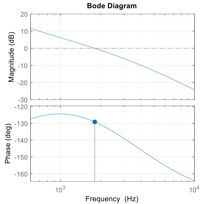
Figure 7.18. Open-loop response of the integrated converter in DAB mode.
