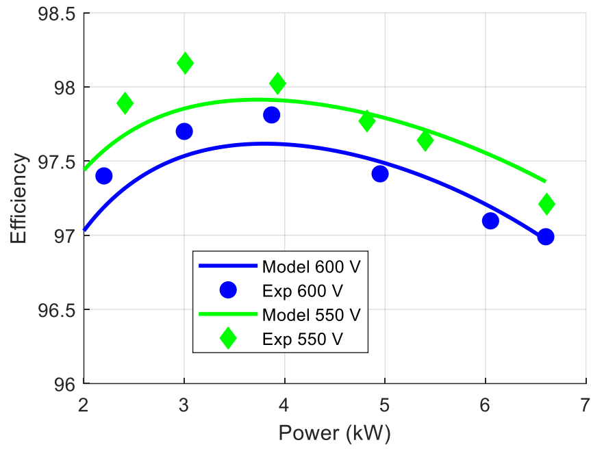
Figure 7.8. Efficiency sweep of the integrated converter in DAB mode.
