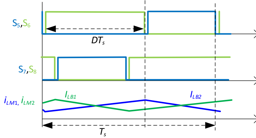
Figure 3.7. Interleaved boost converter in traction mode.
