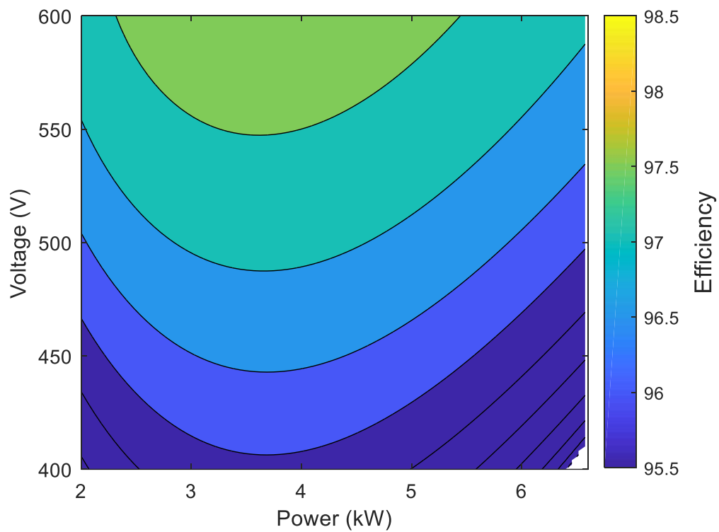
Figure 6.19. Integrated converter efficiency contour in DAB mode.
