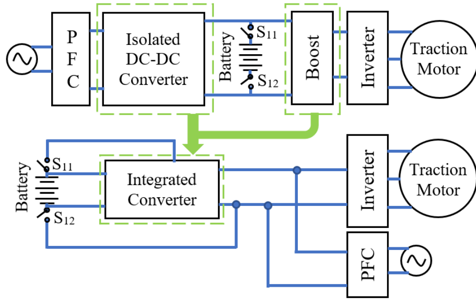
Figure 3.2. Integrated powertrain-charger DC-DC converter architecture.
