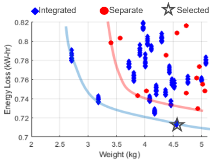
Figure 6.14. Pareto front for traction energy loss versus weight for integrated and separate boost-DAB solutions.
