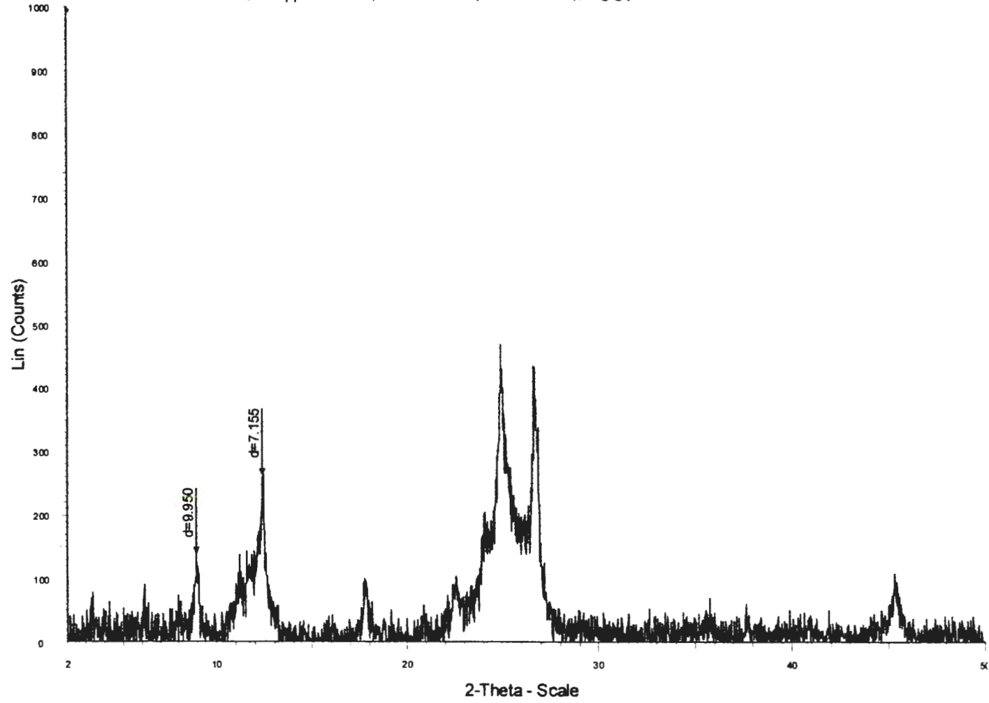
Mississippi Site One, 2Bt1 horizon (203 - 270 cm), Mg glycolated treatment
