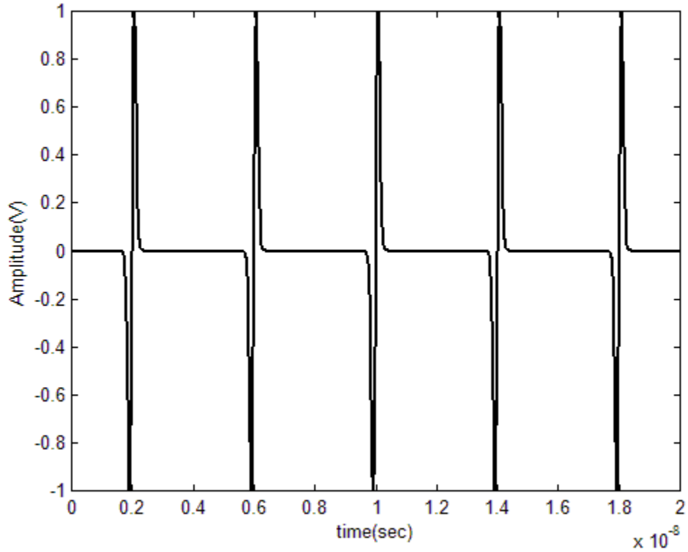
Figure 3.3: Gaussian first derivative pulse train of 5 monopulses.
