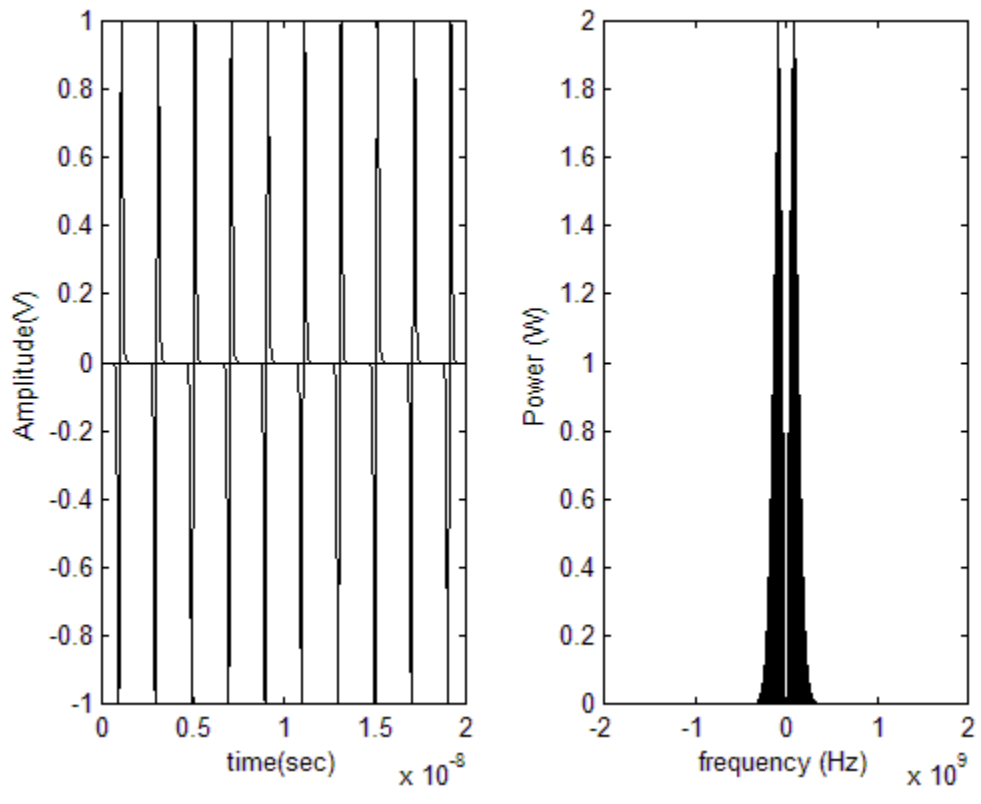
Figure 4.10: PSD of pulse train ( N_s=10 ).
