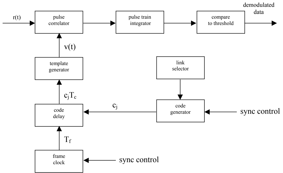
Figure 3.8: Block diagram of the UWB-IR receiver.
