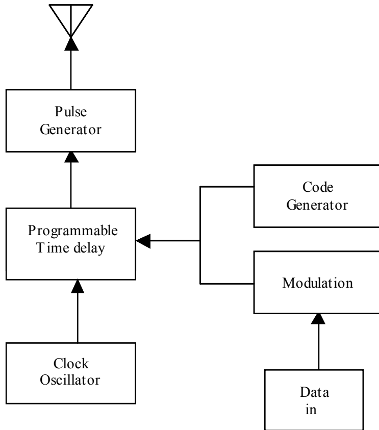
Figure 3.5: Block diagram of the UWB-IR transmitter.
