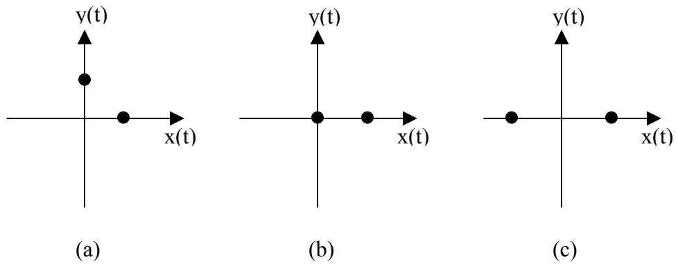
Figure 4.6: Constellation diagrams of (a) PPM (b) OOK (c) BPSK modulation schemes.
