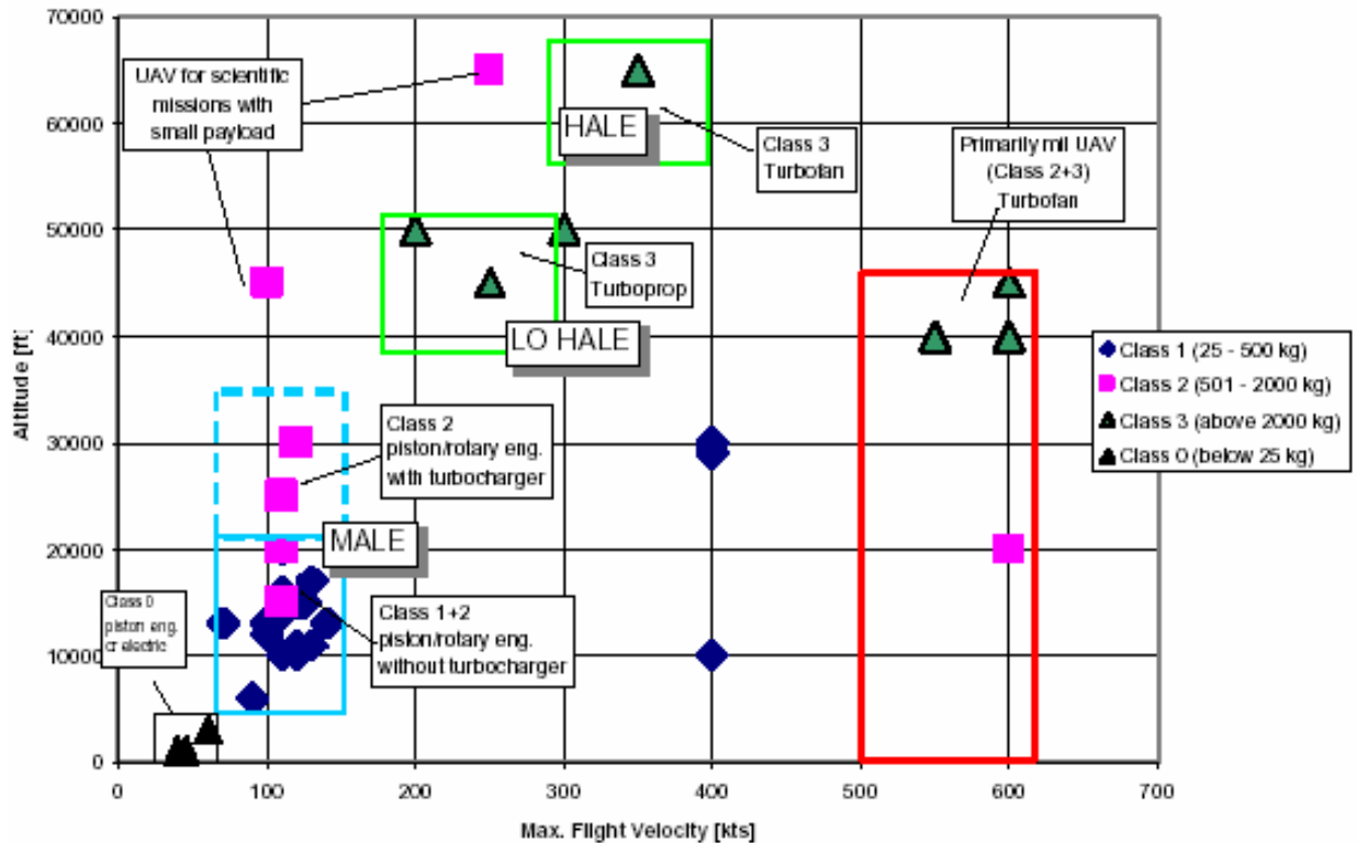
Figure 5: UAV Categorization by Flight Envelope Location (Source: Eurocontrol IABG Report, 2001)
