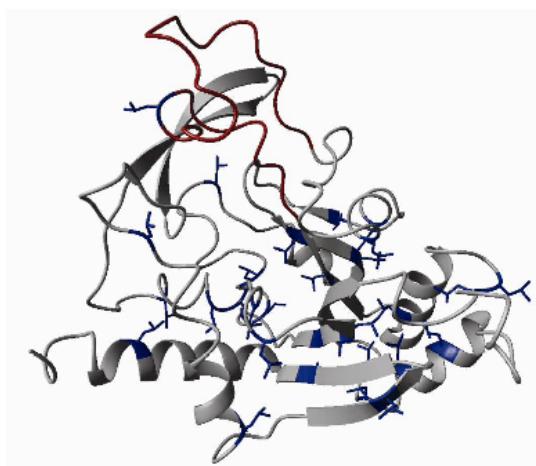
Figure 2: Homology-derived structure of AAC-IIIb
