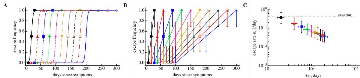
Figure 4. Time interval between measurements has a strong bias on the estimate of the escape rate and leads to a correlation between the escape rate ( \epsilon ) and time of escape ( t_{50} ). We generated artificial data in which viral sequences were measured in three time points, resulting in 0%, 50%, and 100% of the escape variant with N = 10 sequences per time point (panel A). In all cases, escape can be described by the logistic equation (Equation (1)) assuming a delayed immune response and escape rate \epsilon = 0.4 /day. We resampled these simulated “data” using a beta distribution (panel B, different lines indicate different escapes as in panel A) and estimated the average escape rate (panel C). We show the prediction of the logistic curve obtained using \epsilon = 0.4 /day (panel A), sampled data (panel B), and estimates of the escape rate obtained using parametric bootstrap (panel C). The horizontal dashed line in (panel C) denotes the theoretical escape rate of 0.4/day. The 95% confidence intervals in (panel B) are predicted using Jeffrey’s intervals [33], and in (panel C) CIs were calculated from bootstrapped samples.
