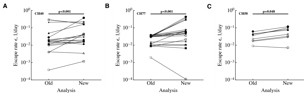
Figure 3. A sampling method provides higher estimates of the escape rates. We plot estimates of HIV escape rates in three patients (panel A: CH40, panel B: CH77, panel C: CH58) as was found in a previous study [25] employing data modifications (“Old” analysis) and estimates found using sampling method (“New” analysis). Different markers on plots indicate escape rate estimates for different escapes in our previous analysis [25]. Comparison of the escape rates in two analyses was done using Wilcoxon signed rank test and p values from these tests are indicated on individual panels.
