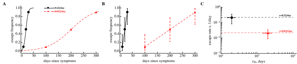
Figure 1. A sampling method accurately recovers virus escape rate for data when both wild-type and escape variant are detected at multiple sequential time points. We simulated viral escape using a logistic equation with two escape rates: \epsilon = 0.22/\text{day} (bullets) and \epsilon = 0.022/\text{day} (triangles). Three data points at which the escape variant was present at 10%, 50%, and 90% out of N = 10 sequences were generated (panel A). These simulated data were fitted by the simple logistic model (Equation (1)) using a likelihood approach, leading to expected escape rates (lines in panel A). These data were then resampled using the beta distribution (panel B, black solid line is for \epsilon = 0.22/\text{day} and red dashed line is for \epsilon = 0.022/\text{day} ) and fitted by the same model using the likelihood method. Resulting averages and their 95% confidence intervals match well with the numbers estimated using actual data (panel C). Dashed lines in panel (C) show estimates of the escape rates found in panel (A), and 95% confidence intervals in panel (B) are predicted using Jeffrey's intervals [33].
