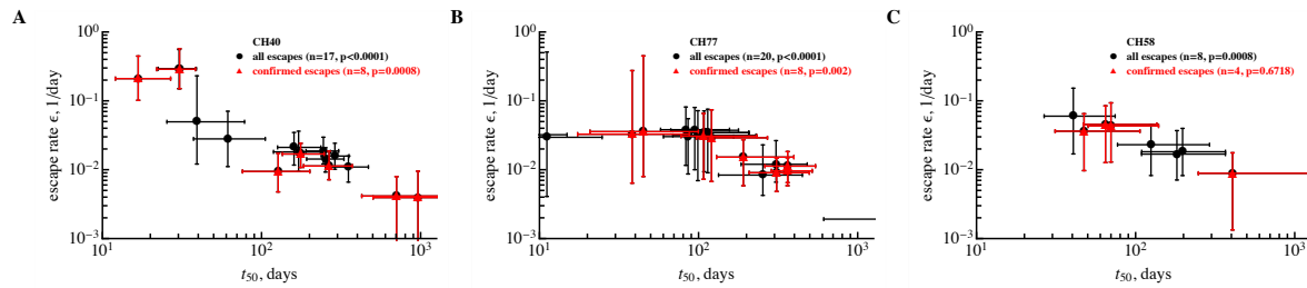
Figure 2. A sampling method which does not involve data modification still predicts a decline in the estimated escape rate with the time since infection. We used a novel approach of data sampling and estimated the rate of human immunodeficiency virus (HIV) escape from CD8 T cell responses for three Center for HIV/AIDS Vaccine Immunology (CHAVI) patients using previously published data [16,25]. Rates ( \epsilon ) and time to 50% of the escape variant ( t_{50} ) and associated errors are shown for three different patients in different panels (panel A: CH40, panel B: CH77, panel C: CH58); bullets indicate all escapes (in black) and triangles are for confirmed escapes (in red) [16]. Confirmed escapes were defined as fixed changes in HIV genome with a clear signature of viral escape with detected epitope-specific T cell response. Other escapes had a well-defined signature of escape but no epitope-specific T cell response was detected [16]. Resulting p values from the Spearman rank correlation test are indicated on individual panels. Panel (B) does not show an estimate for one escape due to very low escape rate \epsilon and long t_{50} .
