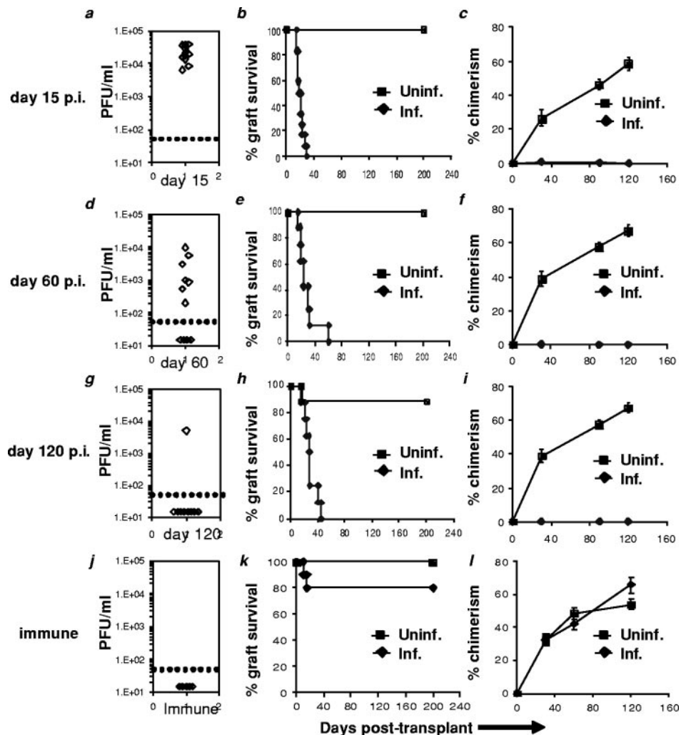
FIGURE 1. Chronic infection with LCMV clone 13 prevents tolerance induction and chimerism over a long time course. B6 mice were infected with 2 \times 10^6 PFU of LCMV clone 13. At 15 (a–c), 60 (d–f), or 120 (g–i) days postinfection, mice were treated with the tolerance induction regimen and given a BALB/c skin graft. j–l, LCMV immune mice also received the tolerance regimen 30 days after an acute infection with LCMV Armstrong. a, d, g, Mice were bled on days 15, 60, or 120 postinfection, respectively, and tested for the presence of LCMV in the serum. The dotted line represents the limit of detection. Mice transplanted at these time points were assessed for skin graft survival (b, e, and h) and donor cell chimerism (c, f, and i) over a long time course (at day 15, n = 15 for infected, n = 10 for uninfected; at days 60 and 120, n = 9 for infected, n = 8 for uninfected). Similar assays were performed for LCMV-immune mice. j, Serum titers were measured 30 days after acute infection with LCMV Armstrong ( n = 5 ). Mice received the tolerance regimen and a BALB/c skin allograft >30 days postinfection and were assessed for skin graft survival (k) and chimerism (l) ( n = 10 for infected, n = 8 for uninfected). All error bars represent the SEM ( p < 0.001 for all infected vs uninfected groups). Skin graft survival and chimerism data are pooled from two separate experiments.
