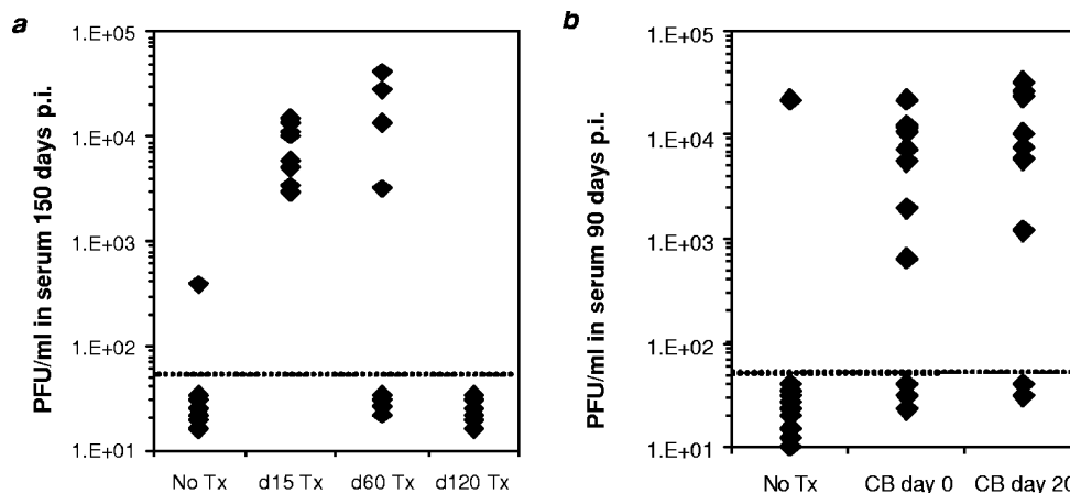
FIGURE 3. Costimulation blockade-based therapies prevent control of ongoing chronic infection. a, B6 mice were infected with LCMV clone 13 and received either no further treatment (No Tx; n = 7 ) or the tolerance regimen on days 15 (d15 Tx; n = 8 , p < 0.01 vs No Tx), 60 (d60 Tx; n = 8 , p < 0.05 vs No Tx), or 120 (d120 Tx; n = 6 ) postinfection. Mice were bled at day 150 postinfection and serum was tested for the presence of LCMV. The y-axis displays plaque forming units per milliliter. The dotted line indicates the limit of detection for this assay. b, B6 mice were treated with LCMV and received either no further treatment (No Tx; n = 10 ) or administration of CTLA4-Ig and anti-CD40L starting on day 0 (CB day 0; n = 10 , p < 0.05 vs No Tx) or day 20 (CB day 20; n = 10 , p < 0.05 vs No Tx) postinfection. Mice were bled on day 90 postinfection and serum was tested for the presence of LCMV. The y-axis displays plaque forming units per milliliter in the serum. The dotted line indicates the limit of detection for this assay. Results are pooled from two separate experiments.
