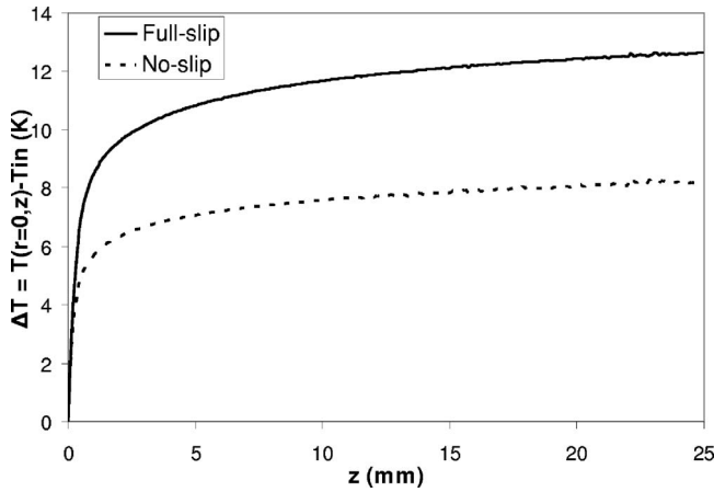
FIG. 7. Effect of the applied boundary conditions on the calculated axial temperature profiles for the HDPE melt at T_{in}=190\text{ }^{\circ}\text{C} and \dot{\epsilon}=34\text{ s}^{-1} .
