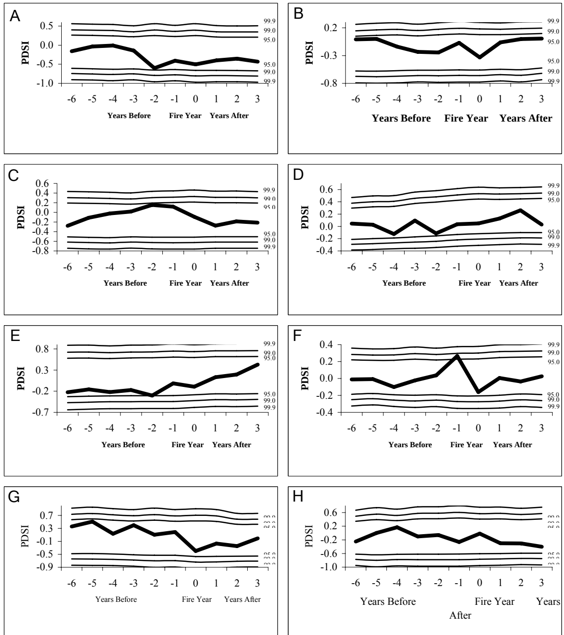
Figure 5.6: Relationships between the Virginia reconstructed PDSI and minor fires (10%-scarred) for Brush Mountain early period (1750–1860) (A) and late period (1861–1934) (B); Griffith Knob early period (1764–1893) (C) and late period (1894–1934) (D); Little Walker Mountain early period (1778–1859) (E) and late period (1860–1934) (F); and, North Mountain early period (1742–1857) (G) and late period (1858–1934) (H).
