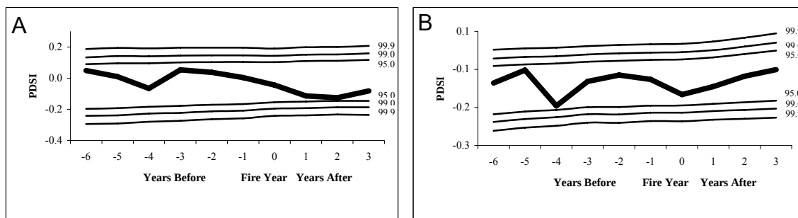
Figure 5.12: Relationships between the Virginia reconstructed PDSI and early period (1732–1850) (A) of all fires and late period (1851–1934) (B) of all fires at all sites.
