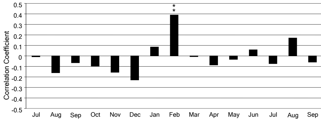
Figure 3.11: Results of correlation analysis of composite chronology: NAO correlated against Table Mountain pine tree growth. Statistically significant relationships are indicated by ** ( p < 0.01 ).
