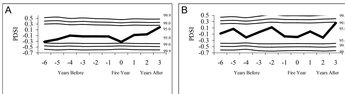
Figure 5.14: Relationship between the Virginia reconstructed PDSI and major fire events at all sites 25%-scarred early period (1732–1850) (A) and major fire events at all sites 25%-scarred late period (1851–1934) (B).
