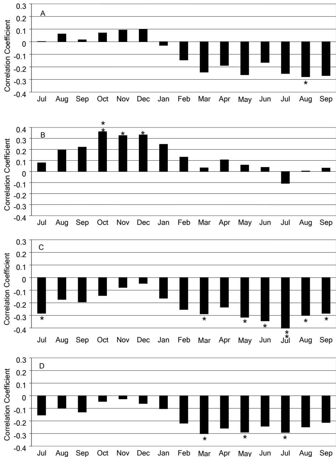
Figure 3.7: Results of correlation analysis for North Mountain (A), Brush Mountain (B), Griffith Knob (C), and Little Walker Mountain (D): Kaplan indices correlated against Table Mountain pine tree growth. Statistically significant relationships are indicated by * ( p < 0.05 ) and ** ( p < 0.01 ).
