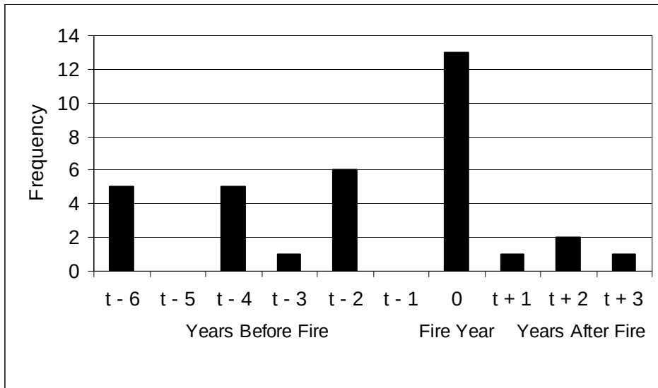
Figure 5.15: Composite results for all superposed epoch analyses conducted in this chapter (all epochs and all fire event classes) using Virginia Table Mountain pine PDSI reconstructions. Only the number of years showing relationships with negative PDSI values (drought years) are shown. Statistically significant and near significant i.e., ecologically meaningful) results are shown.
