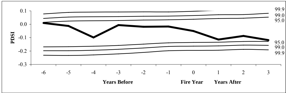
Figure 5.10: Relationships between Virginia reconstructed PDSI and minor fire (10%-scarred) years at all sites.
