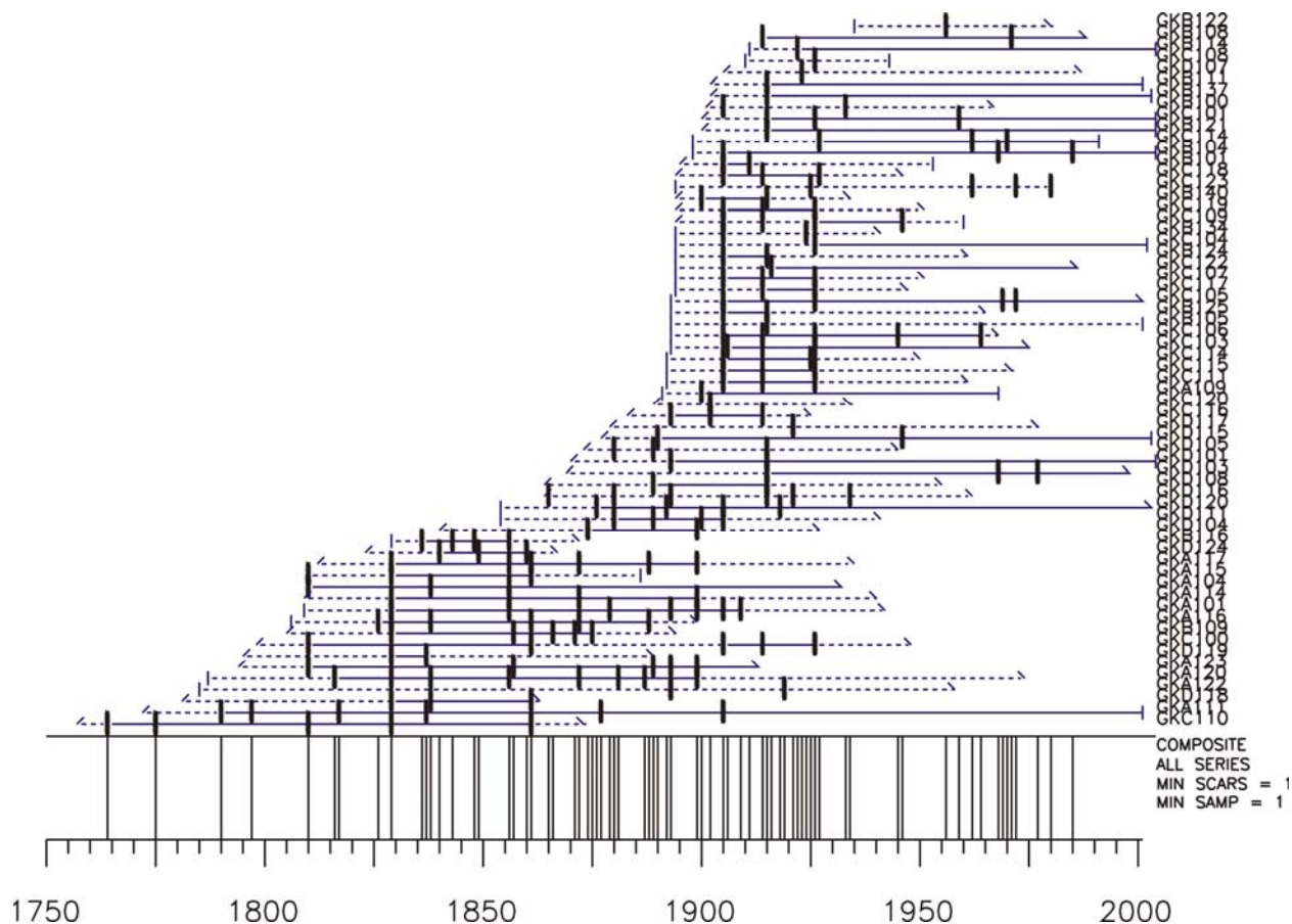
Figure 4.3: Griffith Knob composite fire history chronology. The spatial distribution of fire events is illustrated by the sample identifications on the right while the temporal distribution of fire events is illustrated by the composite axis at the bottom of the chart. Horizontal lines (dashed = non-recorder years, solid = recorder years) represent the range of years for the sample listed at the right. Each vertical bar shown on the horizontal lines is a fire event.
