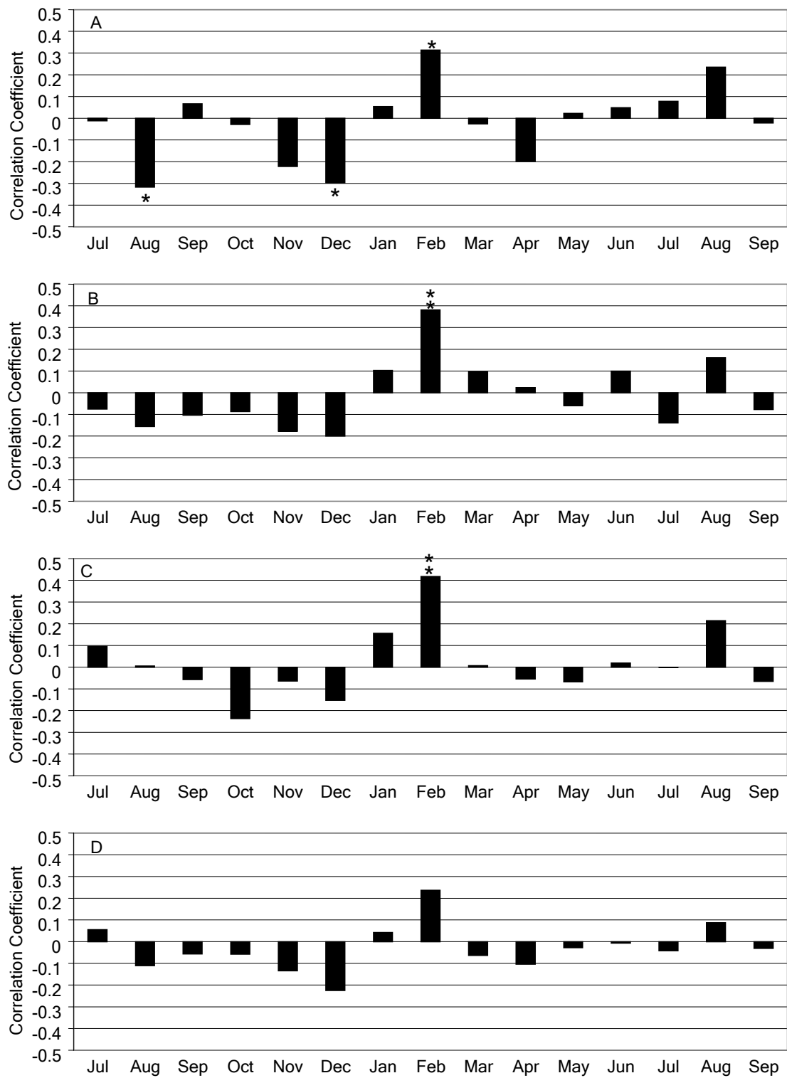
Figure 3.6: Results for correlation analysis of Brush Mountain (A), Griffith Knob (B), Little Walker Mountain (C), and North Mountain (D): NAO correlated against Table Mountain pine tree growth. Statistically significant relationships are indicated by * ( p < 0.05 ) and ** ( p < 0.01 ).
