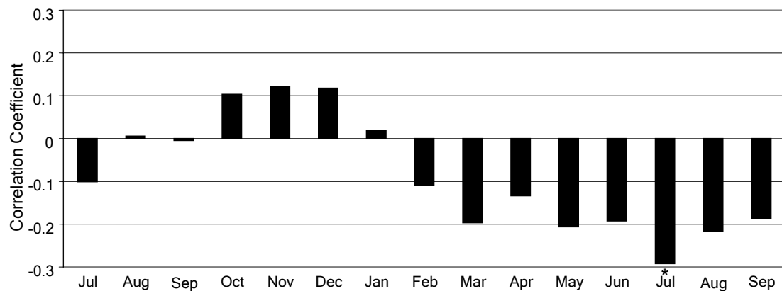
Figure 3.12: Results of correlation analysis for composite chronology: Kaplan indices correlated against Table Mountain pine tree growth. Statistically significant relationships are indicated by * ( p < 0.05 ).
