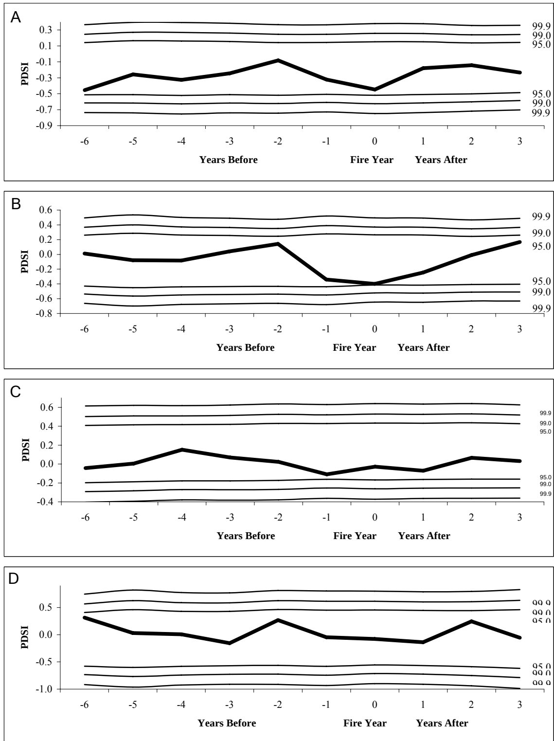
Figure 5.4: The relationship between the Virginia PDSI reconstruction and major fire events (25%-scarred) at Brush Mountain (A), Griffith Knob (B), Little Walker Mountain (C), and North Mountain (D).
