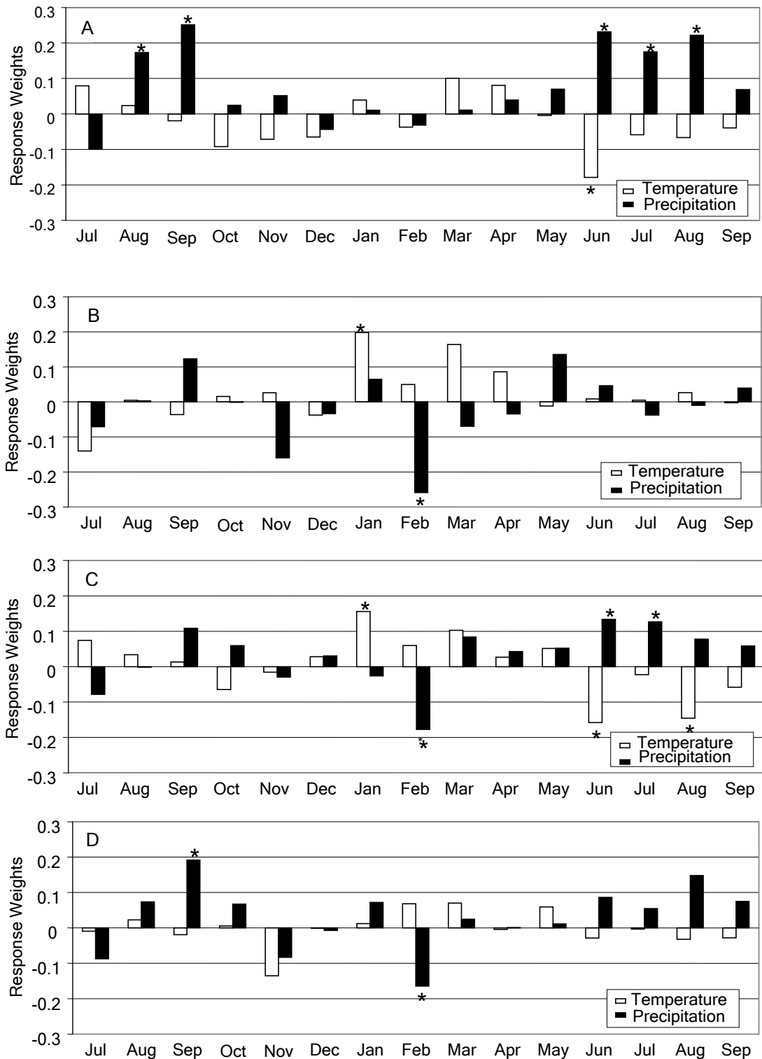
Figure 3.3: Results of response function analysis for North Mountain (A), Brush Mountain (B), Griffith Knob (C), and Little Walker Mountain (D) showing the effects of temperature and precipitation on Table Mountain pine tree growth. Statistically significant relationships are indicated by * ( p < 0.05 ).
