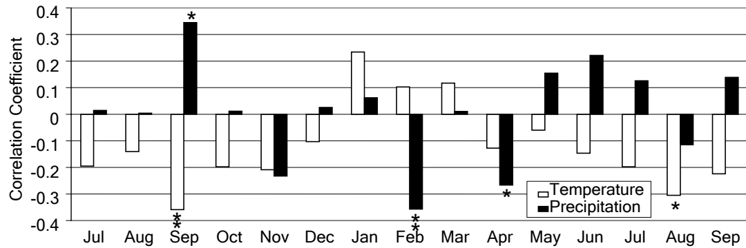
Figure 3.9: Results of correlation analysis for composite chronology, comparing precipitation and temperature Table Mountain pine tree growth. Statistically significant relationships are indicated by * ( p < 0.05 ) and ** ( p < 0.01 ).
