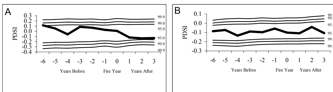
Figure 5.13: Relationships between the Virginia reconstructed PDSI and early period (1732–1850) of minor fires (10%-scarred) (A) and late period (1851–1934) of minor fires (10%-scarred) (B) at all sites.
