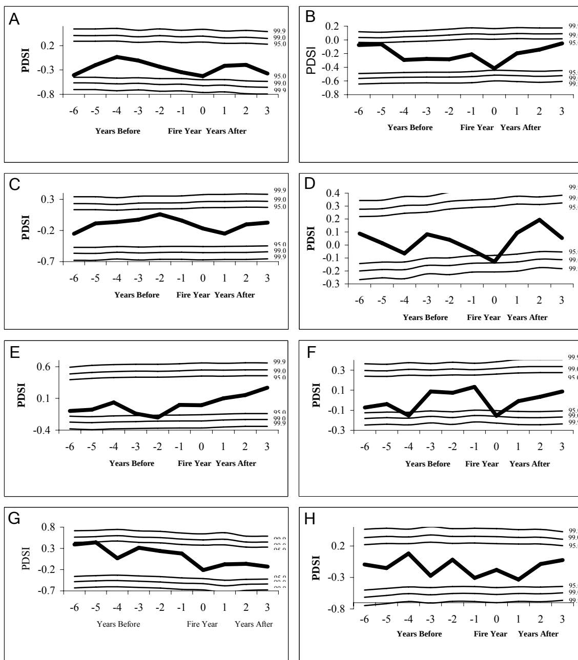
Figure 5.5: Relationships between the Virginia reconstructed PDSI and all fire events for Brush Mountain early period (1750–1860) (A) and late period (1861–1934) (B); Griffith Knob early period (1764–1893) (C) and late period (1894–1934) (D); Little Walker Mountain early period (1778–1859) (E) and late period (1860–1934) (F); and, North Mountain early period (1742–1857) (G) and late period (1858–1934) (H).
