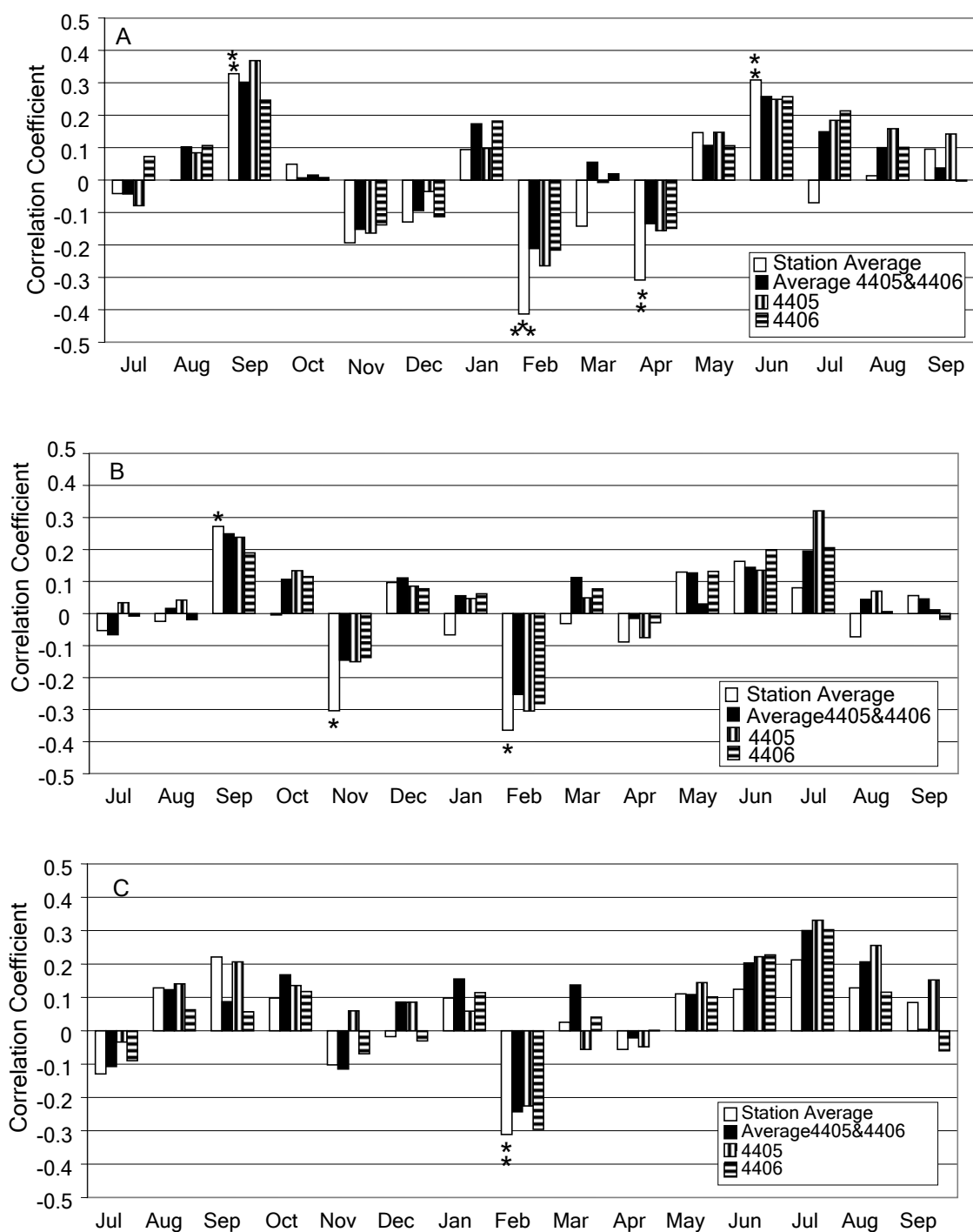
Figure 3.2: Results for the Brush Mountain (A), Griffith Knob (B), and Little Walker Mountain (C) correlation analysis, comparing precipitation for region 4405, region 4406, and the average of regions 4405 and 4406 with the tree-ring chronology. Statistically significant relationships are indicated by * ( p < 0.05 ), ** ( p < 0.01 ) and *** ( p < 0.001 ).
