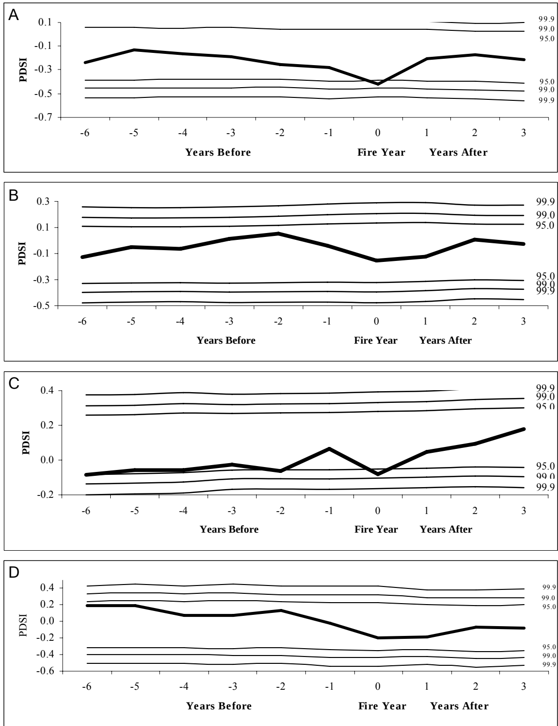
Figure 5.2: Relationships between Virginia reconstructed PDSI and all fire years from Brush Mountain (A), Griffith Knob (B), Little Walker Mountain (C), and North Mountain (D). Positive PDSI values indicate significantly wet periods and negative PDSI values indicate significantly dry periods.
