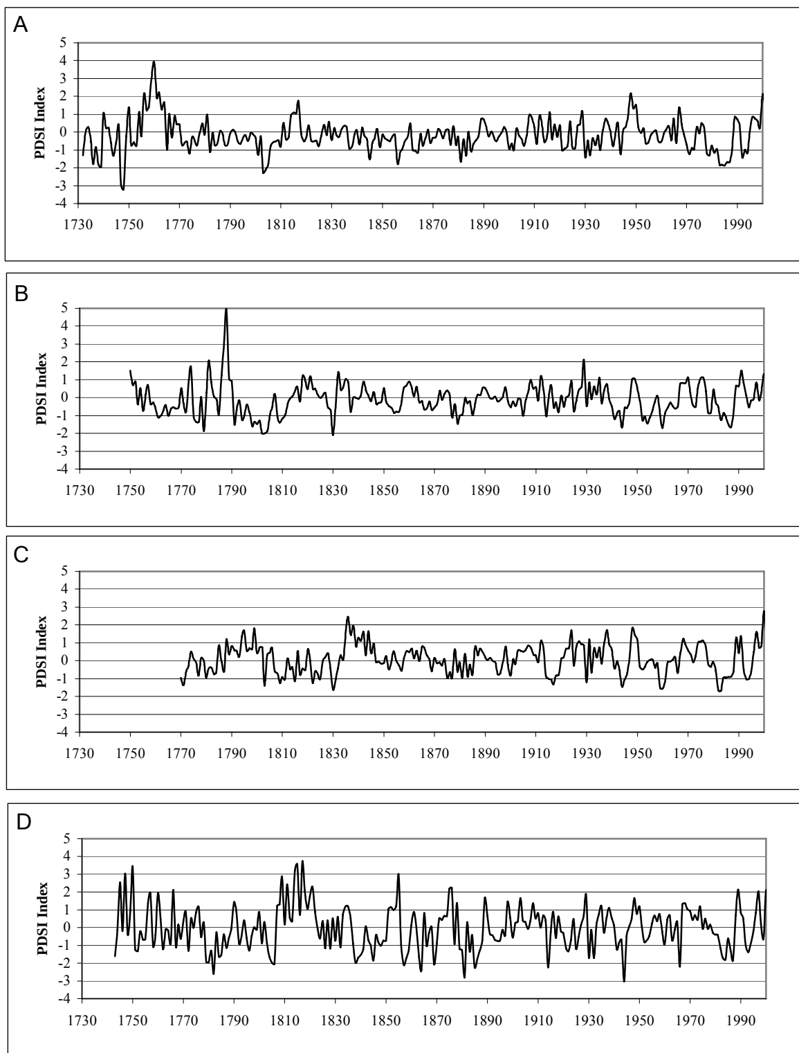
Figure 5.1: PDSI reconstructions based on Virginia Table Mountain pine chronologies for Brush Mountain (A), Griffith Knob (B), Little Walker Mountain (C), and North Mountain (D).
