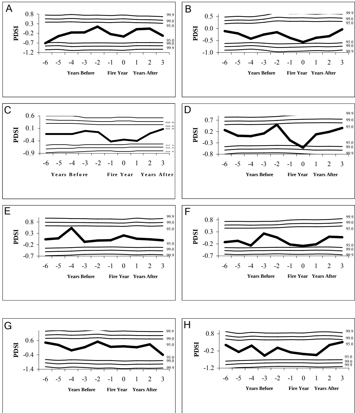
Figure 5.7: Relationship between the Virginia reconstructed PDSI and major fire events (25%-scarred) for Brush Mountain early period (1750–1860) (A) and late period (1861–1934) (B); Griffith Knob fire events early period (1764–1893) (C) and late period (1894–1934) (D); Little Walker Mountain fire events early period (1778–1859) (E) and late period (1860–1934) (F); North Mountain fire events early period (1742–1857) (G) and late period (1858–1934) (H).
