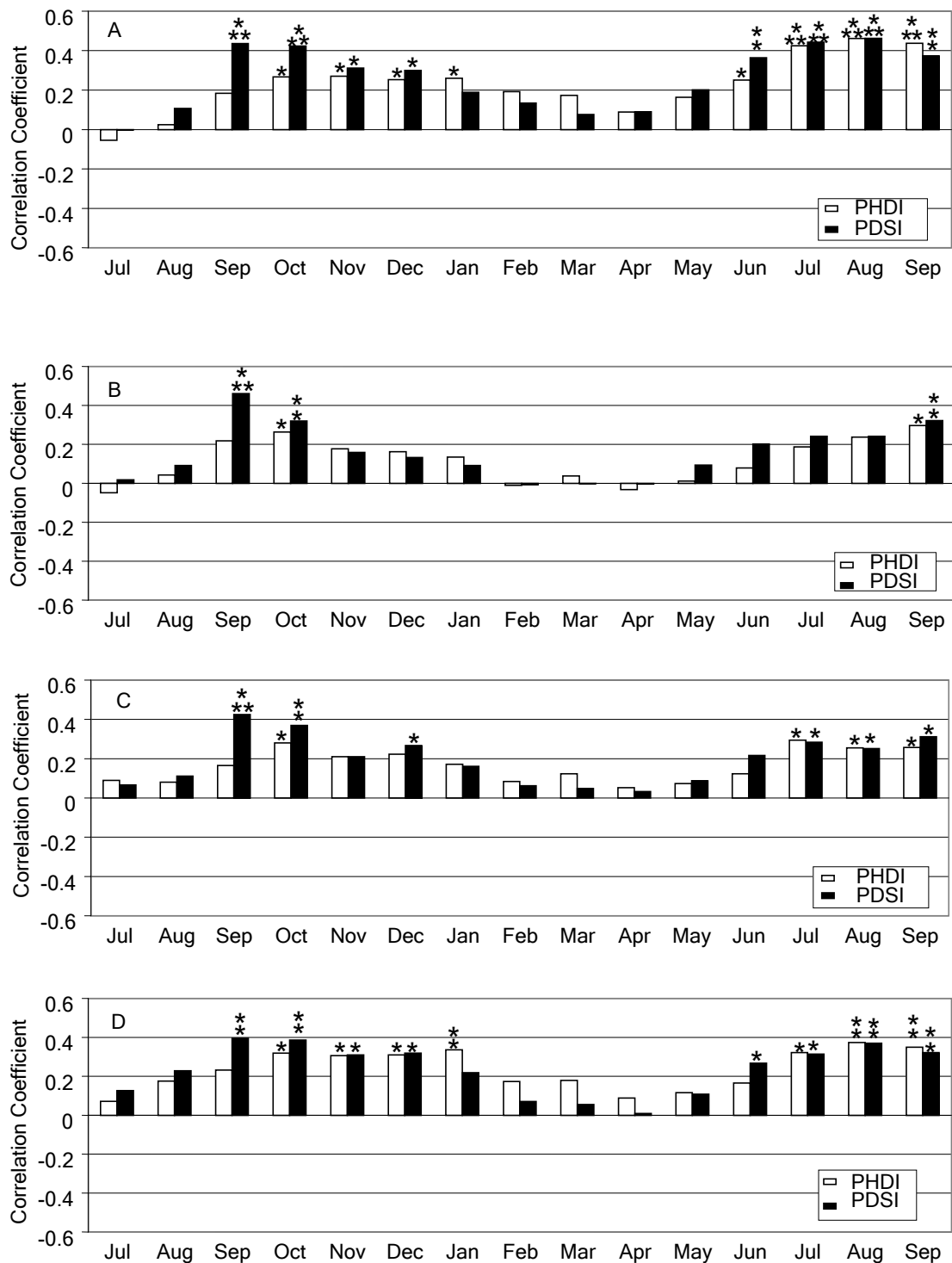
Figure 3.5: Results of correlation analysis for North Mountain (A), Brush Mountain (B), Griffith Knob (C), and Little Walker Mountain (D): PDSI and PHDI correlated against Table Mountain pine tree growth. Statistically significant relationships are indicated by * ( p < 0.05 ), ** ( p < 0.01 ), *** ( p < 0.001 ).
