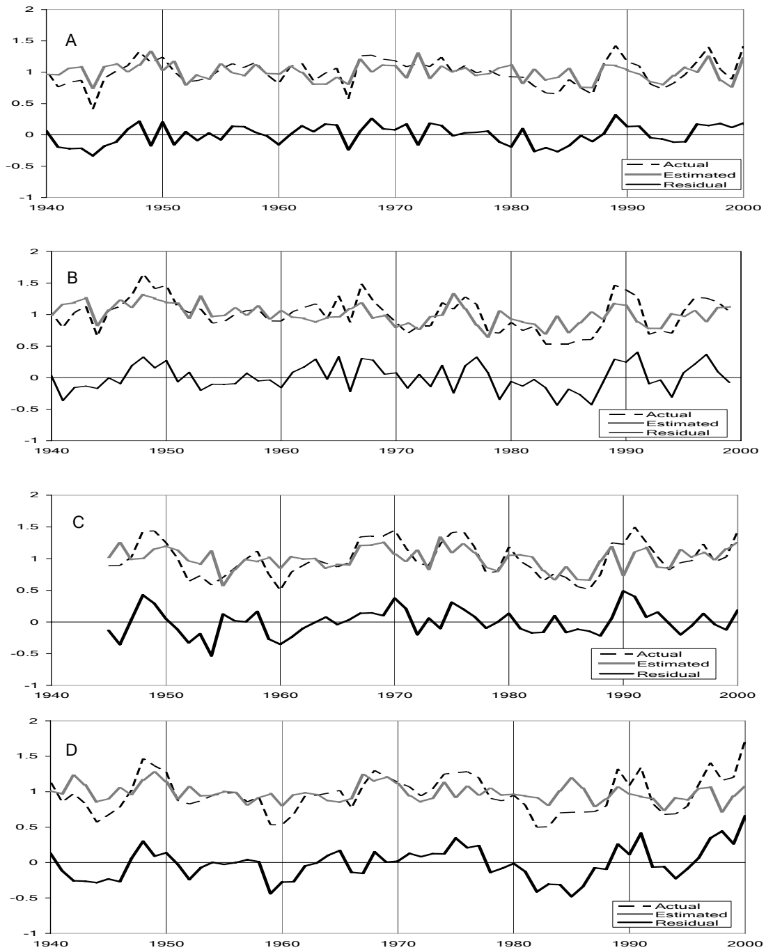
Figure 3.8: Results for North Mountain (A), Brush Mountain (B), Griffith Knob (C), and Little Walker Mountain (D) illustrating those periods in which tree growth was below that expected from the observed climate variables. “Actual” indicates the actual Table Mountain pine tree growth, “estimated” indicates the estimated annual Table Mountain pine tree growth based on the significant climate variables, and “residual” is the difference between the actual and estimated chronologies.
