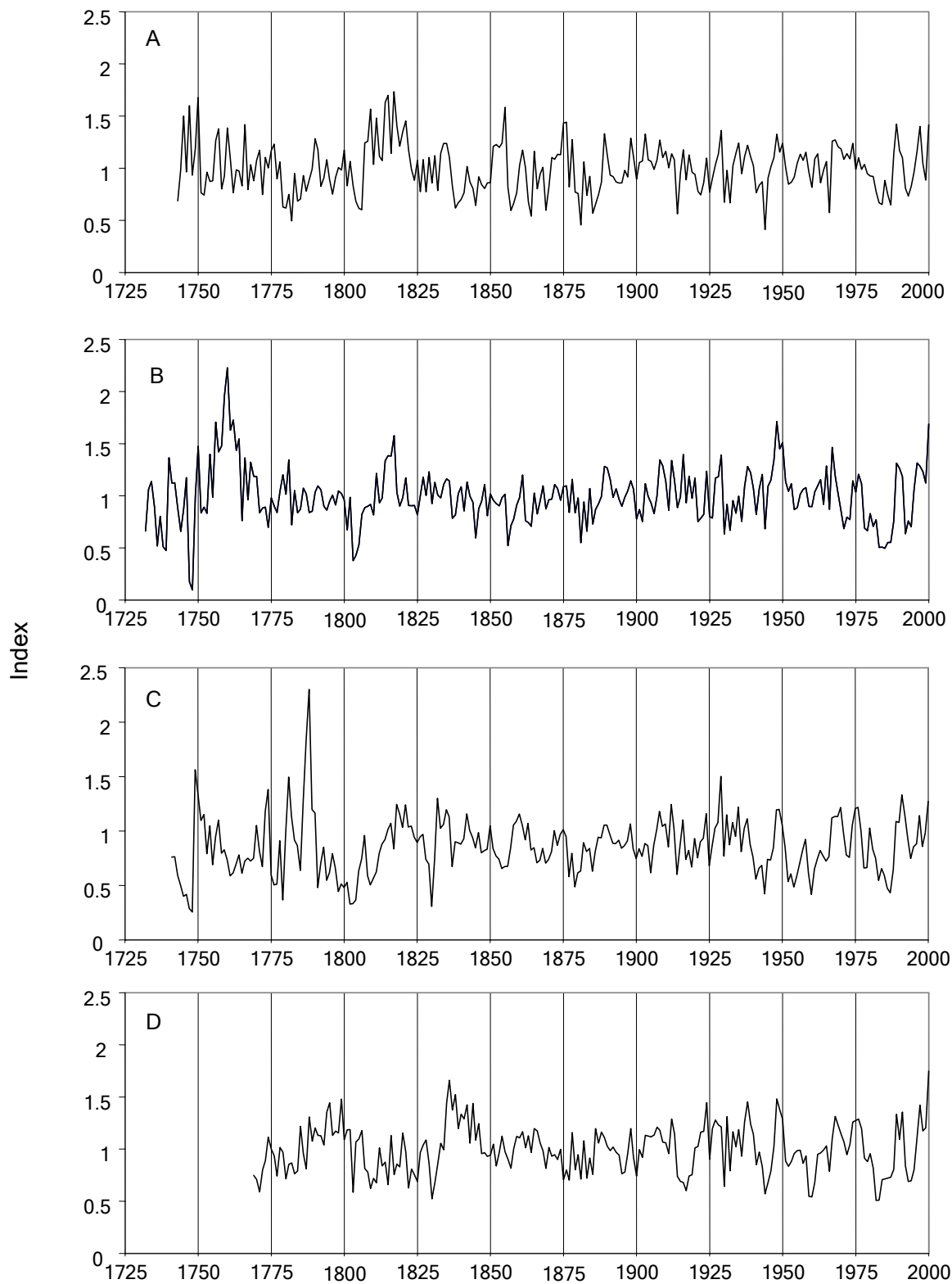
Figure 3.1: The North Mountain (A), Brush Mountain (B), Griffith Knob (C), and Little Walker Mountain (D) tree-ring index chronologies.
