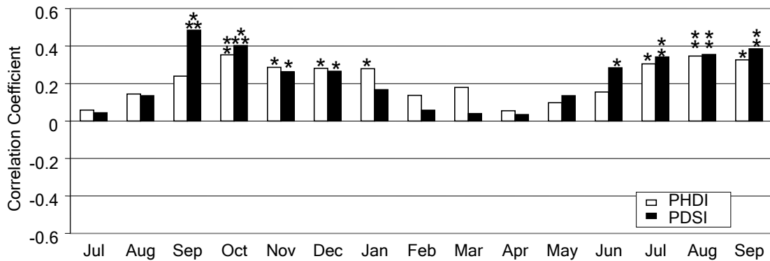
Figure 3.10: Results of correlation analysis for composite chronology: PDSI and PHDI correlated against Table Mountain pine tree growth. Statistically significant relationships are indicated by * ( p < 0.05 ), ** ( p < 0.01 ), and *** ( p < 0.001 ).
