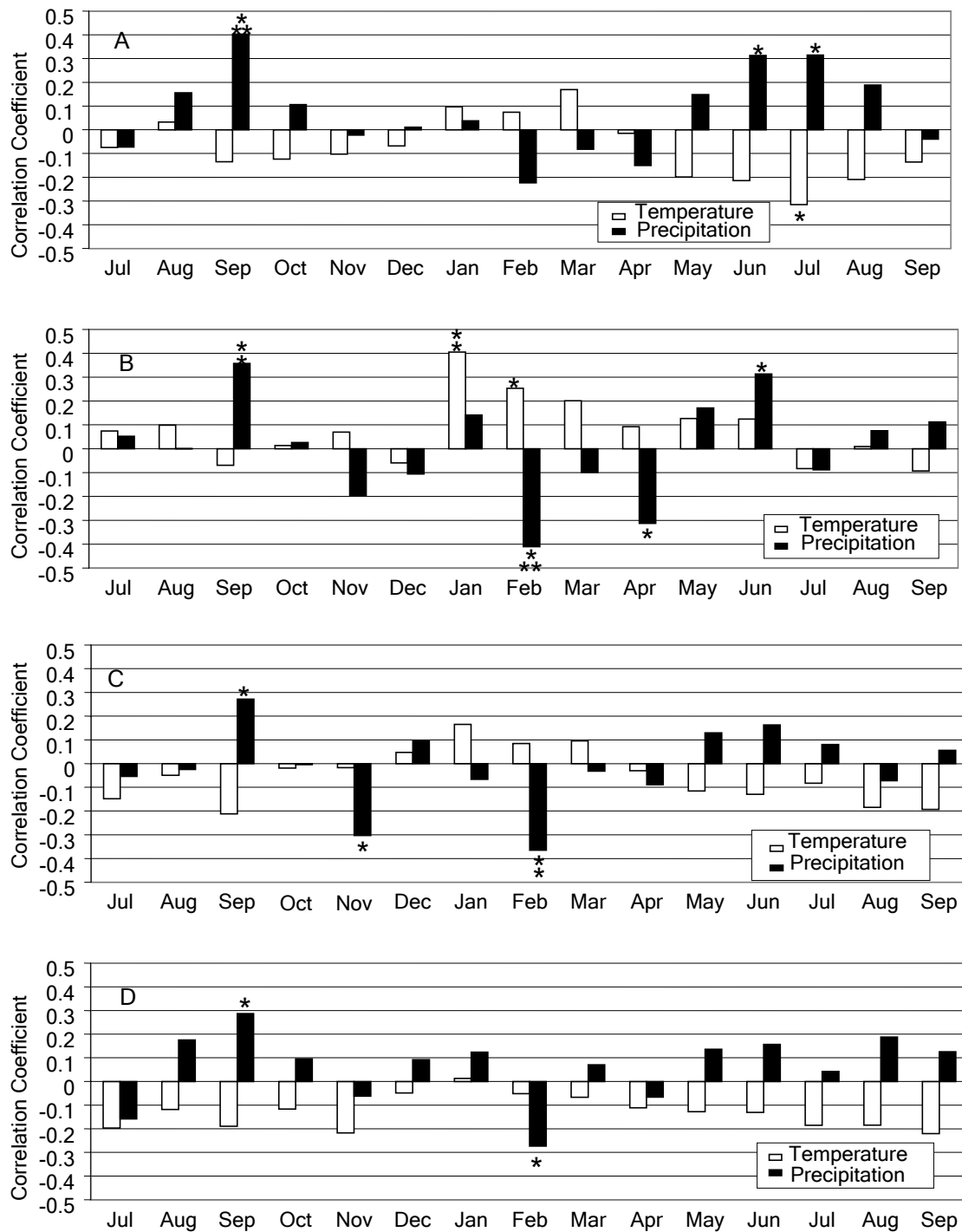
Figure 3.4: Results of correlation analysis for North Mountain (A), Brush Mountain (B), Griffith Knob (C), and Little Walker Mountain (D) comparing precipitation and temperature for the station average and Table Mountain pine tree growth. Statistically significant relationships are indicated by * ( p < 0.05 ), ** ( p < 0.01 ), and *** ( p < 0.001 ).
