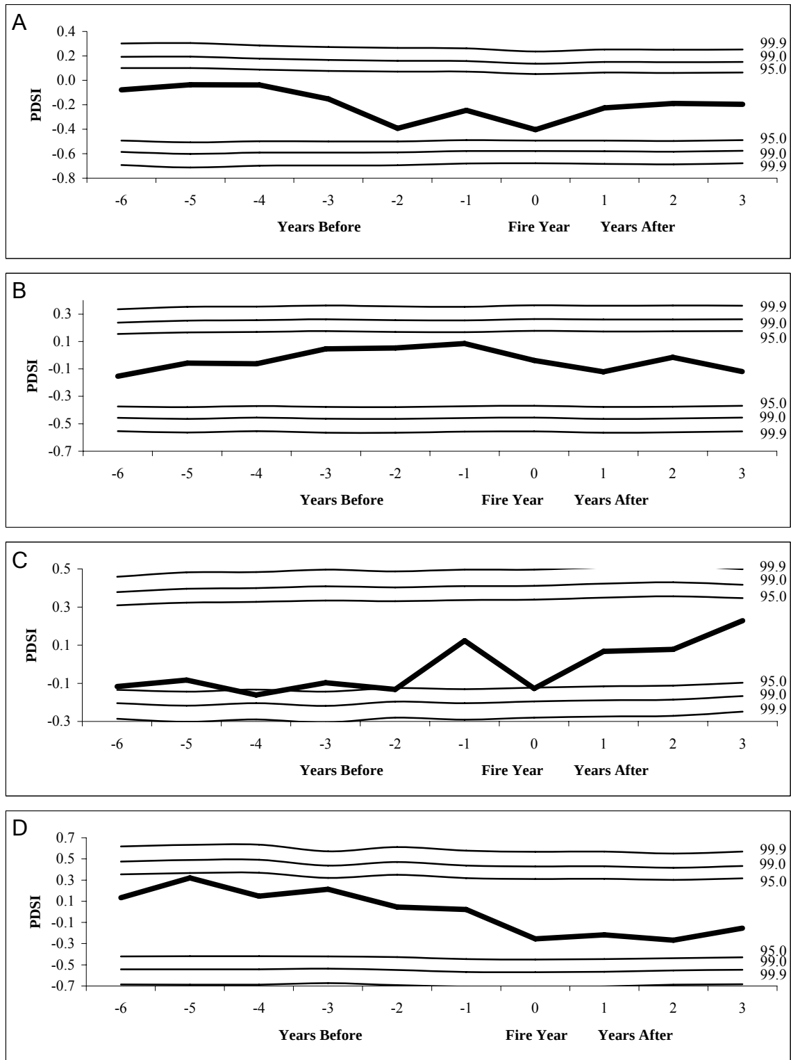
Figure 5.3: The relationship between the Virginia PDSI reconstruction and minor fire events (10%-scarred) at Brush Mountain (A), Griffith Knob (B), Little Walker Mountain (C), and North Mountain (D).
