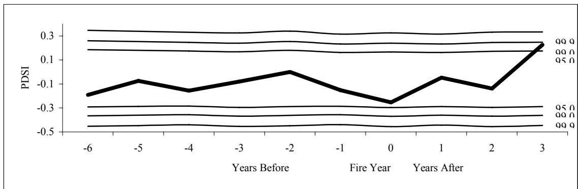
Figure 5.11: Relationships between Virginia reconstructed PDSI and major fire (25%-scarred) years at all sites.
