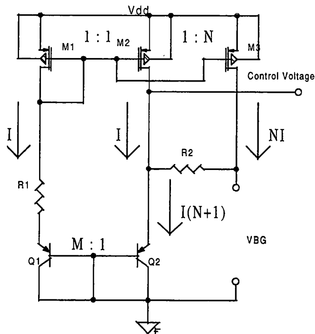
Figure 4.12 - CMOS Compatible Bandgap Reference
