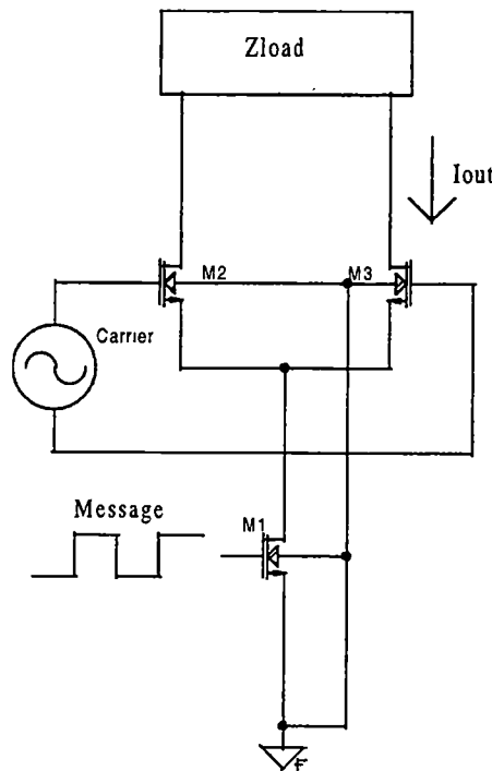
Figure 4.3 - Active CMOS Mixer
