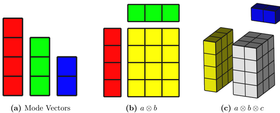
Figure 1.1: Tensor Product
