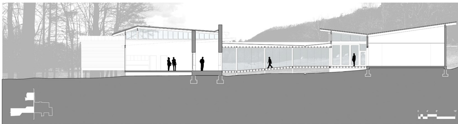
fig. a.07- Section 4 Source: Author
