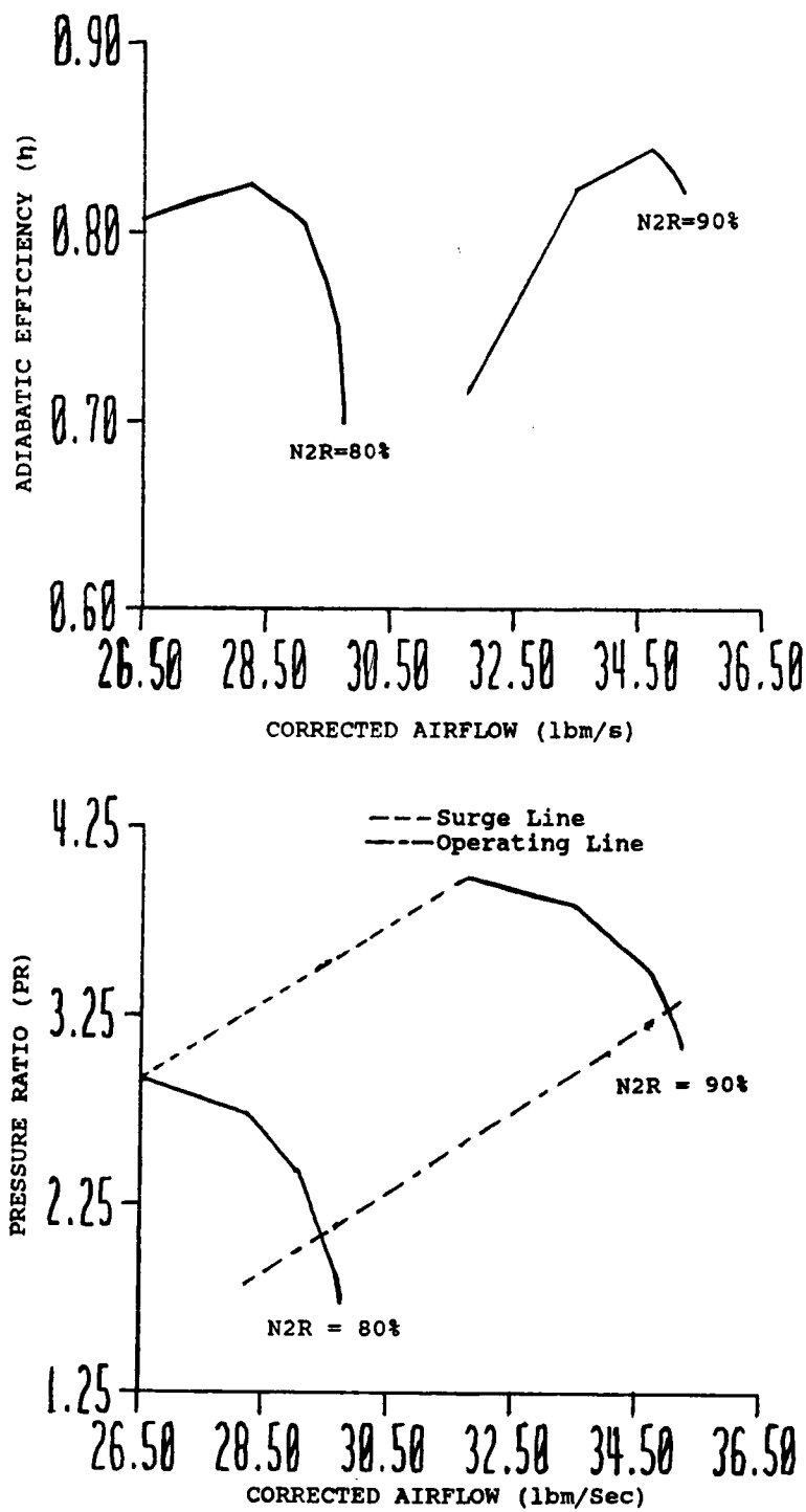
Figure 5. Allison XC-1 Lift Engine Compressor Map
