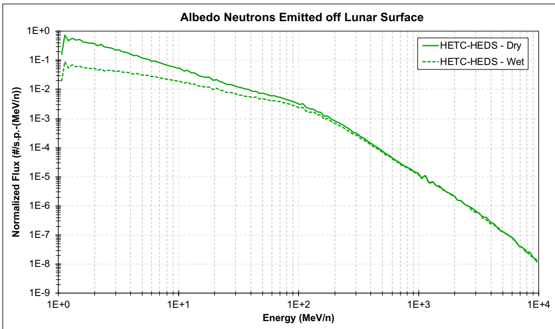
Figure 6.4. A comparison between the energy distribution of albedo neutrons emitted off a dry and a wet regolith generated using HETC-HEDS.
