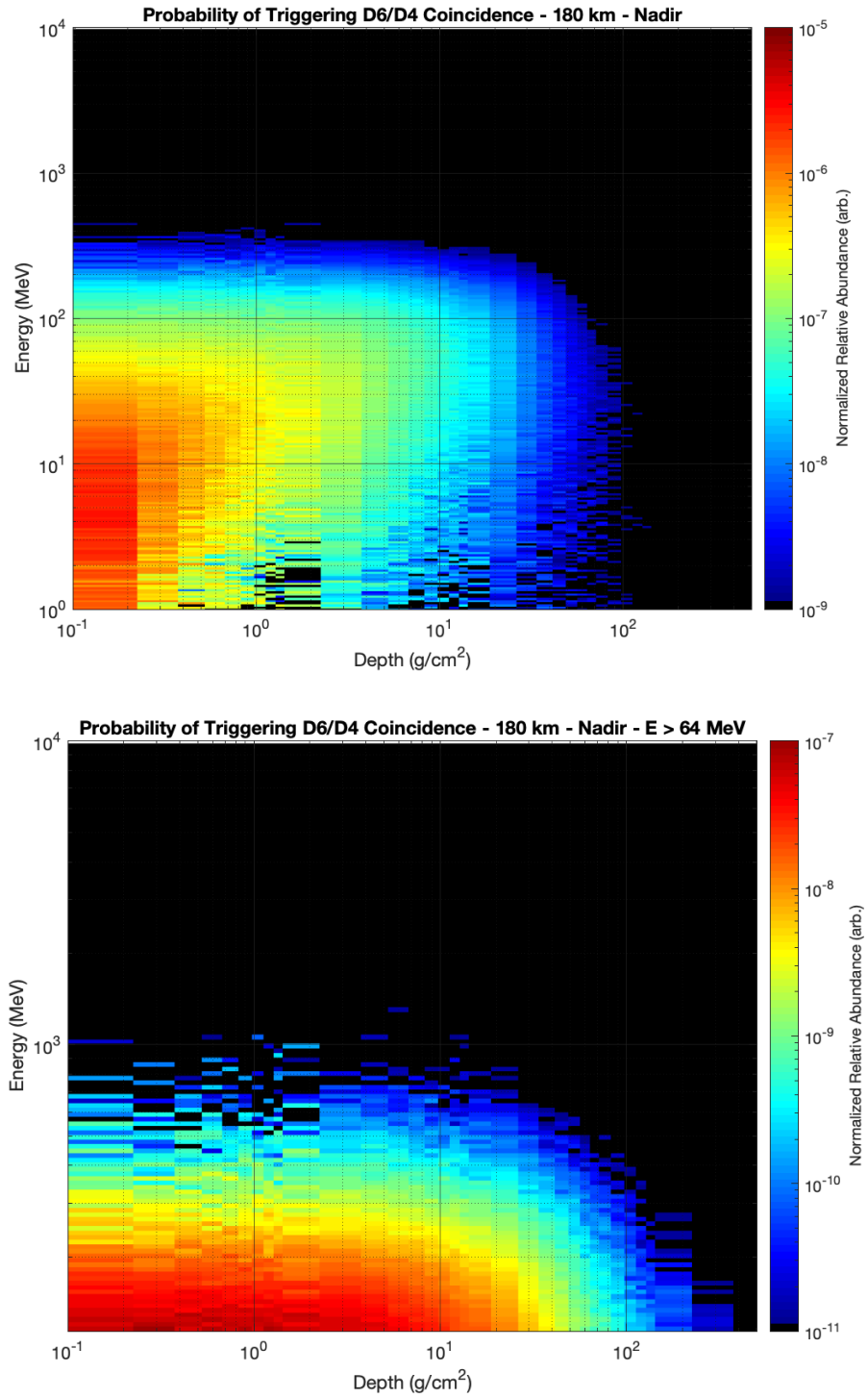
Figure 7.6. The maximum depth distribution of albedo protons triggering D6/D4 coincidence when facing the lunar nadir at altitude of 180 km for all modeled energies (top) and above the threshold energy of 64 MeV (bottom).
