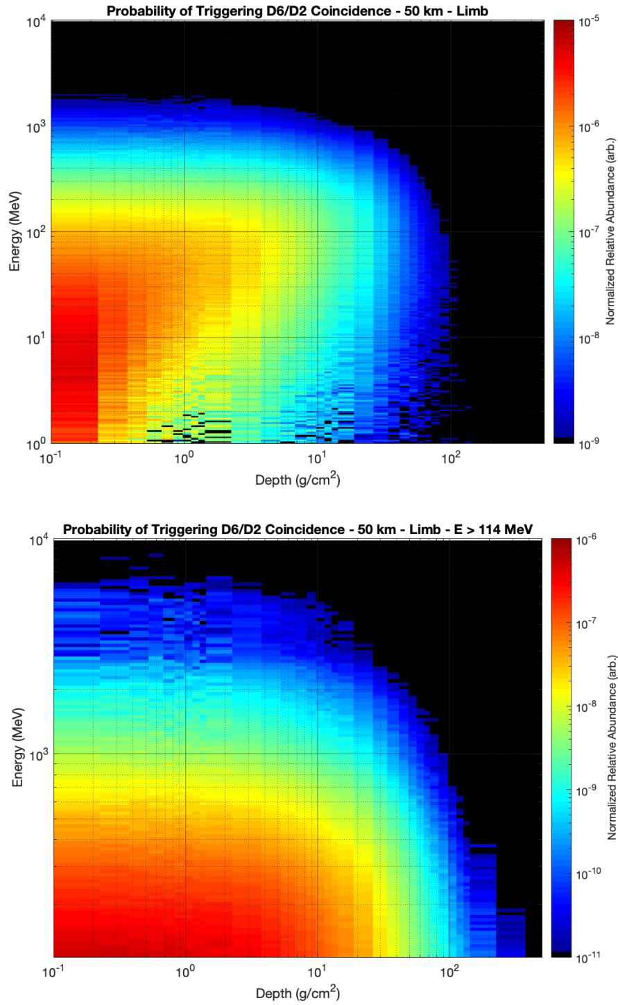
Figure 7.11. The maximum depth distribution of albedo protons triggering D6/D2 coincidence when facing the lunar limb at altitude of 50 km for all modeled energies (top) and above the threshold energy of 114 MeV (bottom).
