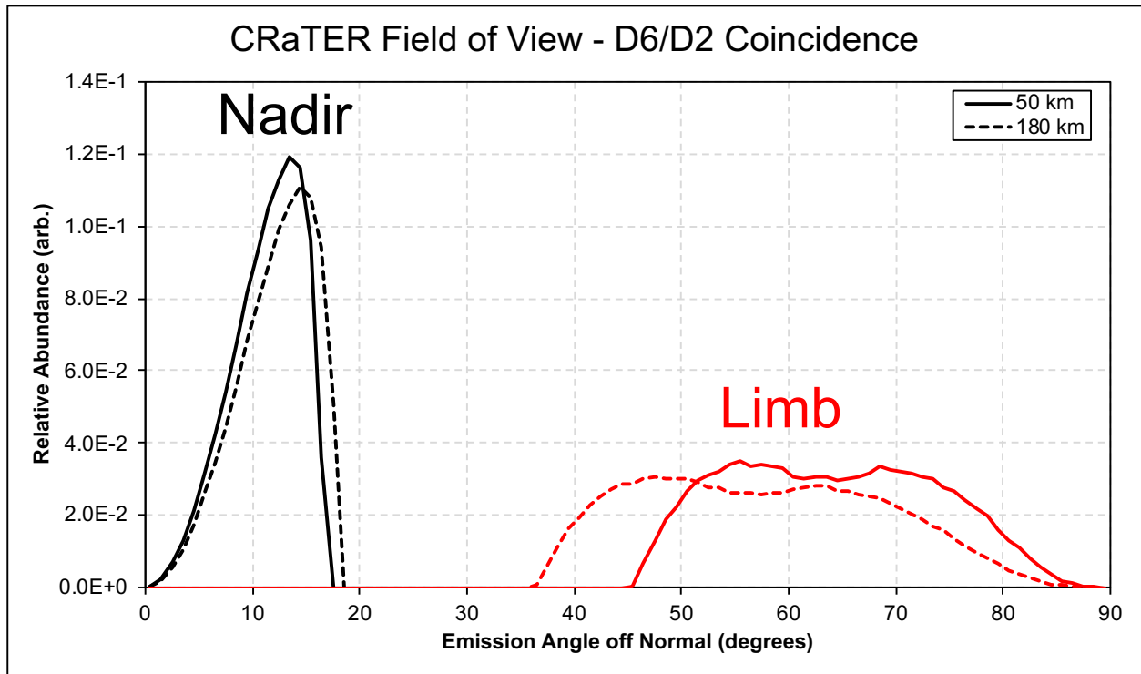
Figure 7.3. The probability of an albedo particle triggering D6/D2 coincidence at the CRaTER instrument as a function of surface emission angle off normal.
