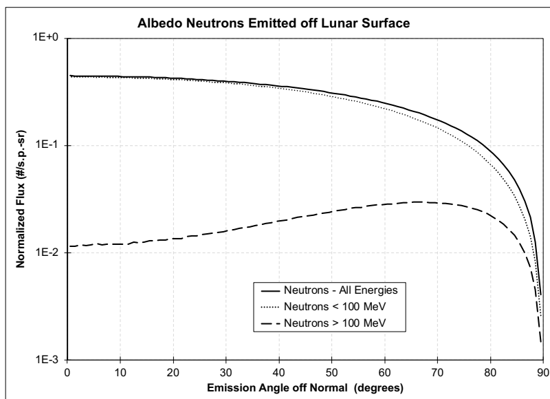
Figure 3.31. The angular distribution of albedo neutrons for two different energy ranges.
