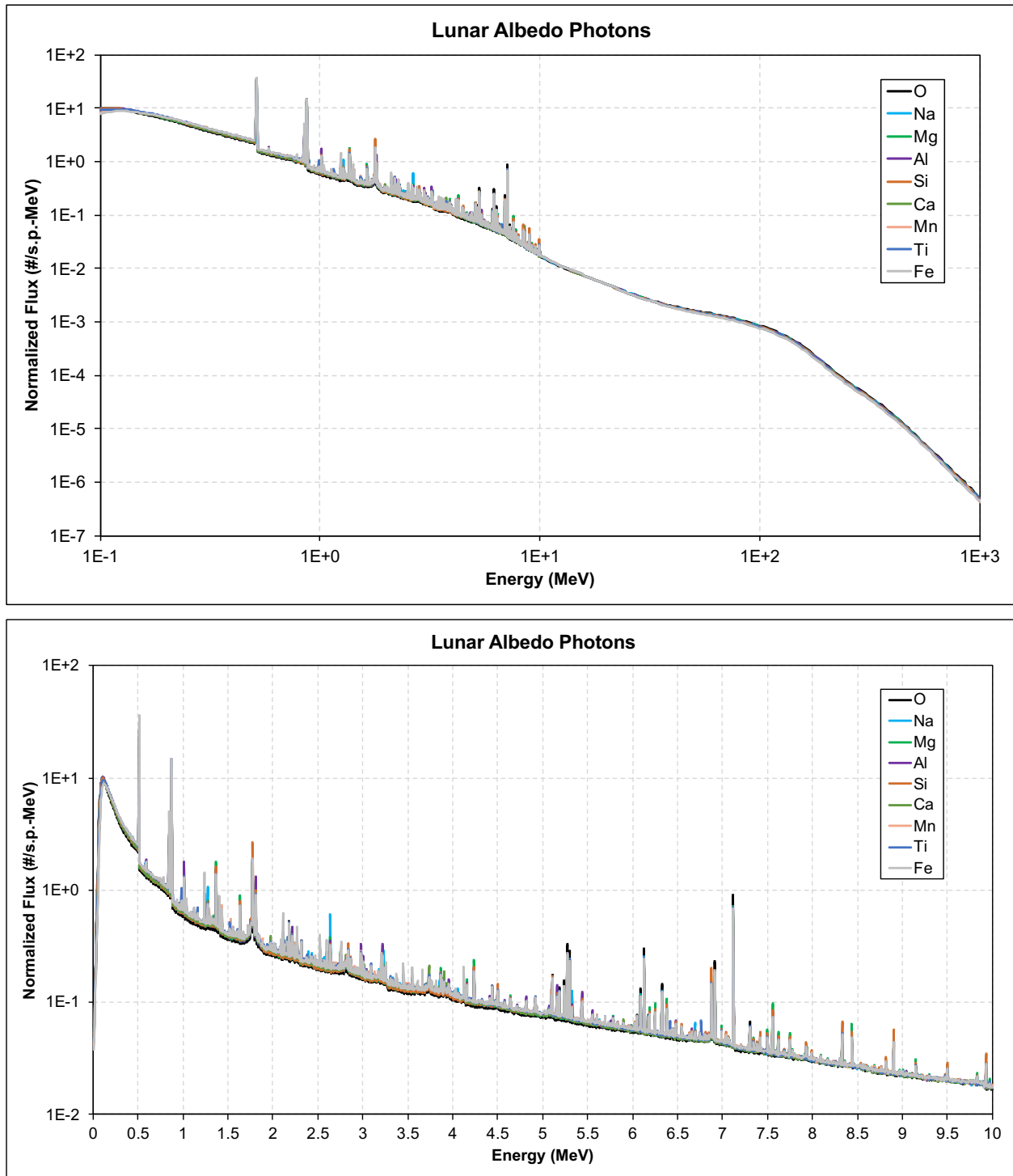
Figure 5.7. The energy spectrum of albedo photons emitted from nine different scenarios, each with a modeled regolith that has an increased content of the specified element for all energies studied (top) with a focus on the low energy part of the spectrum (bottom).
