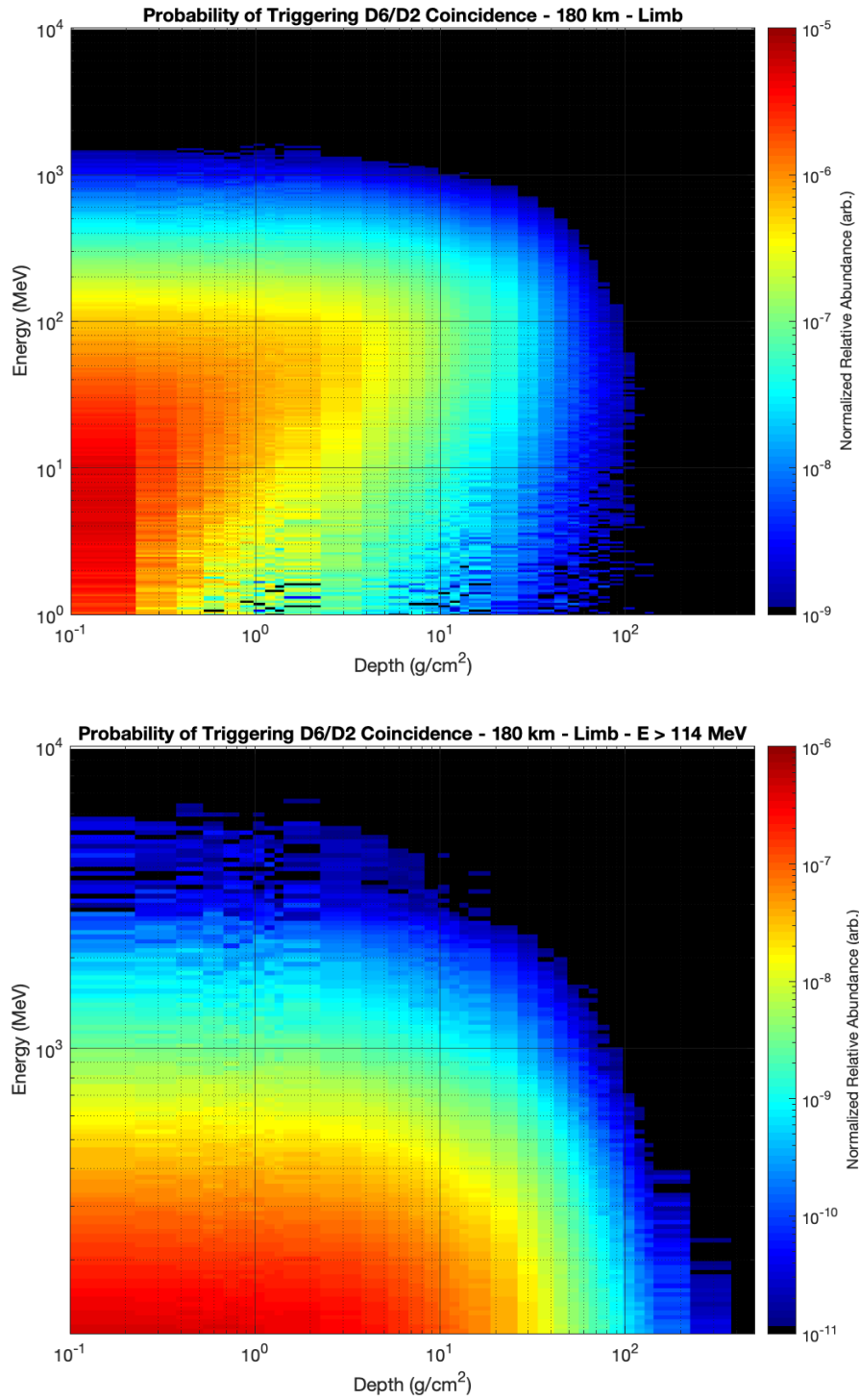
Figure 7.12. The maximum depth distribution of albedo protons triggering D6/D2 coincidence when facing the lunar limb at altitude of 180 km for all modeled energies (top) and above the threshold energy of 114 MeV (bottom).
