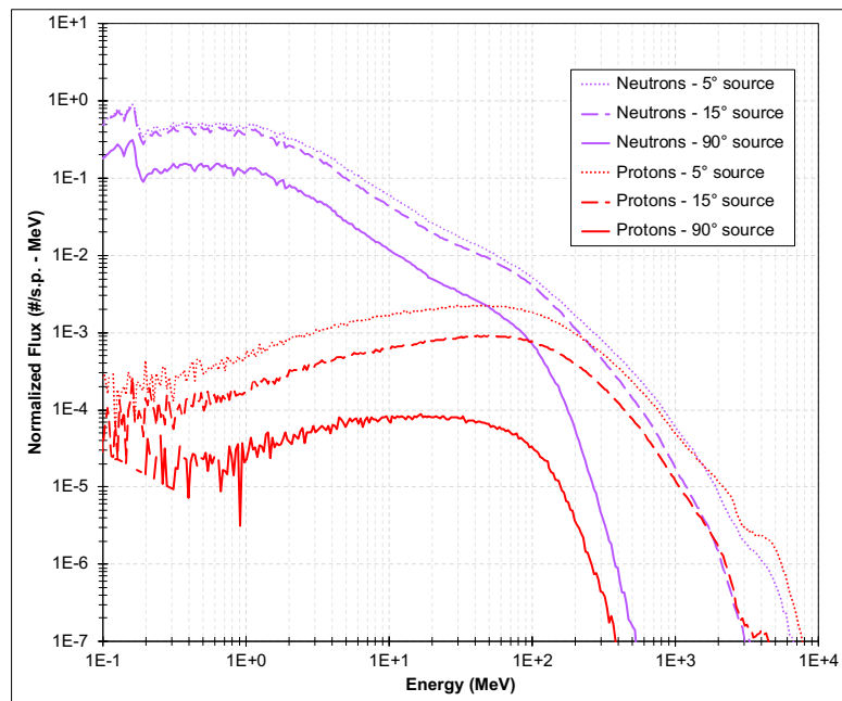
Figure 3.36. The energy distribution of albedo neutrons and protons from three monodirectional source terms pointing towards the regolith: 5 degrees off lunar surface, 15 degrees off lunar surface, and directly downward 90-degree source term.
