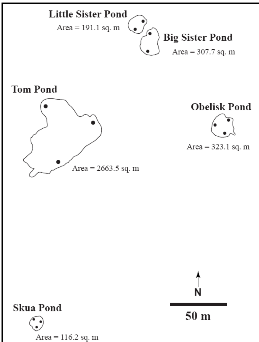
Figure 4. Map of Hjorth Hill Coast field site, depicting the relative location of the 5 ponds sampled for this study. Dots represent locations within the pond where samples were collected. The Ross Sea coast is located ~2 km to the east of Obelisk Pond.
