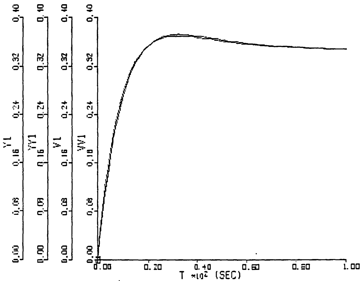
Figure 3.28: Reactivity inputs using the LDOC and RID control paradigms. Figure compares the unconstrained control signals ( Y_1, V_1 ) with the constrained ones ( YY_1, VV_1 ). In test-4, reactivity insertion rate and coolant flow rate are constrained.
