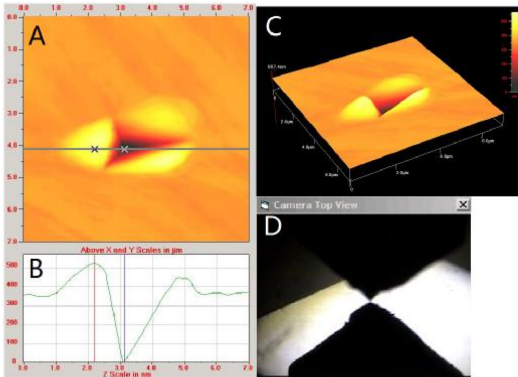
Figure 22 Slip-step patterns over the contact surface and the surrounding area of the \text{Zr}_{50}\text{Cu}_{40}\text{Al}_{10} BMGs.
