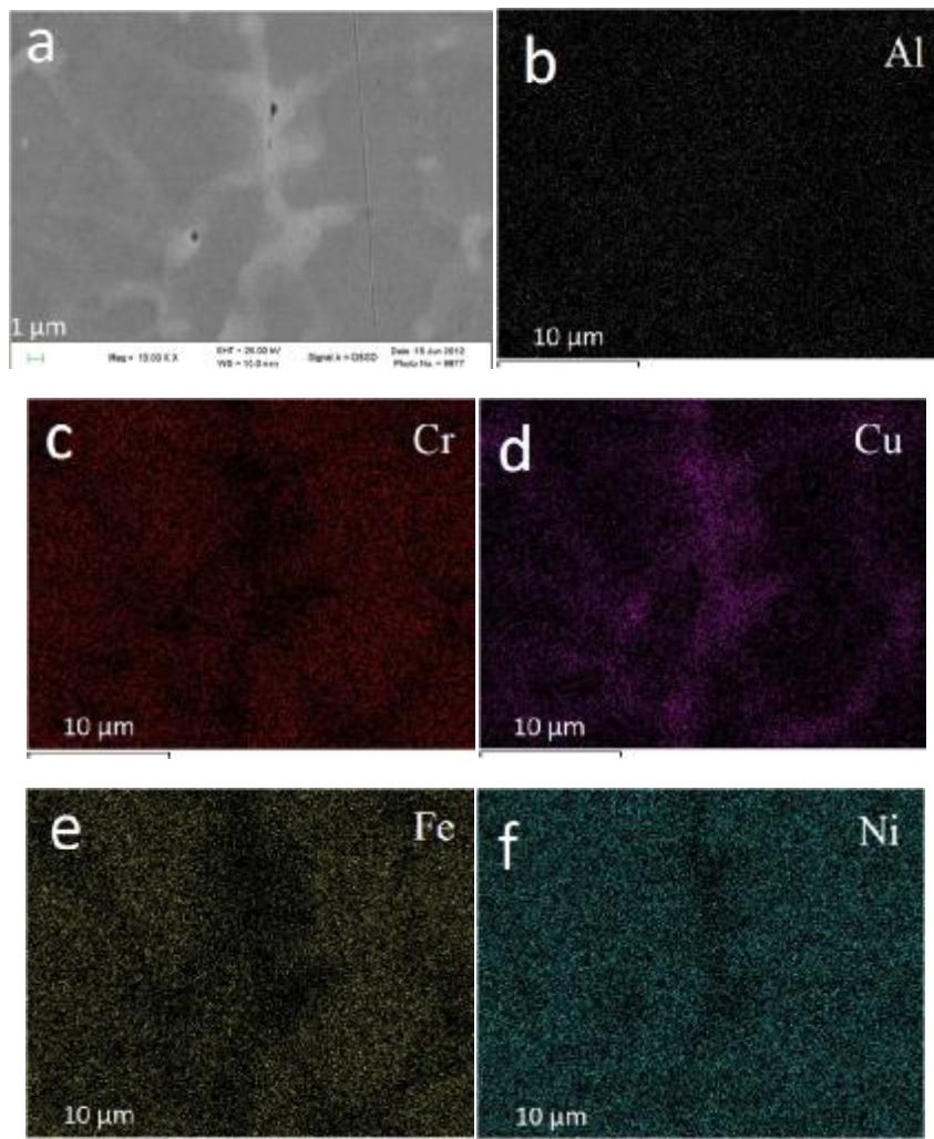
Figure 37 Elemental mapping of the \text{Al}_{0.5}\text{CrCuFeNi}_2 HEA.
