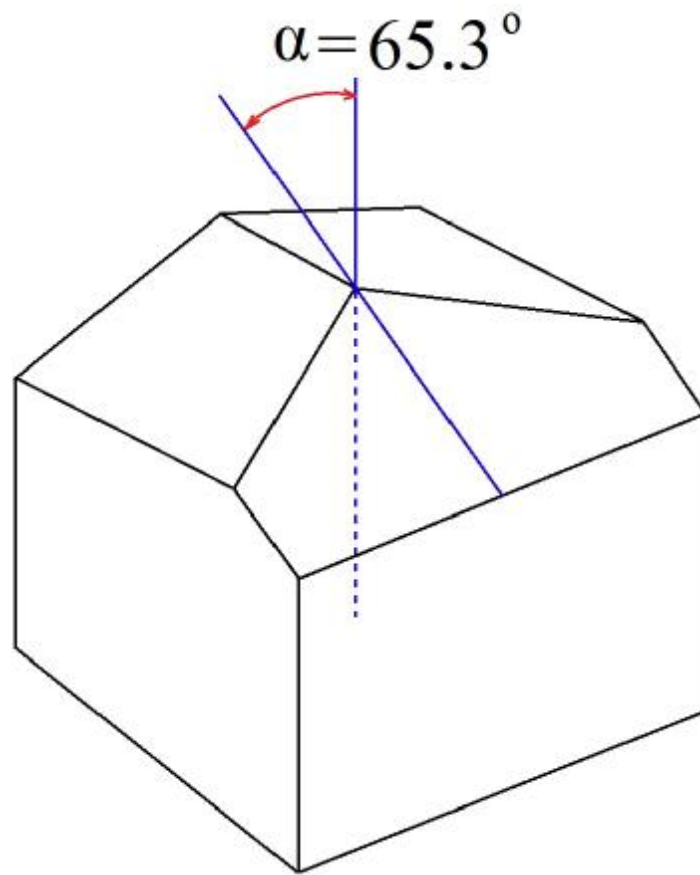
Figure 2 Berkovich indenter
