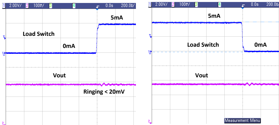
(b) Load regulation response, load switch turns on or off a resistor load. Turn on: 5mA, turn off: 0mA. V_{in} is set 1.5V.
