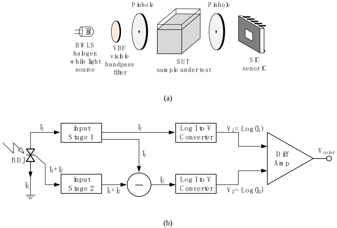
Fig. 3.1. (a) pH measurement setup diagram with optical sensor (b) and the block diagram of the CMOS SIC in [32].
