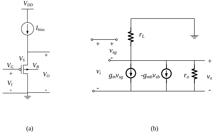
Fig. 4.2. (a) Input stage of the proposed pH readout system and (b) the small-signal equivalent circuit model with body effect.
