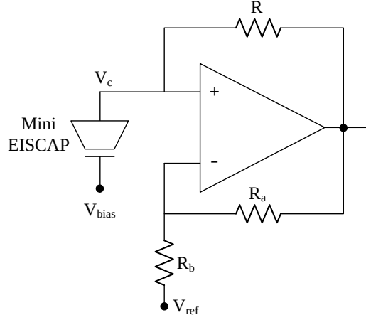
Fig. 3.5. Schematic of the EISCAP relaxation oscillator.
