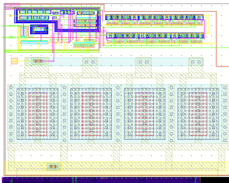
Fig. 4.24. Layout of the old pH Readout Circuit (114 \mu\text{m} x 86 \mu\text{m} ).
