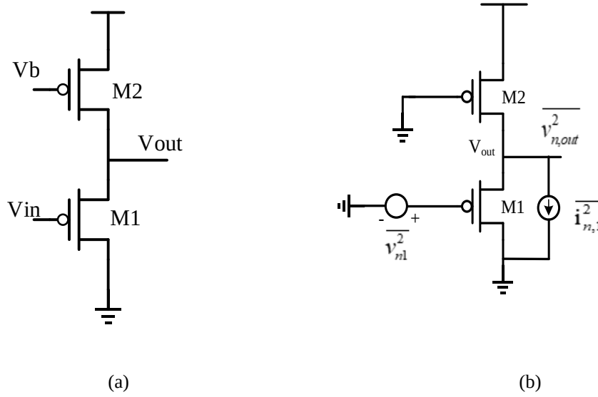
Fig. 4.14. (a) Basic level shifter structure and (b) noise model for the level shifter device.
