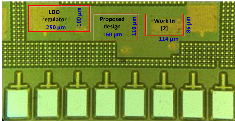
Fig. 5.1. Chip photo with bond pads.
