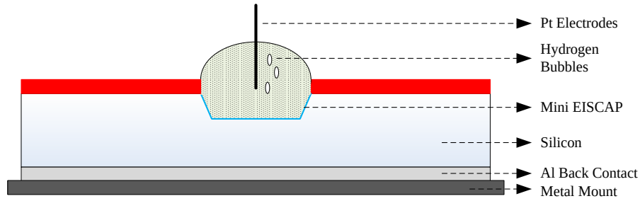
Fig. 3.4. The structure of the EISCAPs pH sensor in [38].
