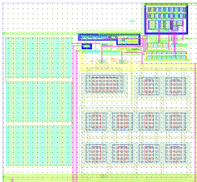
Fig. 4.23. Layout of the proposed pH Readout Circuit (200 \mu\text{m} x 140 \mu\text{m} ).
