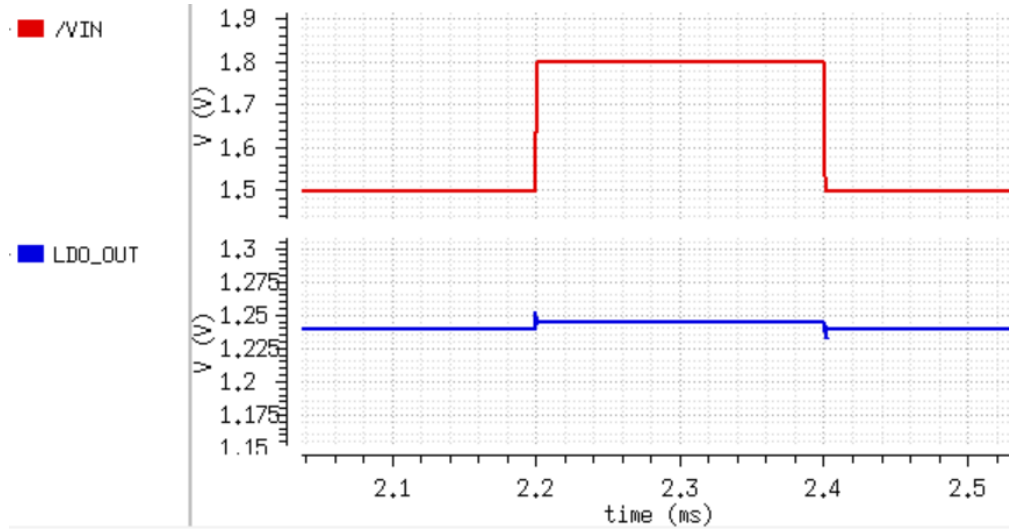
(a) Line regulation response with load current set to 1mA.
