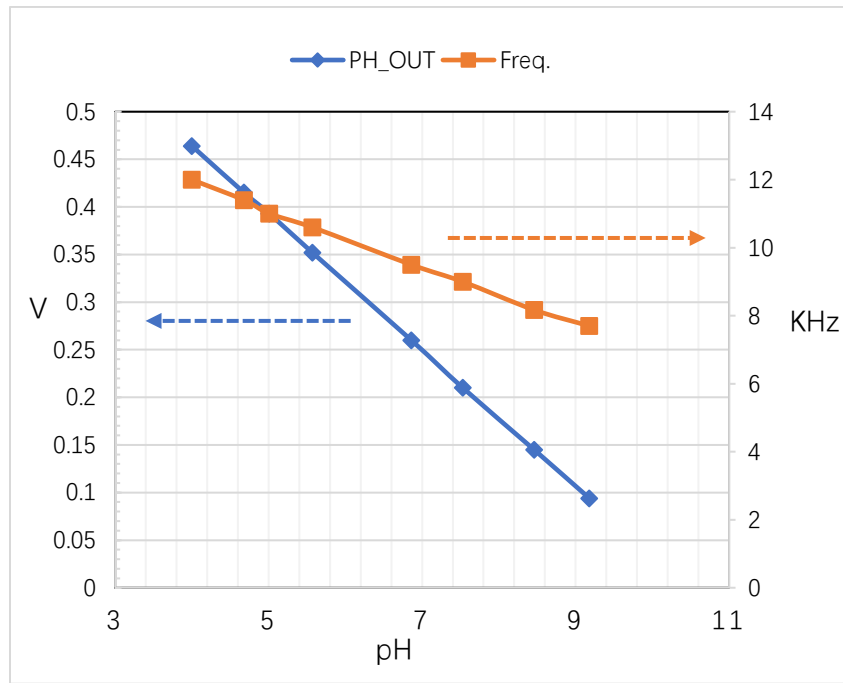
Fig. 5.10. pH sensor output voltage measurement system output frequency versus input pH values.
