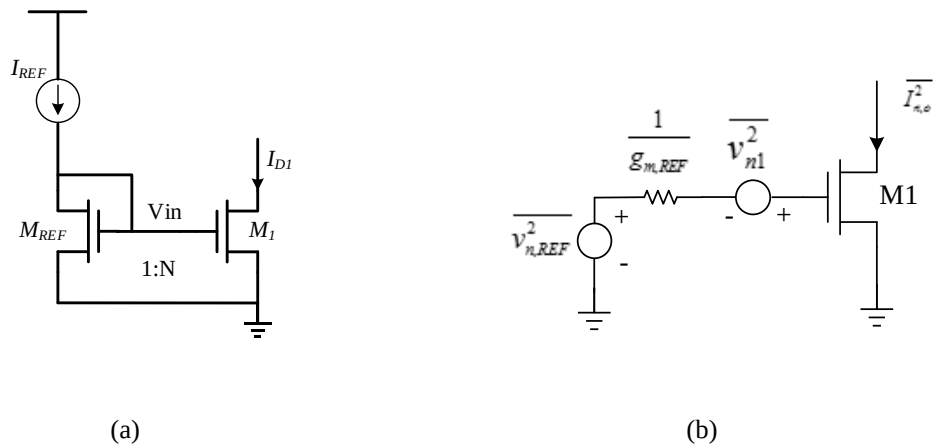
Fig. 4.16. (a) Basic current mirror structure and (b) circuit model for noise analysis.
