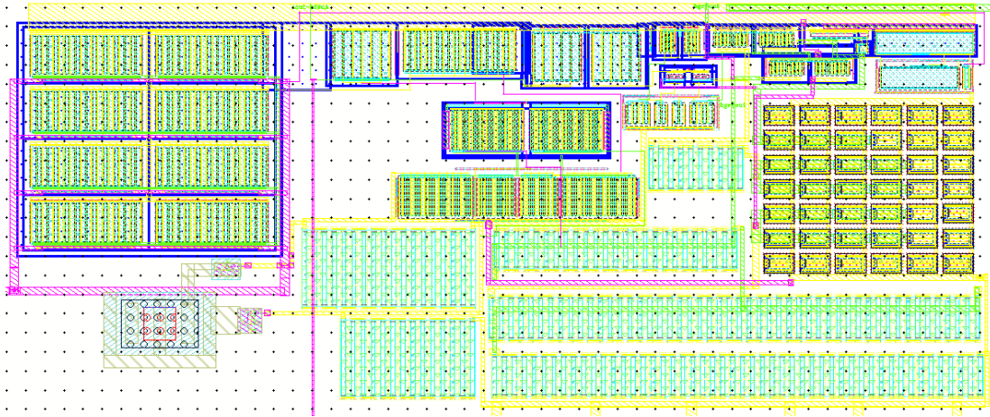
Fig. 4.22. Layout of the LDO and Bandgap Circuit (250 \mu m x 100 \mu m).
