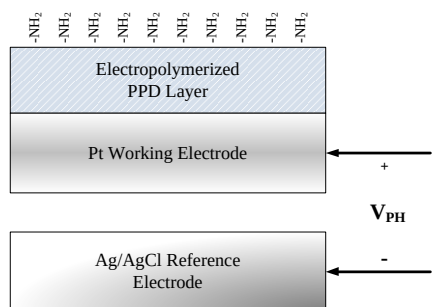
Fig. 3.7. Ag/AgCl reference electrode and Pt working electrode of the coil-type pH sensor.
