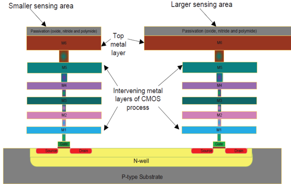
Fig. 3.3. Cross section views the differential ISFET in [45].
