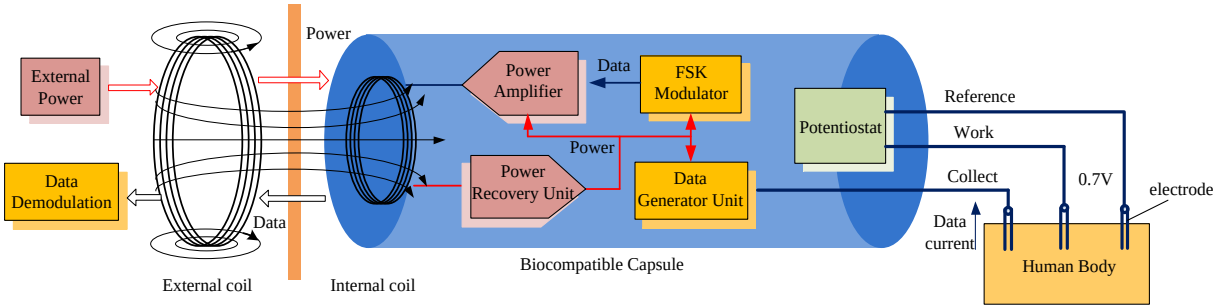
Fig. 2.1. Block diagram of the inductively-powered implant system [21].
