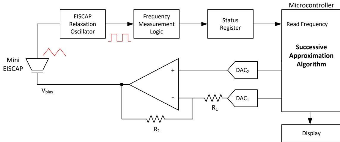
Fig. 3.8. Block diagram of the pH measurement system in [38].
