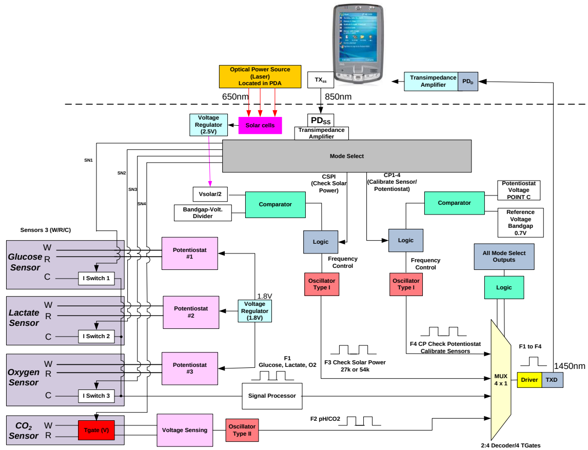
Fig. 2.2. Multi-analyte sensor architecture where instructions are received from a transmitter located in the PDA unit.
