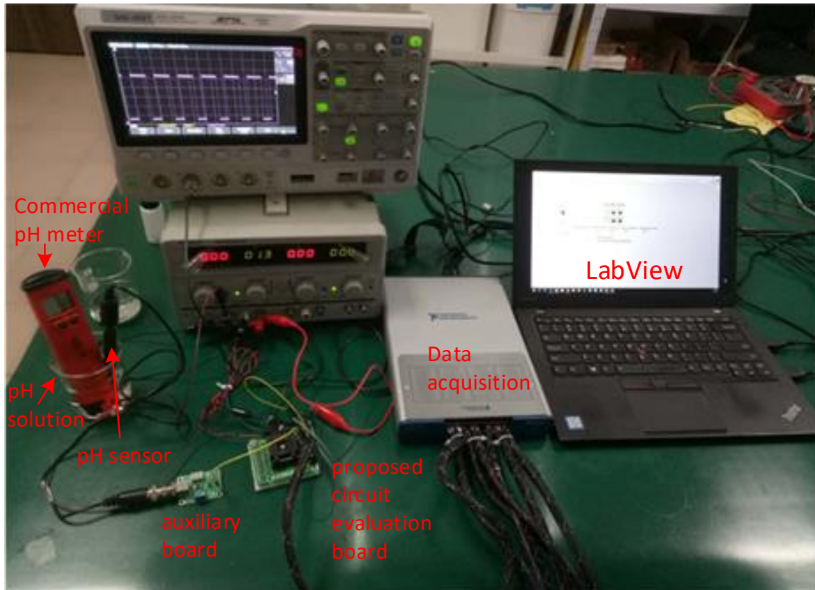
Fig. 5.9. In-vitro test setup for the pH measurement system in this work, including solution, pH sensor/electrode, and an auxiliary board. Auxiliary board provides a proper socket and RC filter. A National Instruments™ acquisition system is employed to transfer data from the proposed circuit to computer.
