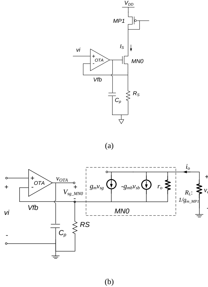
Fig. 4.3. (a) Voltage buffer including the OTA and MN0 with source degeneration R_S to generate current proportional to input voltage with MP1 as load and (b) its small signal model including body effect. MP1 is diode-connected and can be modeled as a resistor 1/g_{m\_MP1} .
