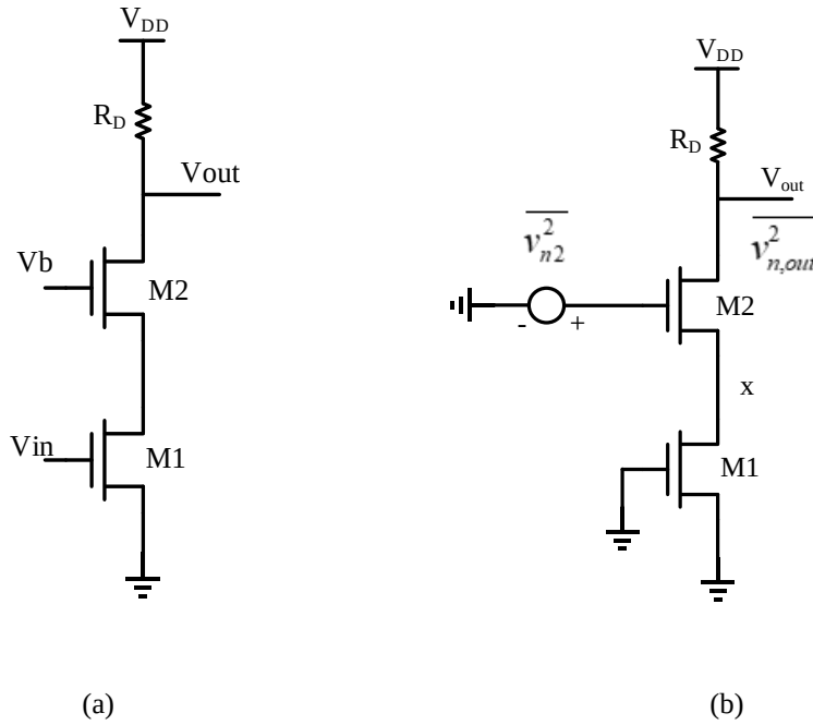
Fig. 4.15. (a) Basic cascode structure and (b) noise model for cascode device
