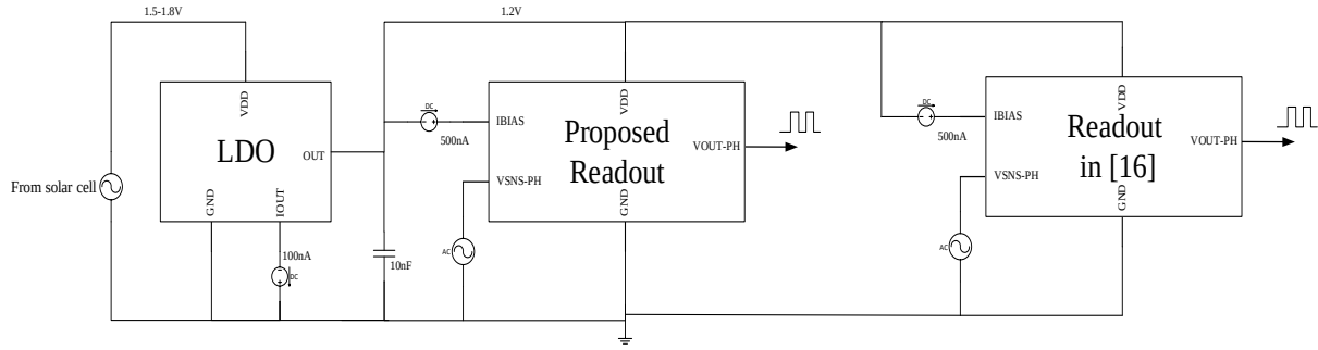
Fig. 4.18. The test bench setup.
