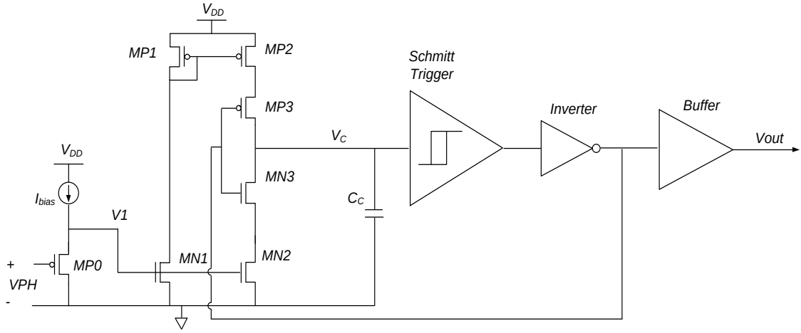
Fig. 3.11. Relaxation oscillator based readout circuit reported in [16].
