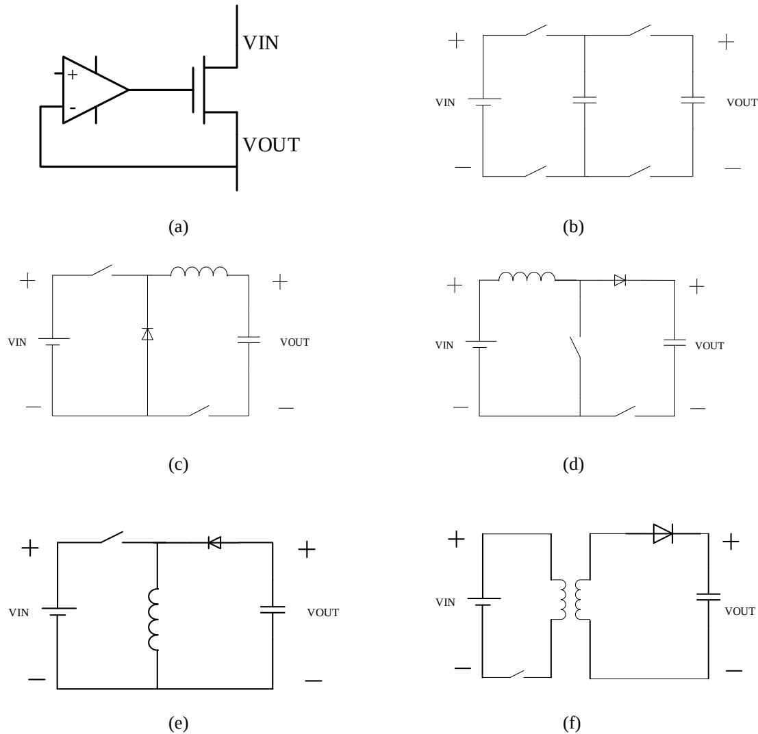
Fig. 3.12. Six typical voltage regulator topologies, (a) linear regulator, (b) charge pump, (c) step-down (Buck), (d) step-up (Boost), (e) inverter, and (f) Flyback. The input voltage is V_{IN} and the output voltage is V_{OUT} . From (c) to (f), these four topologies are so-called “switch-mode regulators”.
