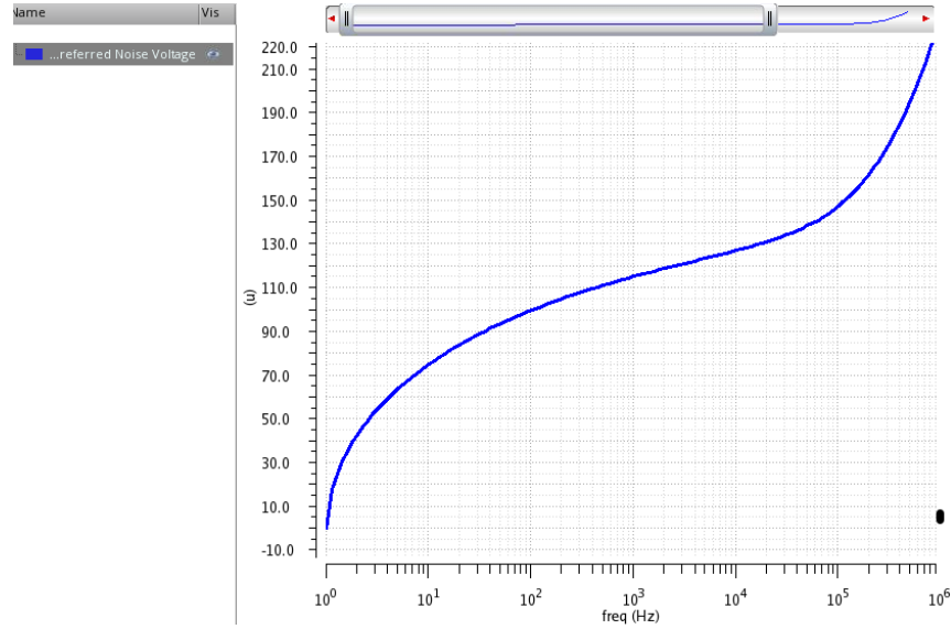
(b) Integrated input-referred noise voltage, integrating from 1Hz to 1MHz.
