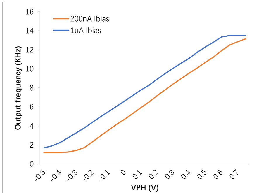
Fig. 5.4. Output frequency comparison with 200nA and 1 \mu A I_{bias} current.
