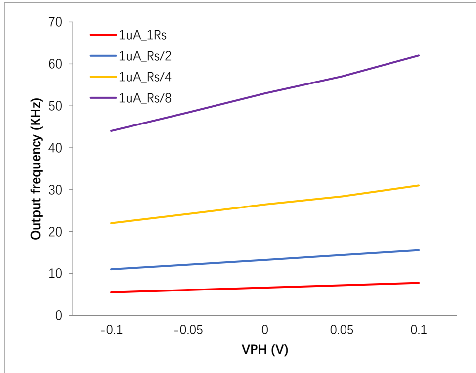
Fig. 4.21. The simulated output frequency under 1\mu A I_{bias} and different scaled resistance. The sensitivity increases from 11.35KHz/V to 90KHz/V. The current consumption increases as well, but it is scaled up. The simulated current for R_S , R_S/2 , R_S/4 , R_S/8 are 11.2 \mu A , 12.8 \mu A , 16.1 \mu A and 20.5 \mu A , respectively.
