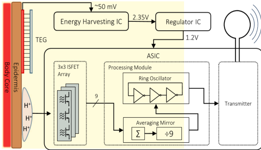
Fig. 3.9. The diagram of the system, showing the application set-up of an on-body TEG and skin-facing sensor, the main components of the ASIC and the power management ICs, reported in [43].
