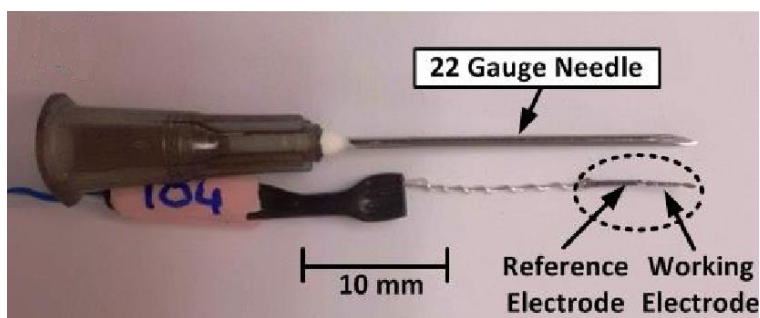
Fig. 5.7. Photograph of the fabricated electrochemical sensor alongside a 22-gauge needle for size comparison.
