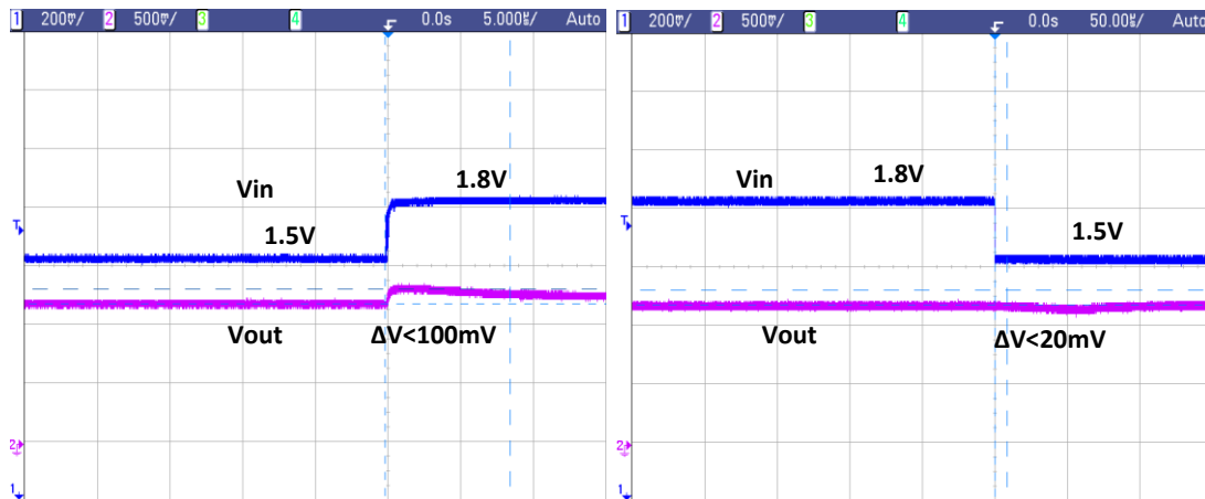
(a) Line regulation response, V_{in} is set to be a waveform ranging from 1.5V to 1.8V with 10ns rise/fall time, load current is 1mA.
