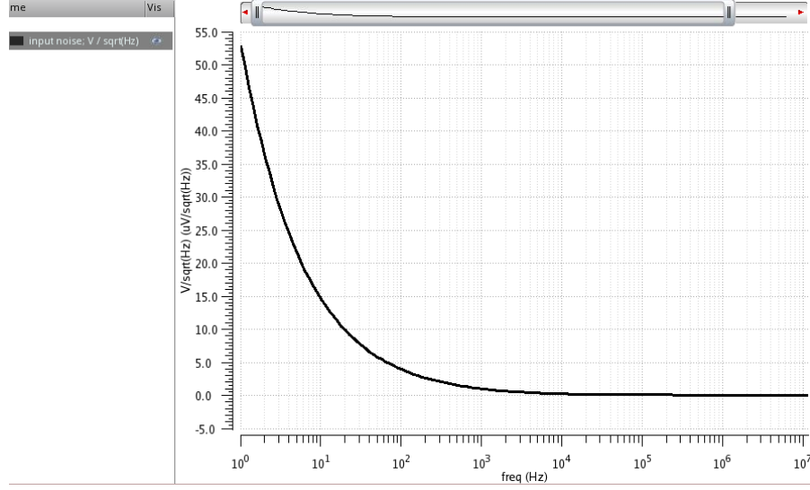
(a) Input-referred noise spectrum density
