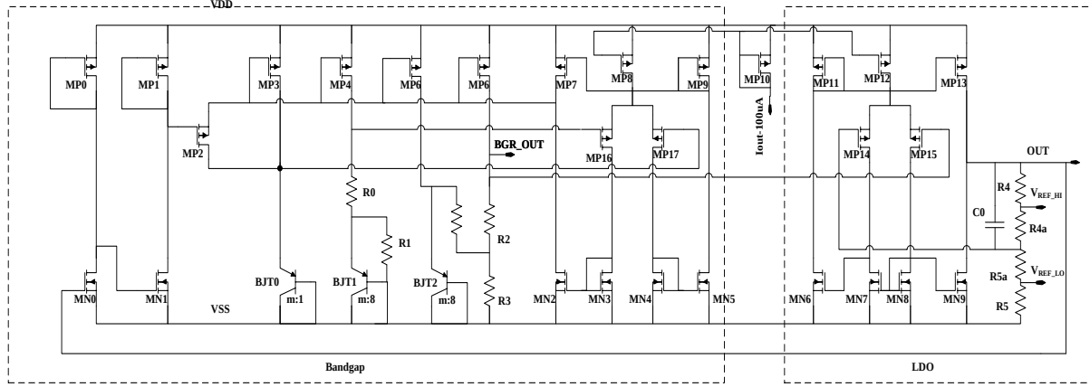
Fig. 4.9. Schematic of low voltage, high PSRR LDO with bandgap reference circuit.
