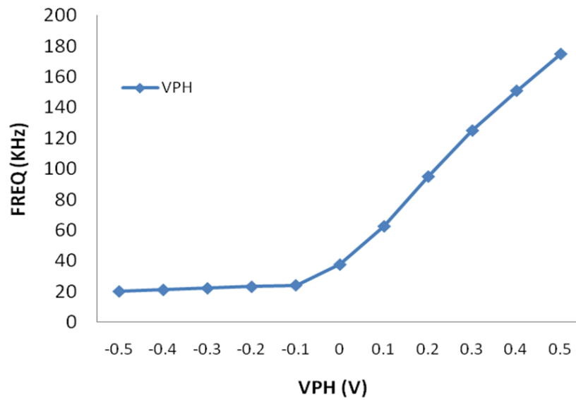
Fig. 4.19. Linearity of the old PH Readout circuits implemented in 0.13- \mu\text{m} process as a comparison.
