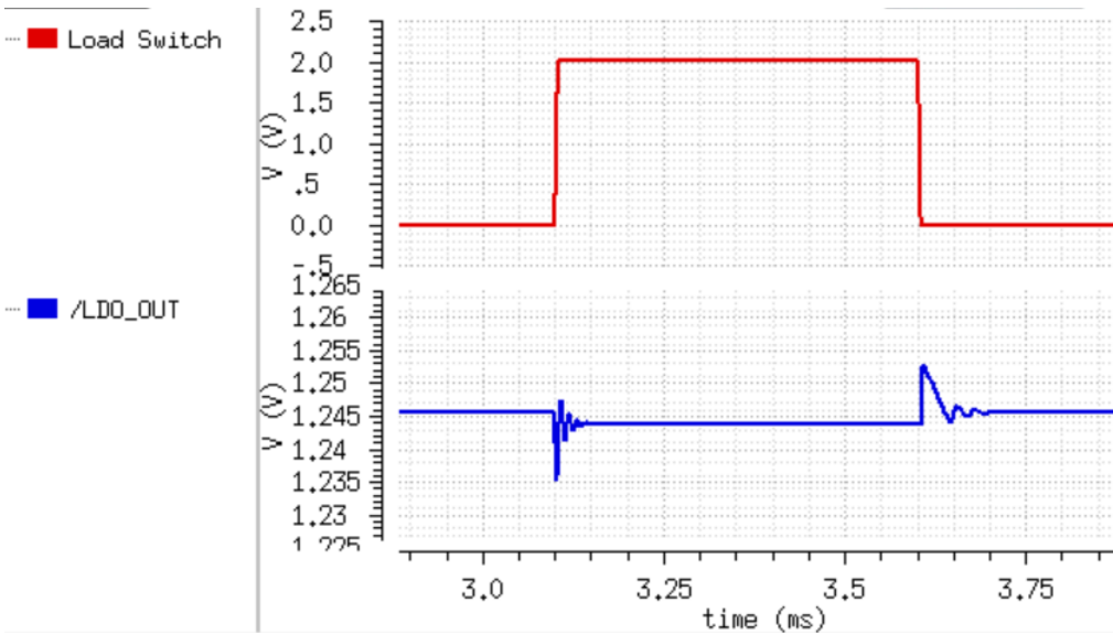
(b) Load regulation response, with 0~5mA load pulse. V_{in} is set 1.5V.
