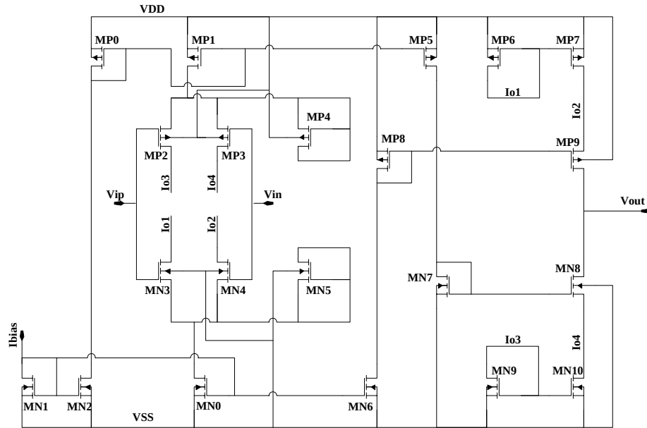
Fig. 4.6. Schematic of the OTA used in the pH circuit.
