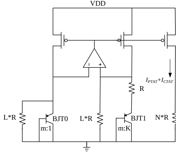
Fig. 4.8. Low supply voltage bandgap reference circuit.
