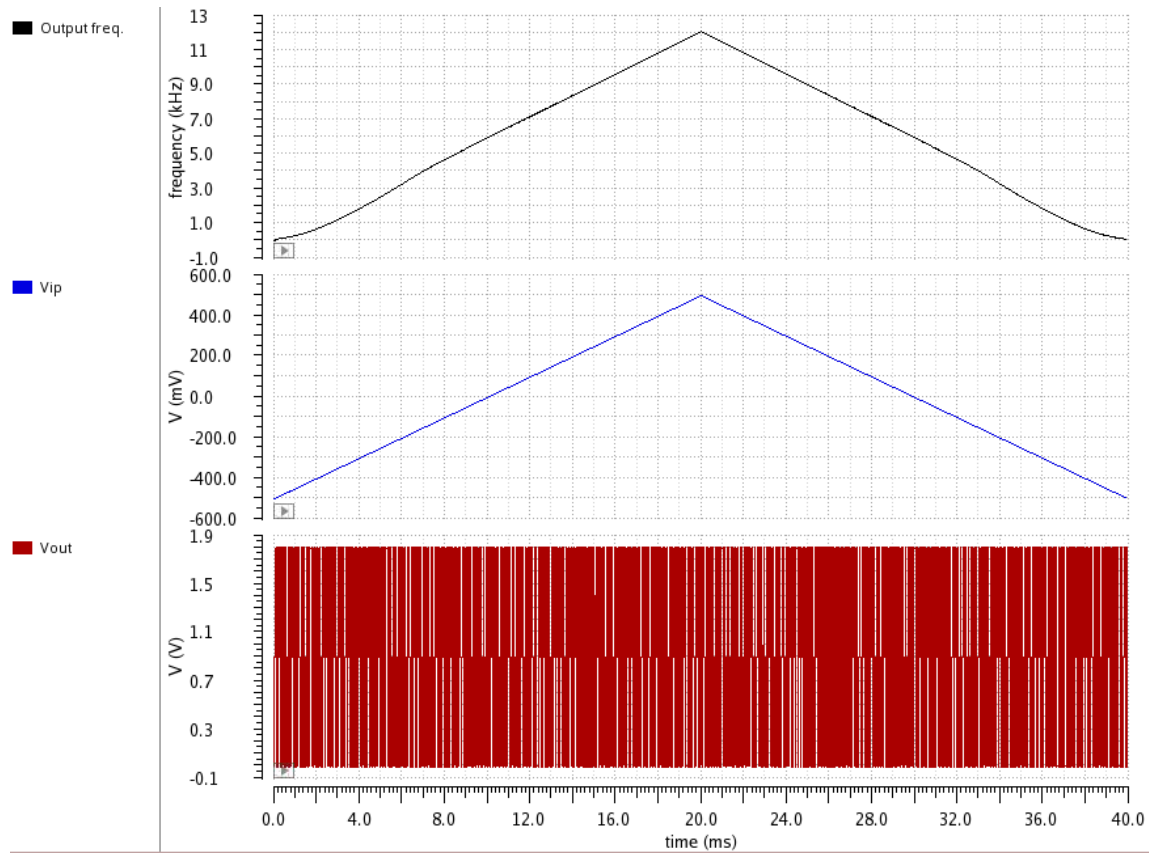
Fig. 4.20. The simulated output frequency sweeping V_{pH} values.
