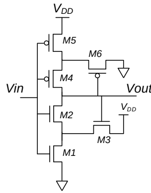
Fig. 4.4. Schematic of the CMOS Schmitt Trigger in [16].
