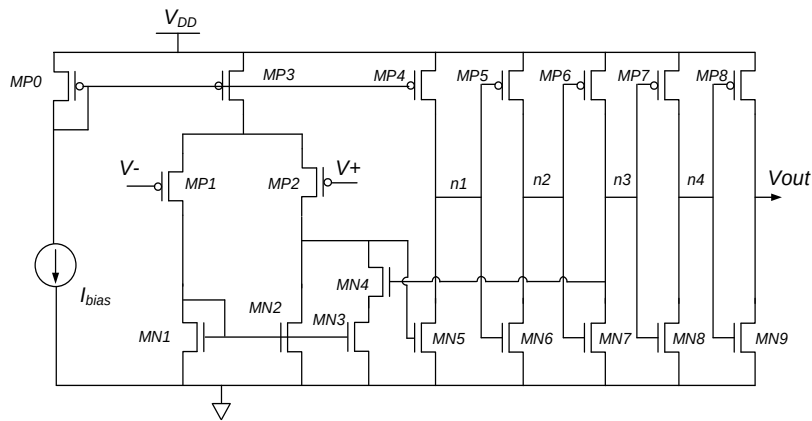
Fig. 4.5. Schematic of the comparator used in the pH circuit.
