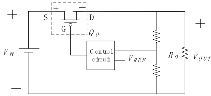
Fig. 3.13. Typical topology of a linear voltage regulator.
