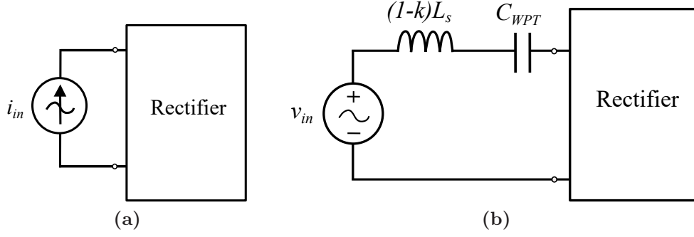
Figure 6.2: Diagrams of the (a) current model built with an input current source and (b) suggested model accounting for the low coupling coefficient.
