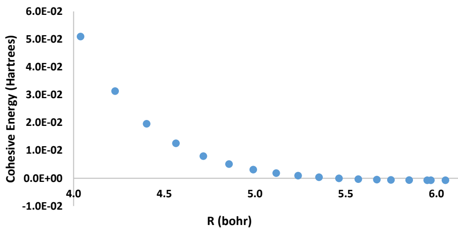
Figure 4.9: Cohesive Energy Vs Nearest Neighbor Distance
