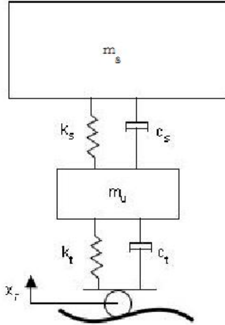
Figure 2.1: Simple representation of two degree of freedom suspension system
