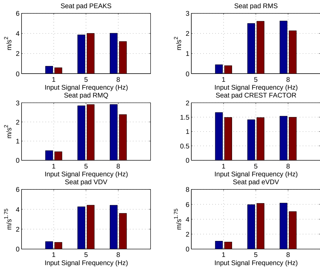
Figure 6.22: Results: Accelerometer-Seatpad- Whole body vibration evaluation parameters: Blue bar-test and Red bar-sim
