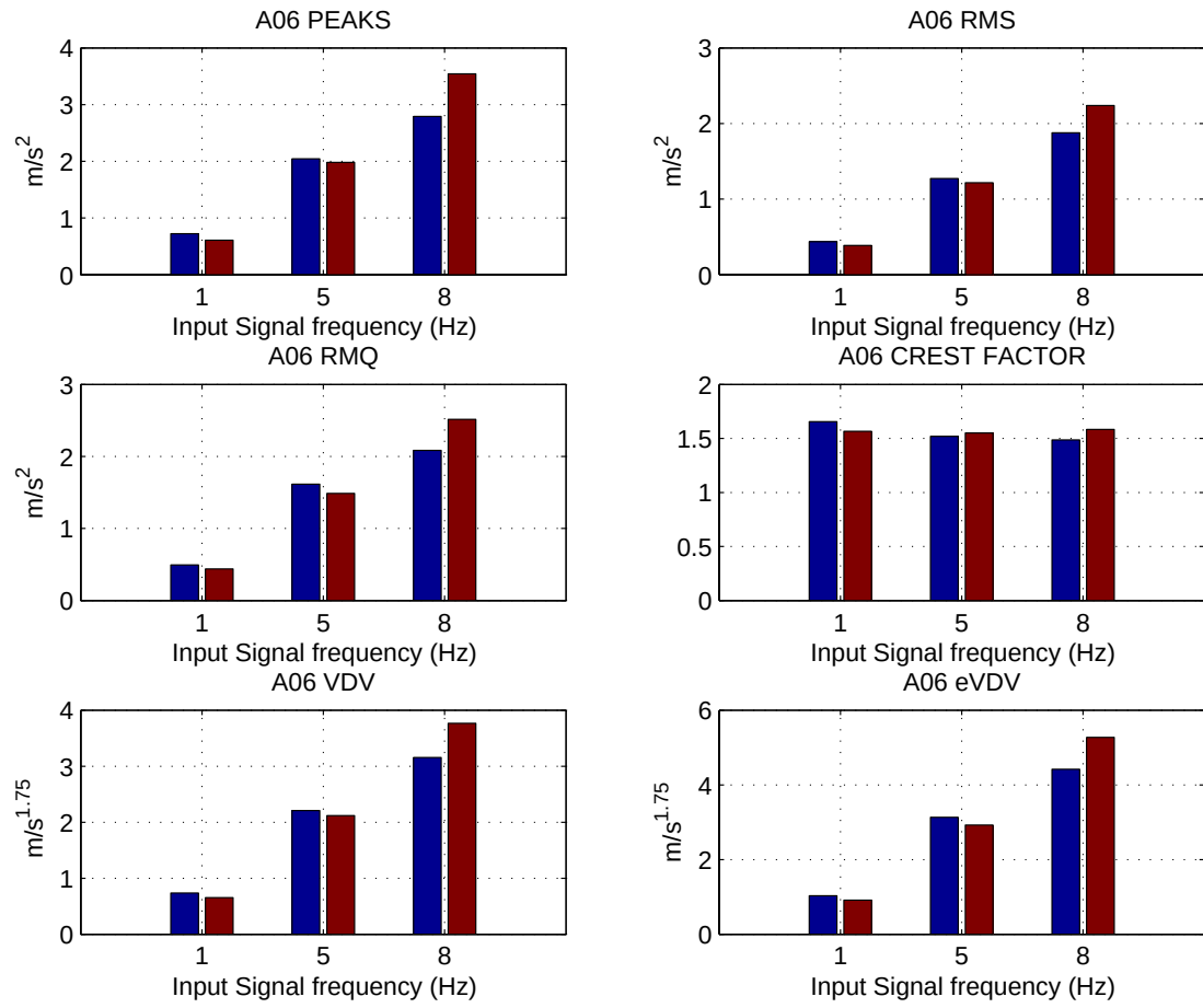
Figure 6.20: Results: Accelerometer-06- Whole body vibration evaluation parameters: Blue bar-test and Red bar-sim
