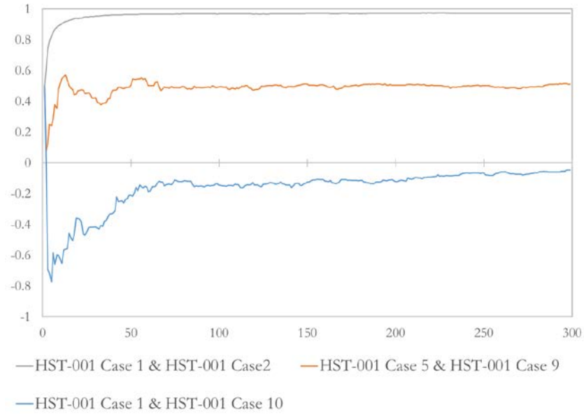
Figure 81. Convergence of three selected correlation coefficients.
