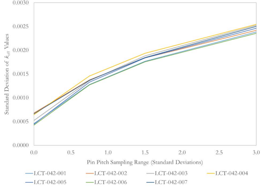
Figure 60. Standard deviation of k_{\text{eff}} values for 300 realizations converged to 0.00010 \Delta k .
