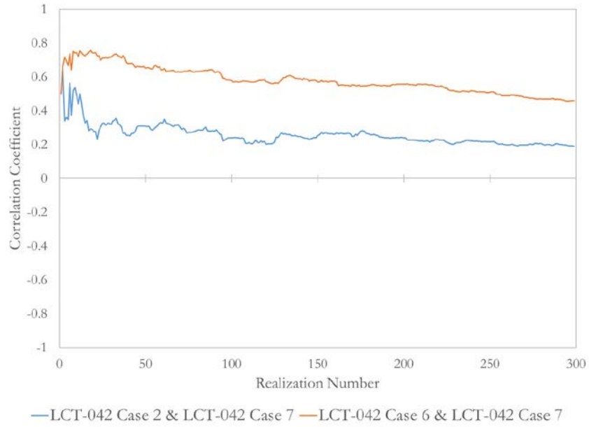
Figure 69. Convergence of two correlation coefficients, random fuel rod positions.
