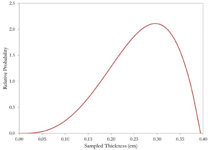
Figure 45. PDF for the plexiglass stiffener thickness in LCT-042 Case 5.
