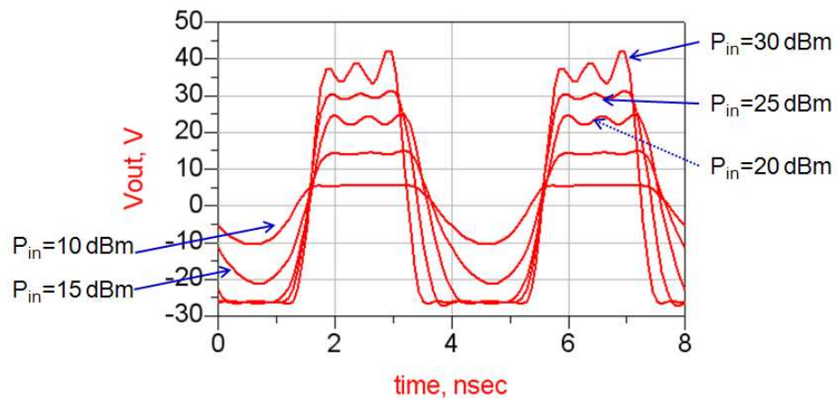
Figure 4.8 Transient drain voltage vs. input power
