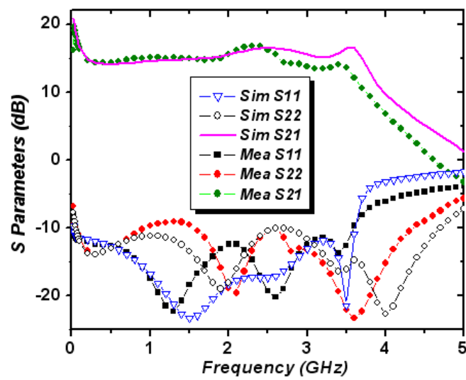
Figure 2.29 Simulated & measured small signal S parameters of optimized DPA
