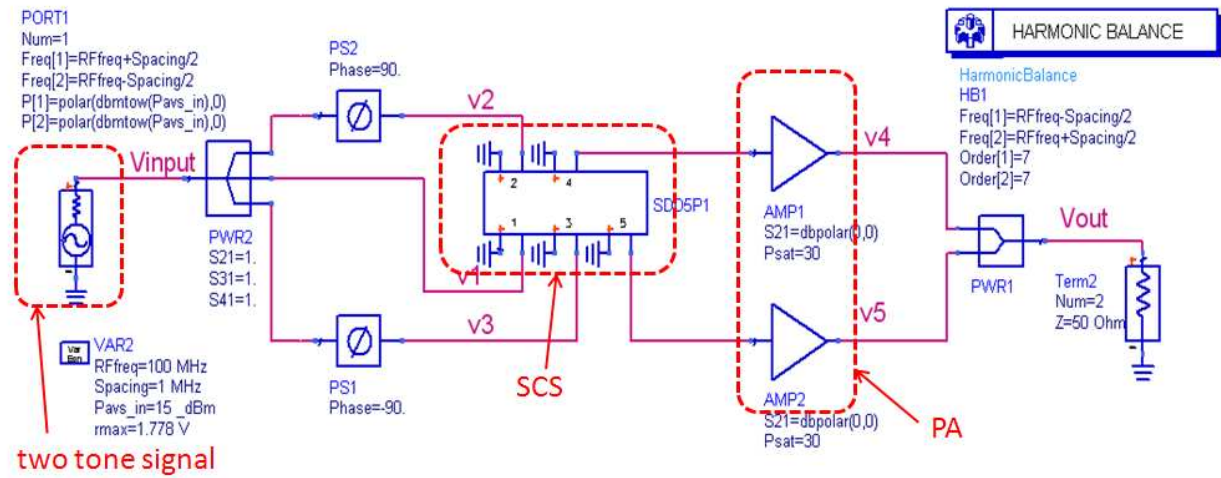
Figure 3.3 LINC transmitter using Wilkinson combiner
