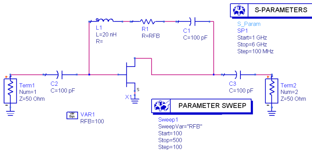
Figure 2.13 Schematic of simplified feedback amplifier
