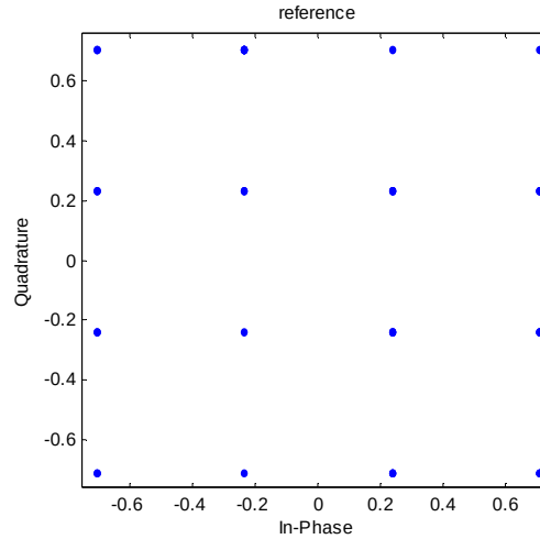
Figure 6.10 Constellation of an ideal 16 QAM signal used as a reference signal
