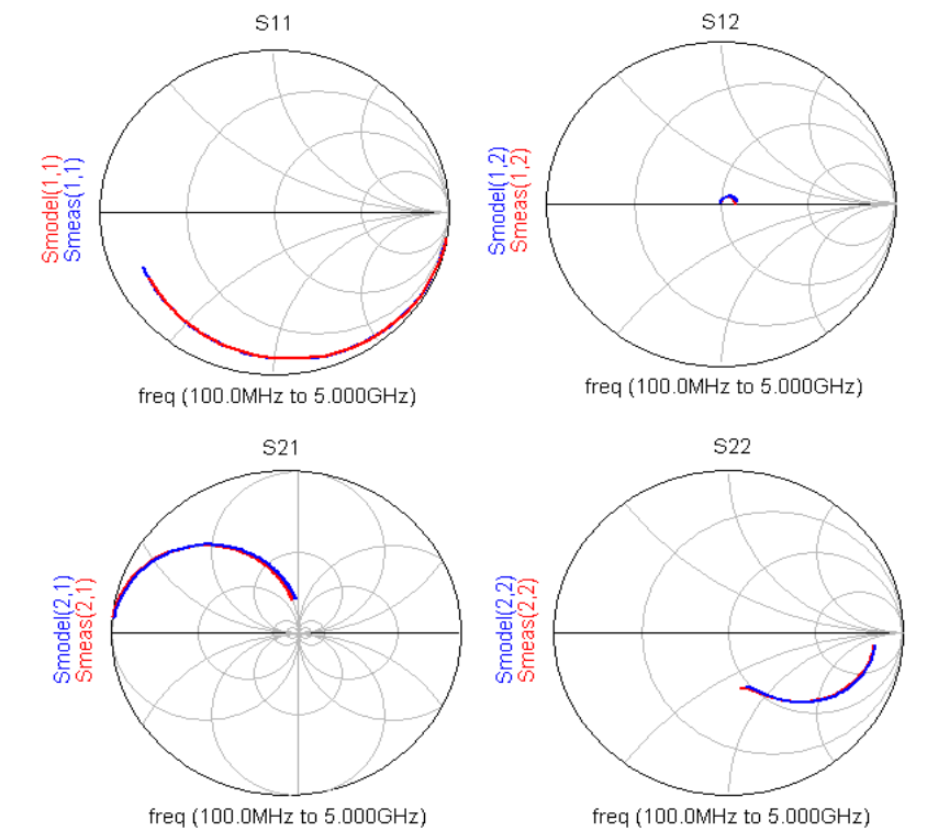
Figure 2.12 Comparison of the S-parameters of optimized linear equivalent model with extracted S-parameters
