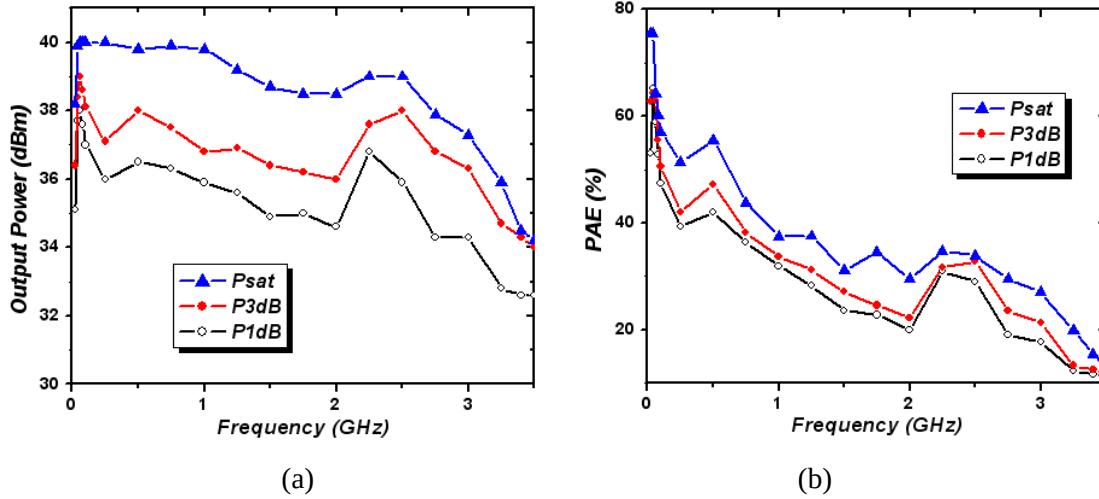
Figure 2.30 Measured power performance of the optimized DPA: (a) Output power; (b) PAE
