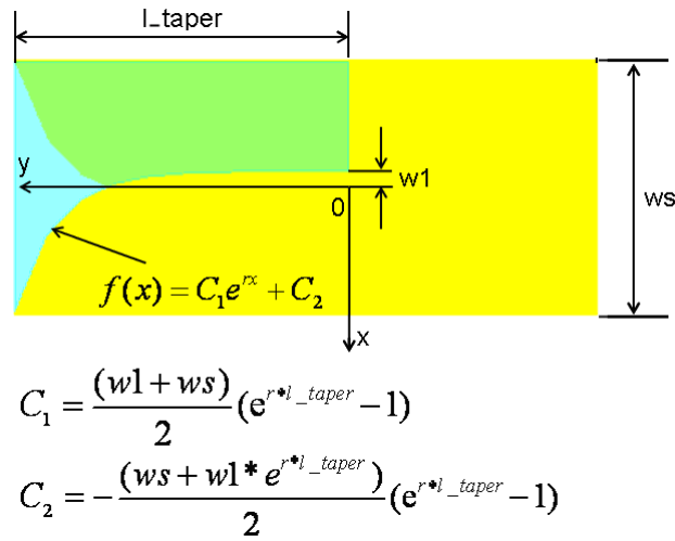
Figure 7.6 Configuration of the proposed antipodal Vivaldi antenna
