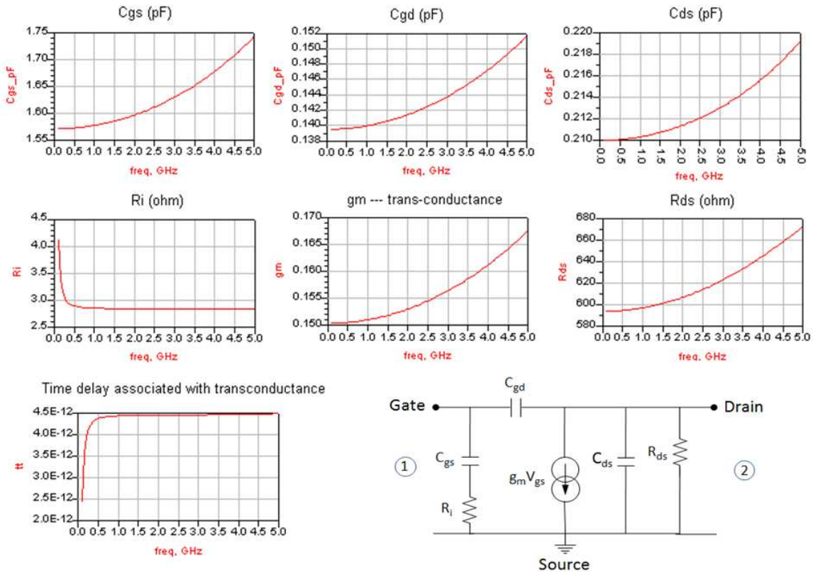
Figure 2.10 Extracted component values
