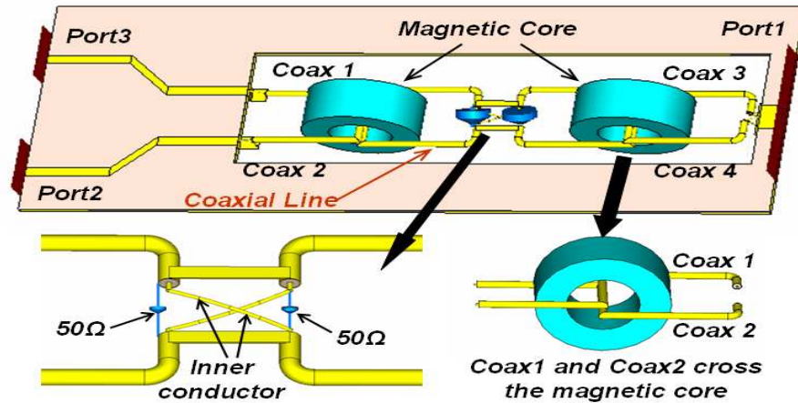
Figure 5.10 CST model of the modified splitter; ATC power resistors were utilized in our implementation and have modeled as ideal 50\ \Omega resistors given that their small parasitic capacitance (1.0 pF) can be neglected
