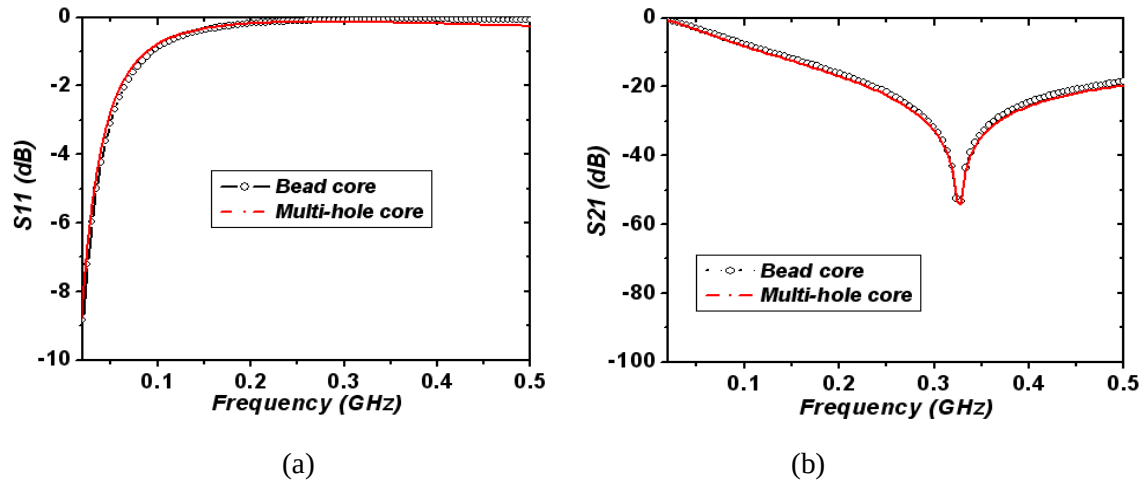
Figure 5.3 CST simulation results of bead core structure with \epsilon_r=250 and multi-hole core structure with \epsilon_r=125 : (a) S_{11} ; (b) S_{21}
