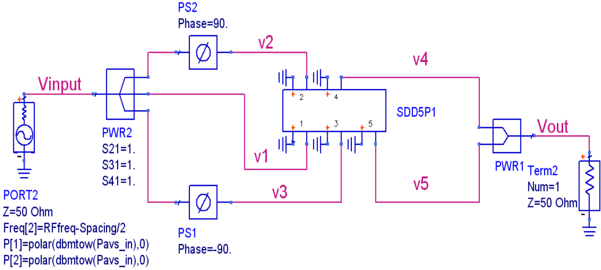
Figure B1. Simplified LINC transmitter
