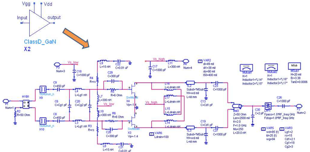
Figure C3. Wide band class D power amplifier (50 to 550 MHz) Eudyna GaN HEMT (EGN045MK)
