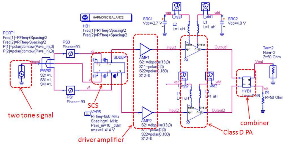
Figure 6.4 LINC transmitter with two-tone signal
