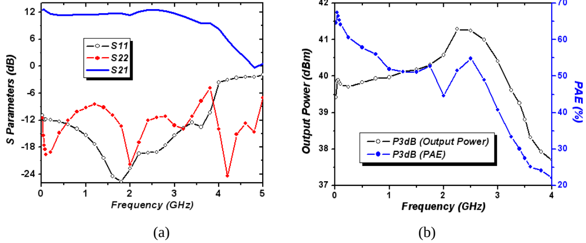
Figure 2.26 Simulation results: (a) large signal S parameters with a 27 dBm input power; (b) P_{3dB} performance of the optimized DPA.
