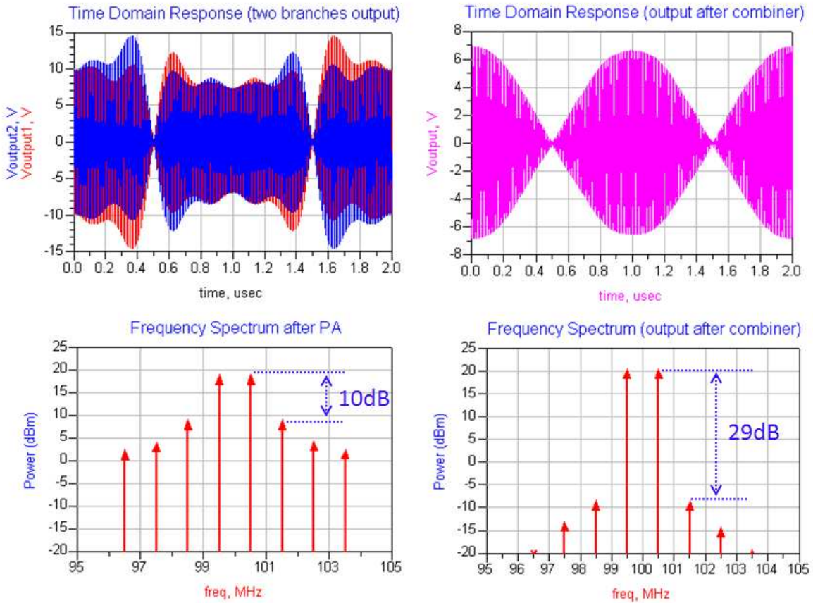
Figure 3.4 Simulation results of LINC transmitter using Wilkinson combiner
