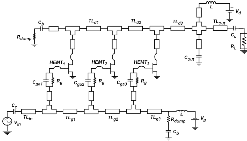
Figure 2.25 Schematic of the optimized tapered drain line DPA
