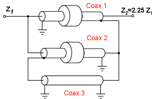
Figure 5.4 Simple model of a 1:2.25 impedance transformer
