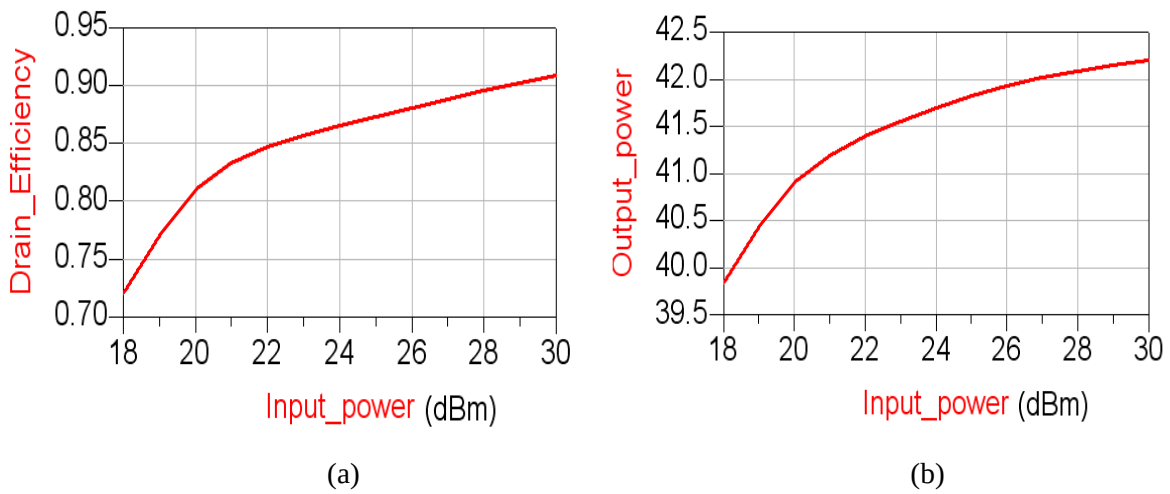
Figure C2. (a) Drain efficiency vs. input power; (b) Output power vs. input power
