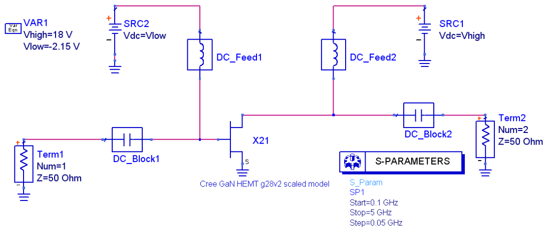
Figure 2.9 Schematic to extract S-parameter from large signal model
