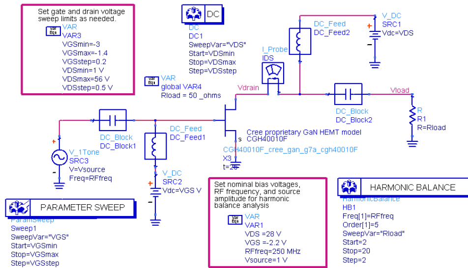
Figure 4.5 DC sweep schematic
