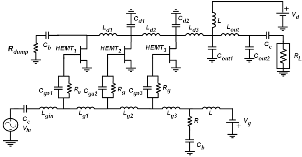
Figure 2.24 Schematic of the simplified tapered drain line DPA with ideal lumped elements
