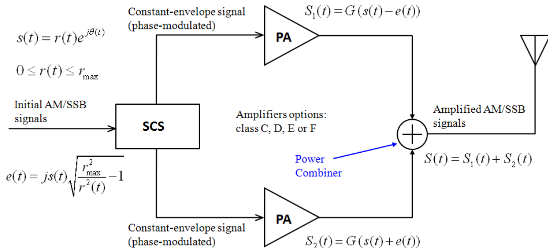
Figure 3.1 A simplified LINC transmitter schematic [40]
