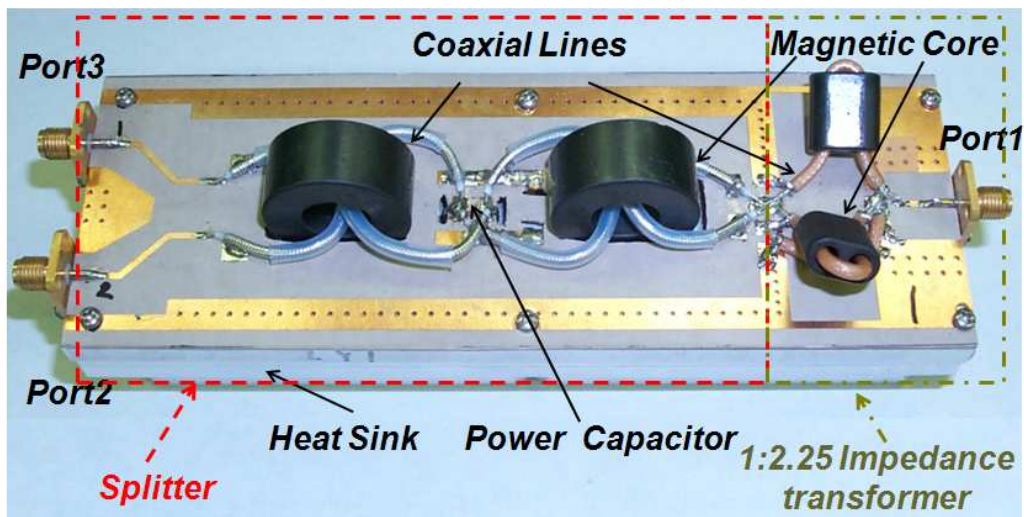
Figure 5.11 (a) Simulation structure (combined CST & ADS) (b) Fabricated combiner (the splitter with the 1:2.25 impedance transformer)
