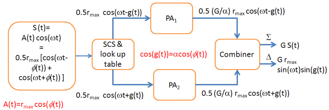
Figure 6.7 Transmitter Schematics: (a) Conventional LINC; (b) Adaptive bias LINC
