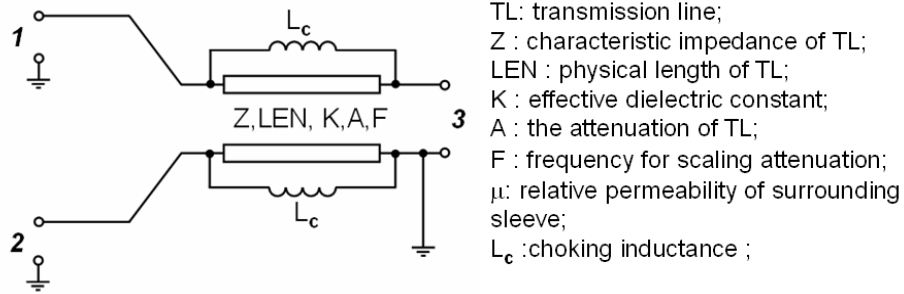
Figure 5.1 Balun Equivalent model [64]
