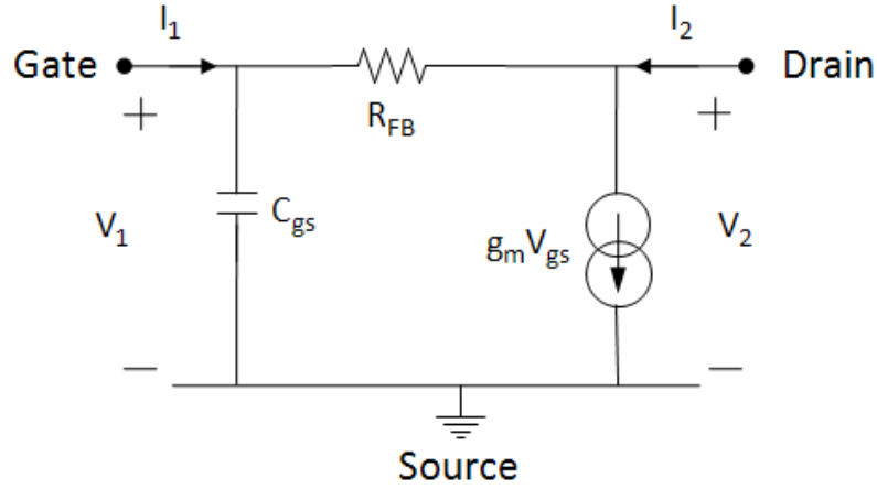
Figure A2. FET feedback equivalent circuit
