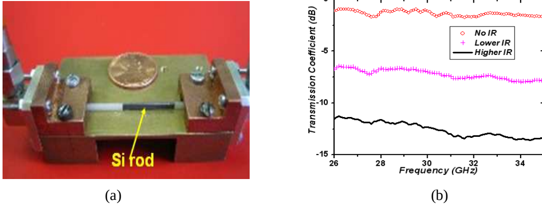
Figure 7.14 Optical controlled attenuators: (a) Fabricated attenuator; (b) Measured results
