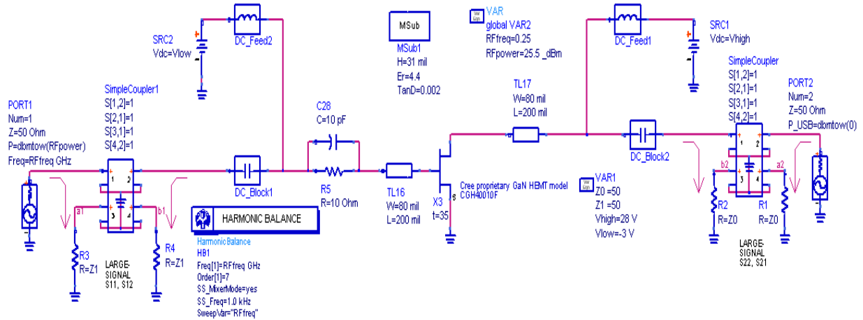
Figure 4.9 ADS simulation setup for large signal S parameters
