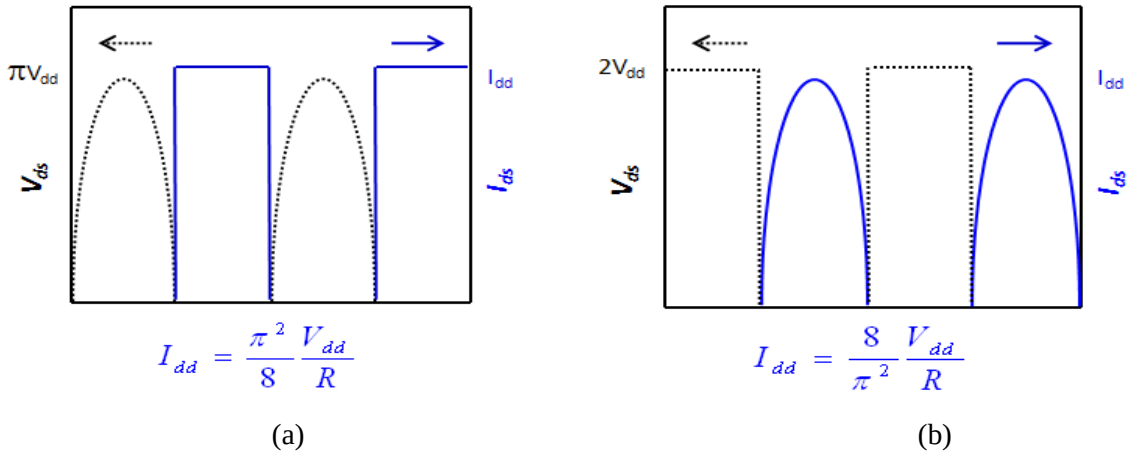
Figure 4.3 Class D PA transient waveforms: (a) CMCD; (b) VMCD
