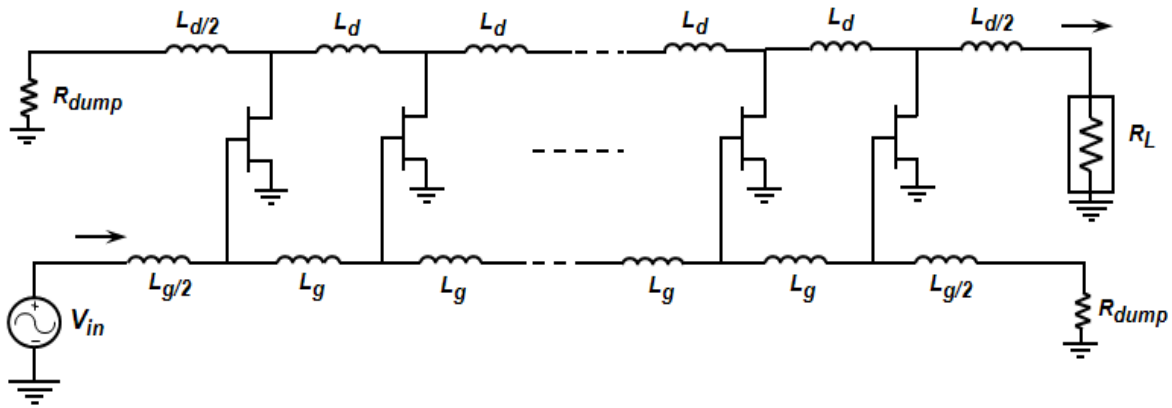
Figure 2.22 Schematic diagram of a conventional distributed amplifier
