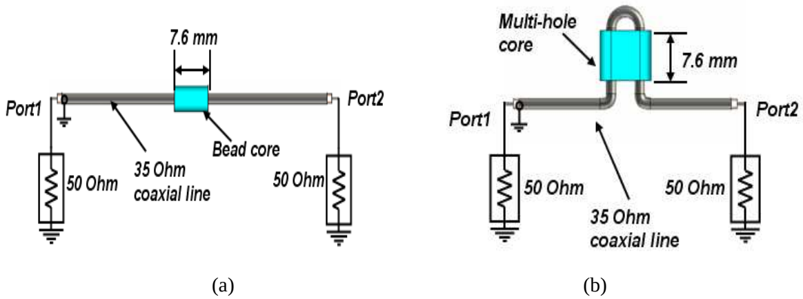
Figure 5.2 CST model: (a) Bead core structure; (b) Multi-hole core structure
