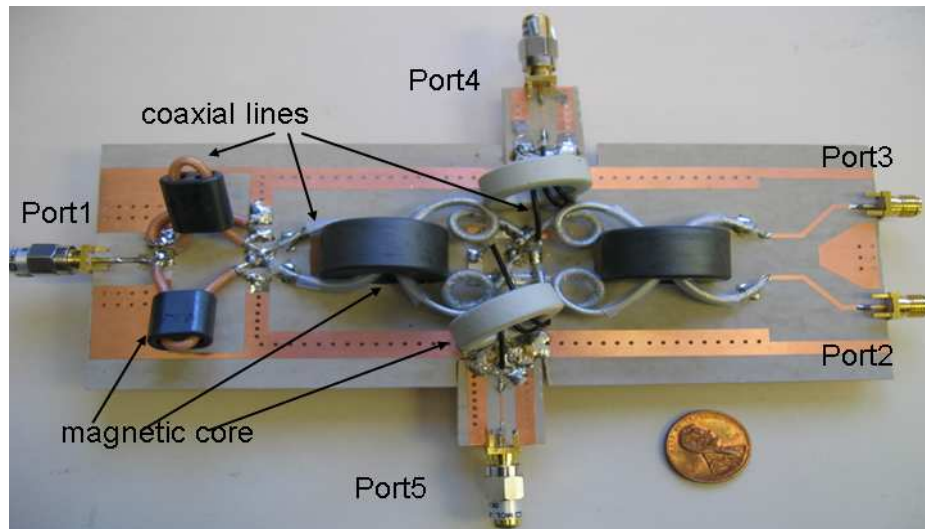
Figure 5.13 The five-port combiner, where ports 2 and 3 are the inputs, port 1 is the output, and ports 4 and 5 are the outputs used for power recycling
