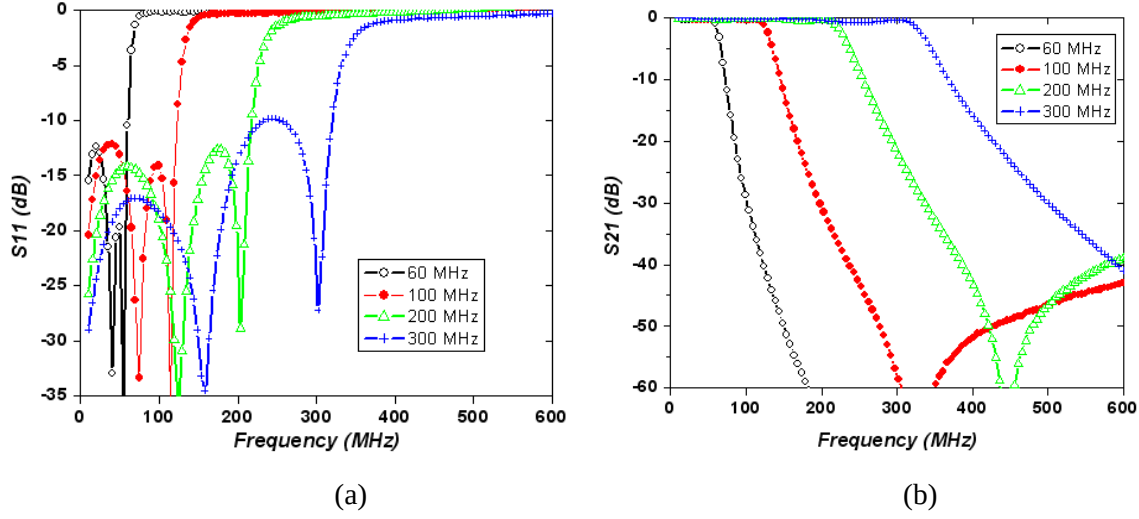
Figure 4.16 Measured results of filters: (a) S_{11} ; (b) S_{21}
