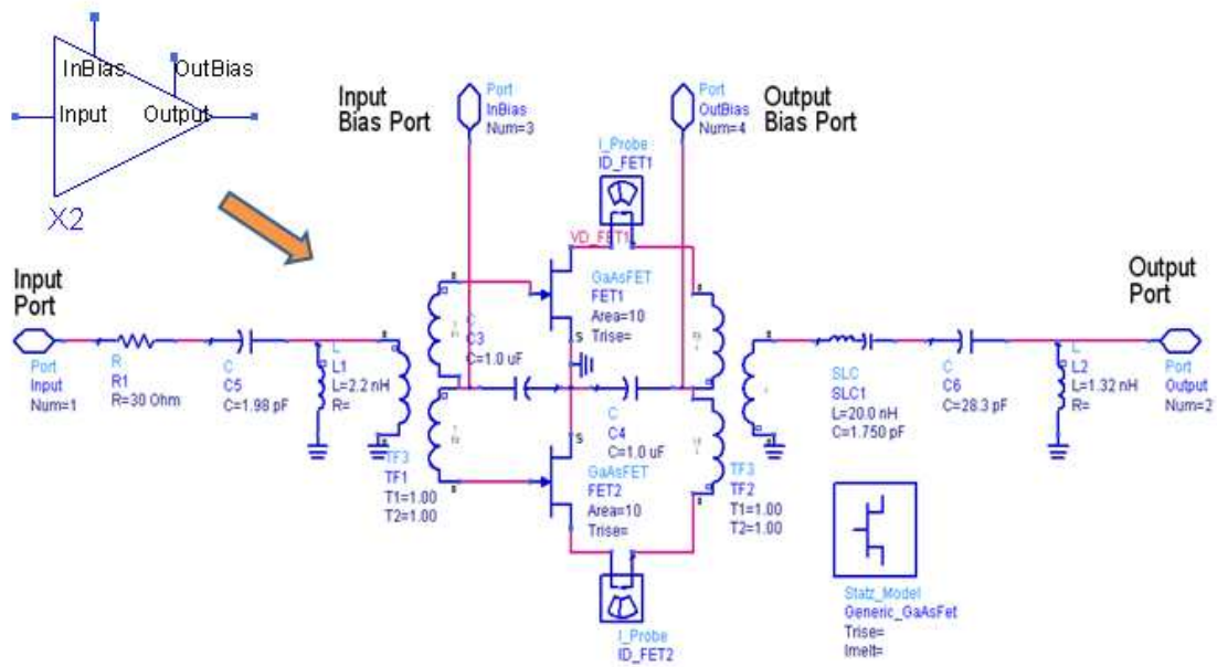
Figure C1. Narrow band class D power amplifier @ 850 MHz using GaAs FET
