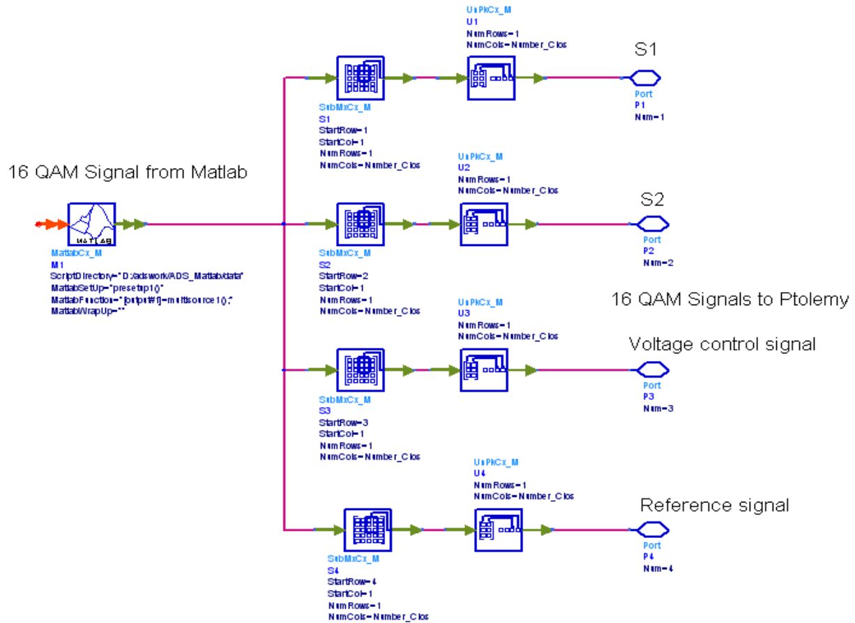
Figure D1. Sub-circuit of QAM signal generator
