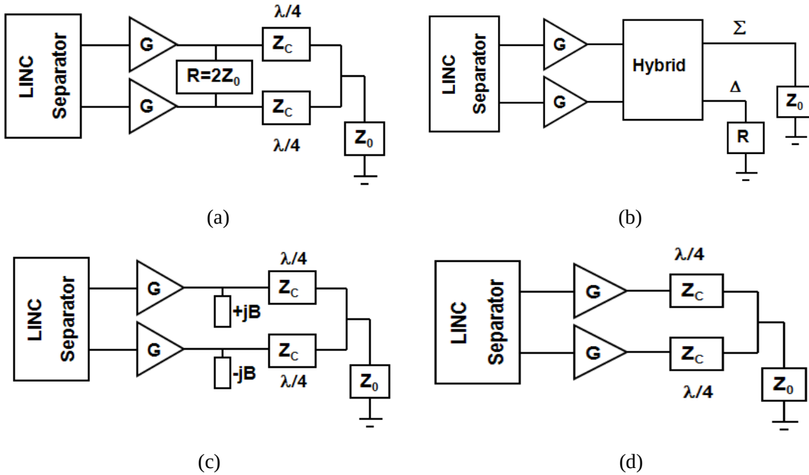
Figure 3.2 Power Combiners: (a) Wilkinson combiner; (b) Hybrid combiner; (c) Chiréix combiner; (d) Conventional non-isolated combiner (modified Chiréix).
