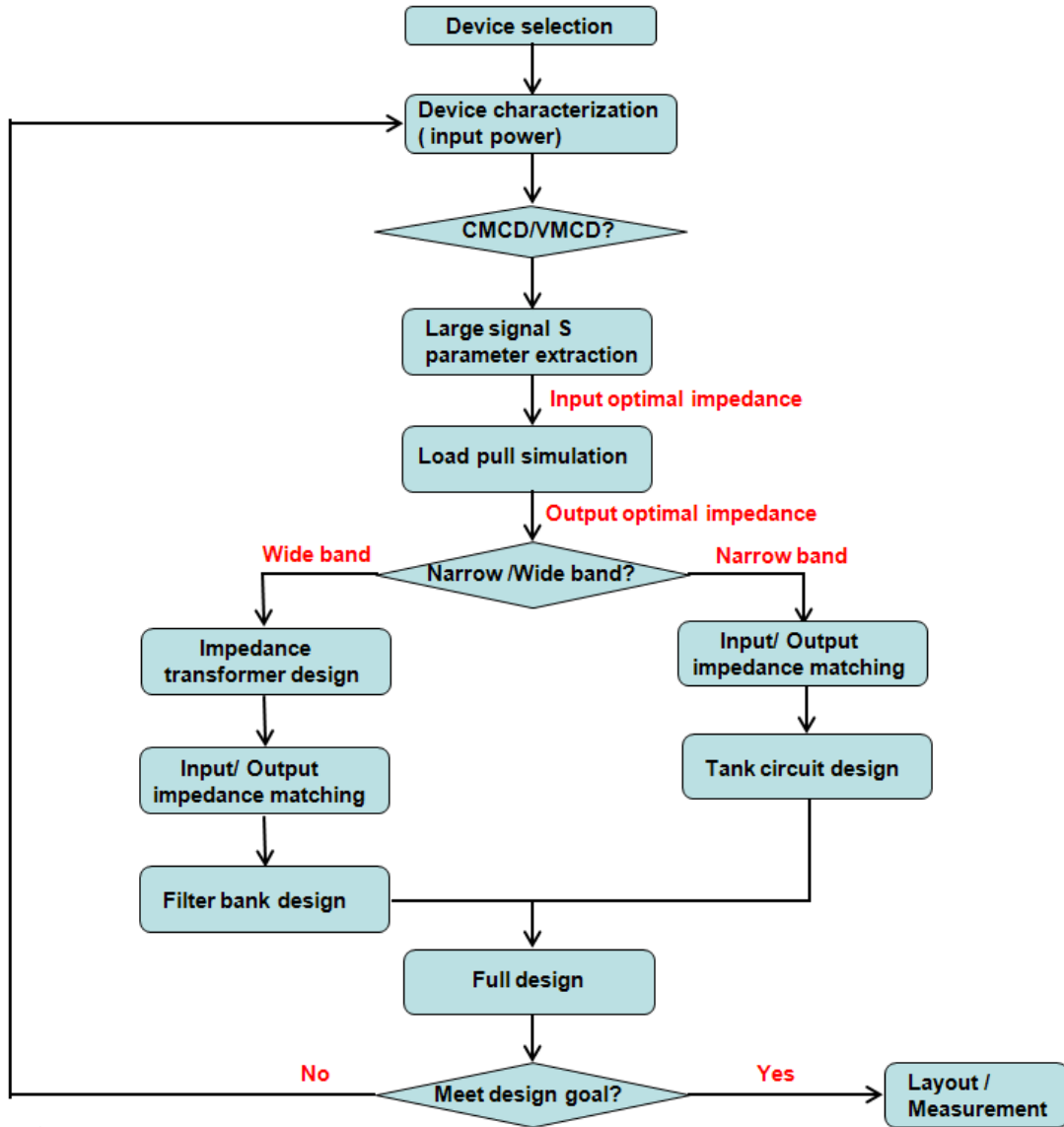
Figure 4.4 Class D PA design flow
