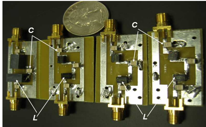
Figure 4.15 Fabricated filters (60MHz/100MHz/200MHz/300MHz)
