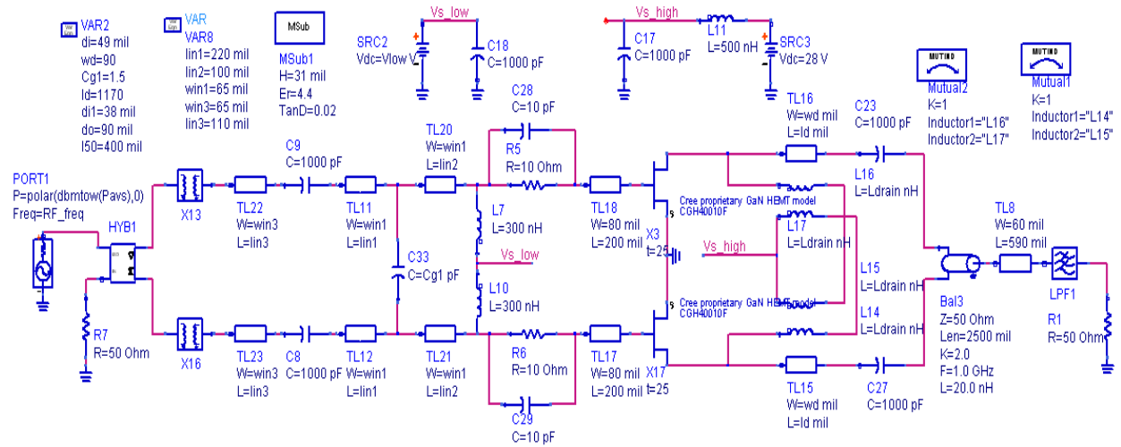
Figure C8. Wide band class D power amplifier (50 to 550 MHz) Cree GaN HEMT (CGH40010F)
