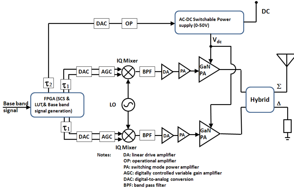
Figure 6.18 Adaptive bias LINC transmitter
