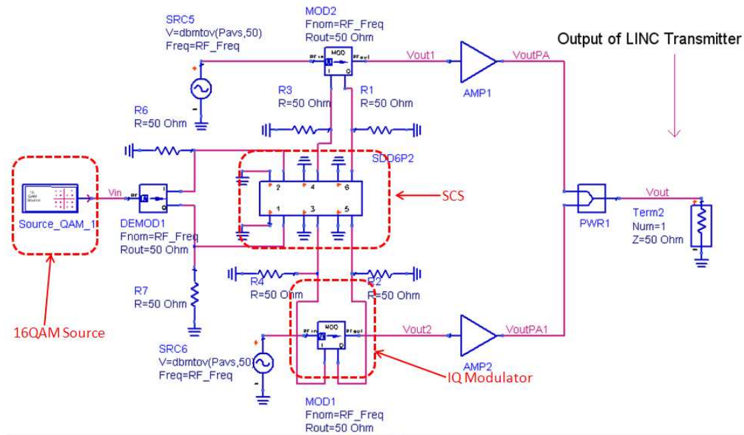
Figure 3.5 LINC transmitter with a 16 QAM signal [50]
