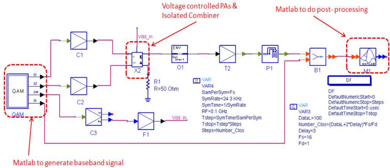
Figure 6.13 Simulation schematic for 16QAM signal with ideal voltage controlled amplifier (Note: The details of sub-circuits are shown in Appendix D.)
