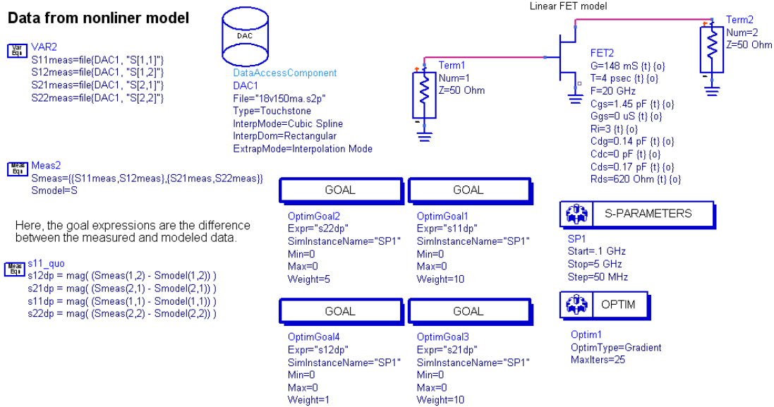
Figure 2.11 Schematic to optimize the component values for wideband operation
