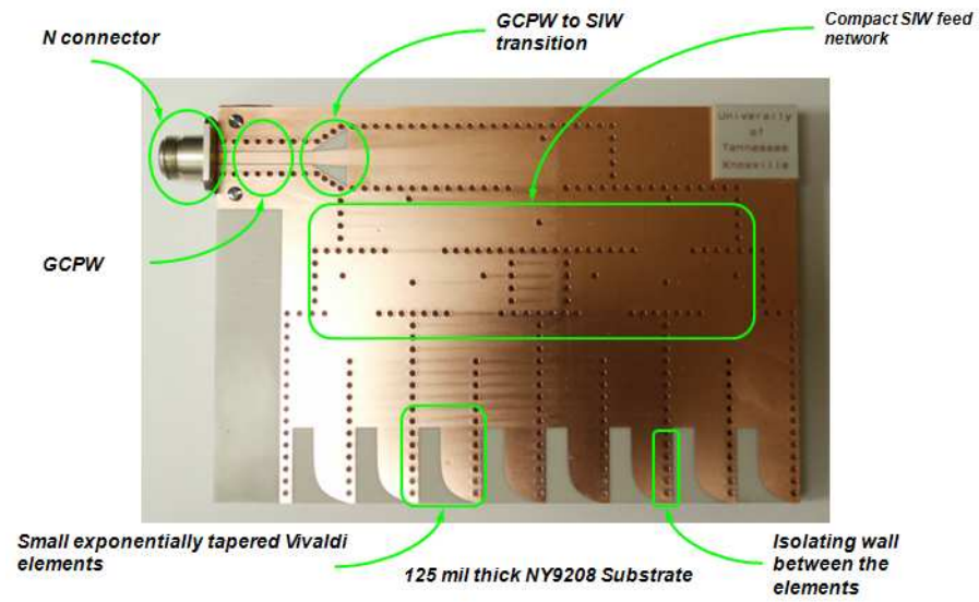
Figure 7.9 Eight elements Vivaldi array
