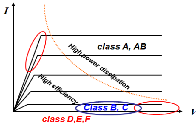
Figure 2.1 Operation regions for different power amplifiers' classes
