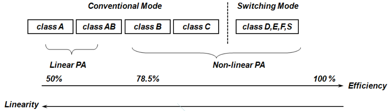
Figure 2.2 Power amplifiers' classes [3]
