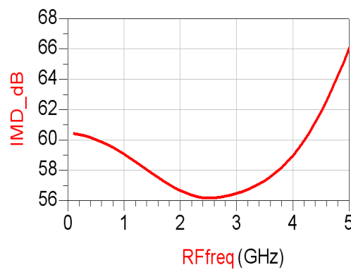
Figure 2.18 Simulated IMD with P_{in}=0 dBm
