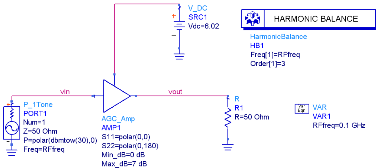
Figure C6. Test figure for voltage controlled amplifier
