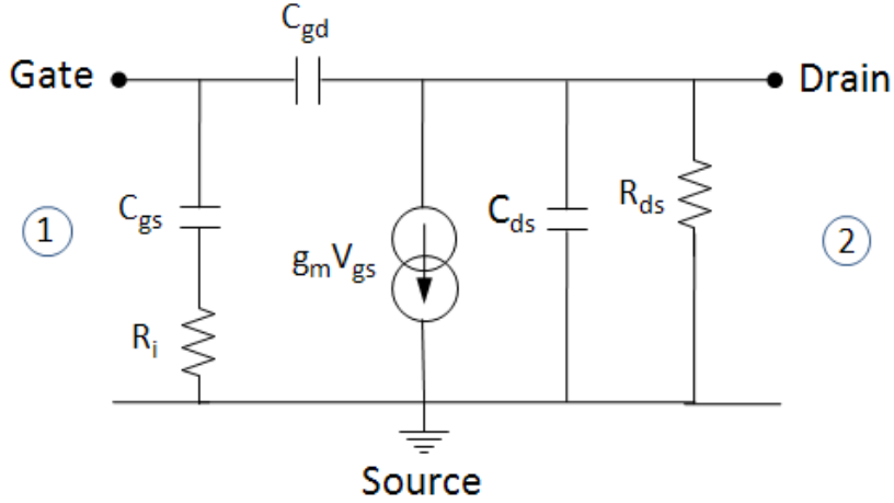
Figure A1. 7-element small signal FET model [1]
