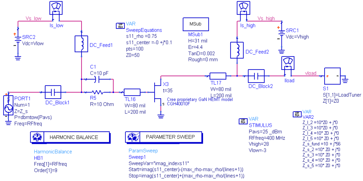
Figure 4.11 Load-pull simulation schematic
