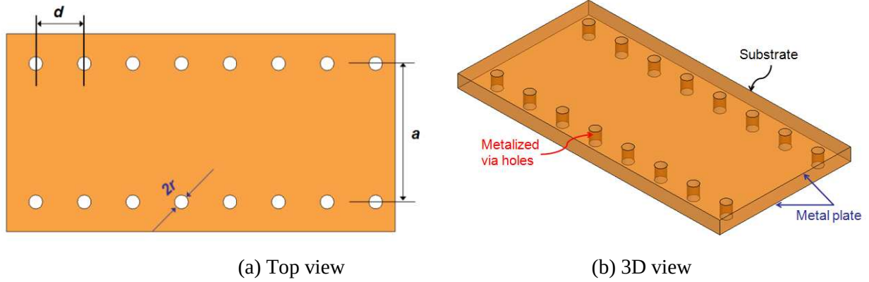
Figure 7.1 Substrate integrated waveguide on dielectric substrates
