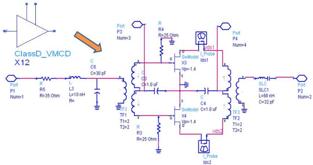
Figure C5. Narrow band Class D power amplifier @ 100 MHz using Eudyna GaN HEMT (EGN045MK)
