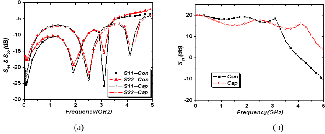
Figure 2.23 Small signal simulation results of conventional (Con) and capacitively coupled (Cap) DPAs: (a) S_{11} and S_{22} ; (b) S_{21}
