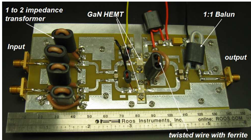
Figure 4.18 Fabricated VMCD PA
