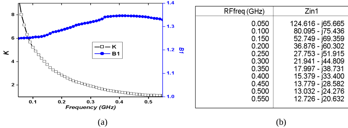
Figure 4.10 Large signal stability performance: (a) Stability factors and measure; (b) Input impedance
