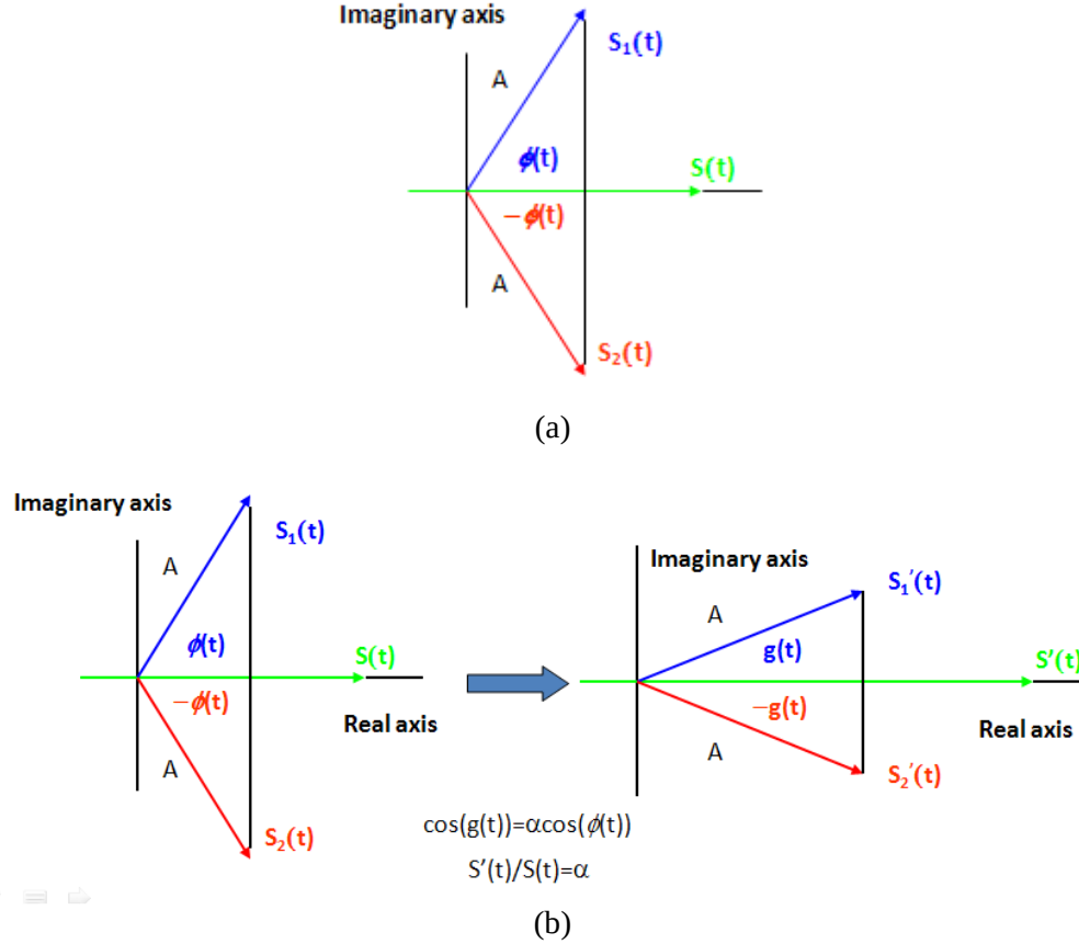
Figure 6.8 Signal decomposition: (a) Conventional LINC; (b) Adaptive bias LINC
