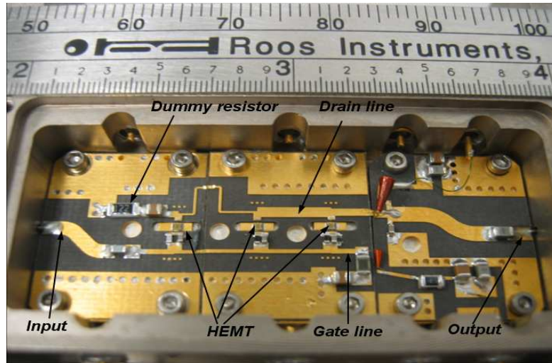
Figure 2.28 Implemented hybrid DPA
