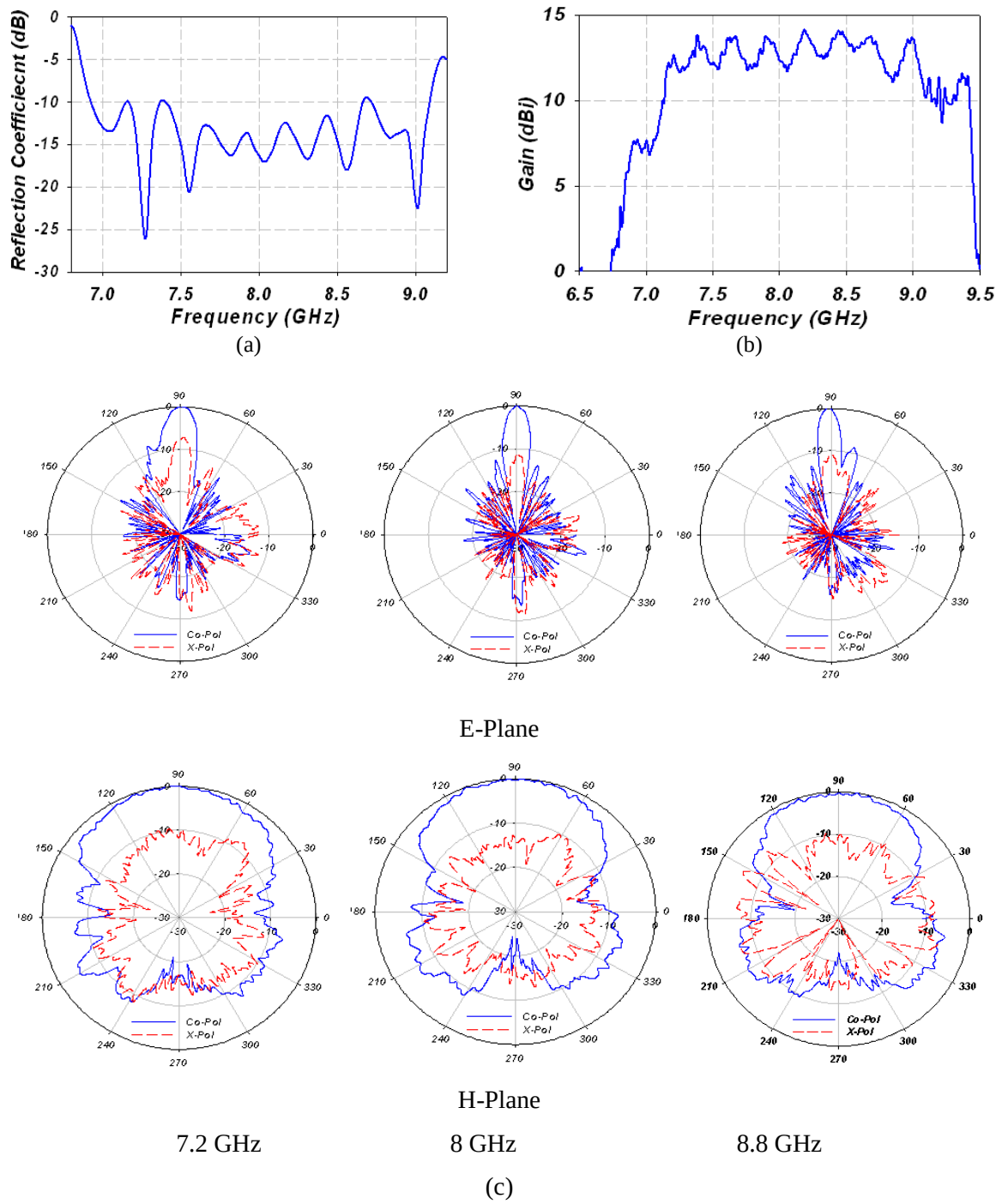
Figure 7.10 (a) Reflection coefficient of the array; (b) Gain vs. Frequency; (c) Radiation pattern vs. Frequency
