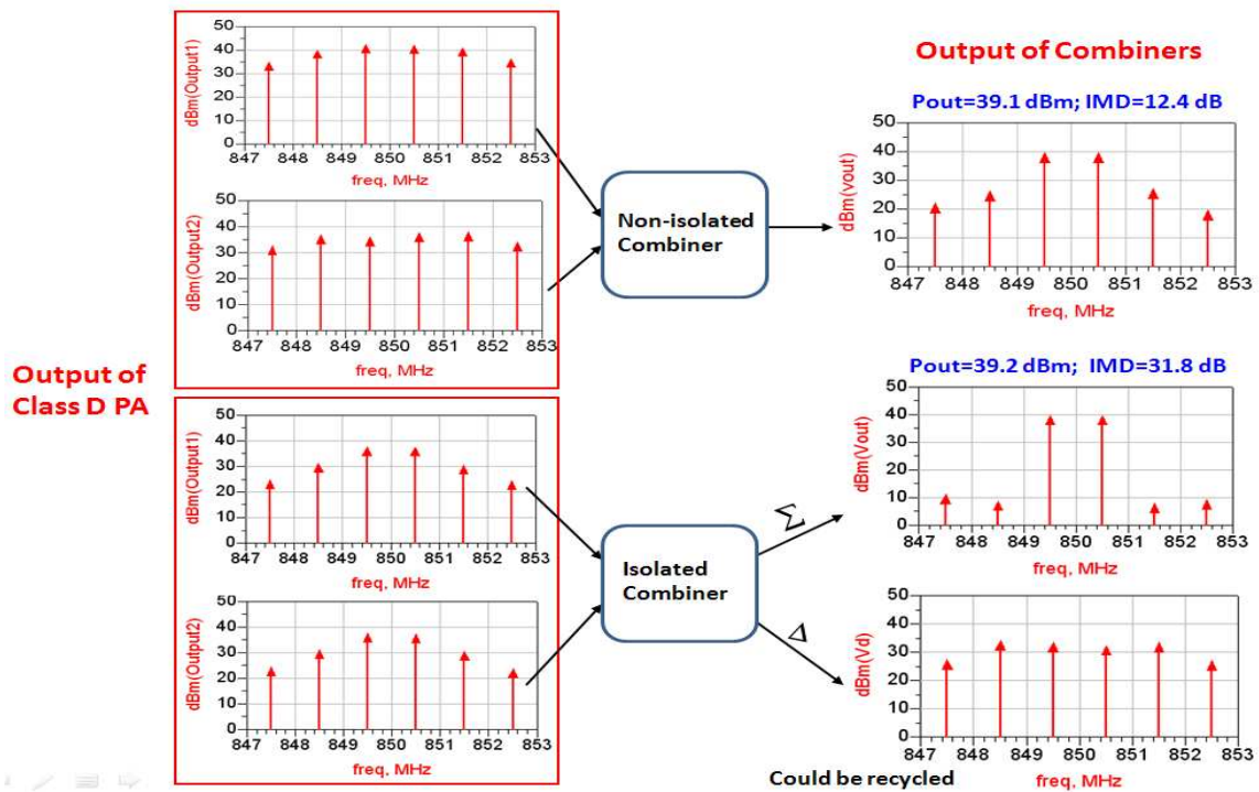
Figure 6.5 Simulation results of the LINC transmitter with two-tone signal using isolated/ non-isolated combiners
