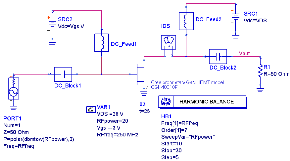
Figure 4.7 Input Power sweep schematic
