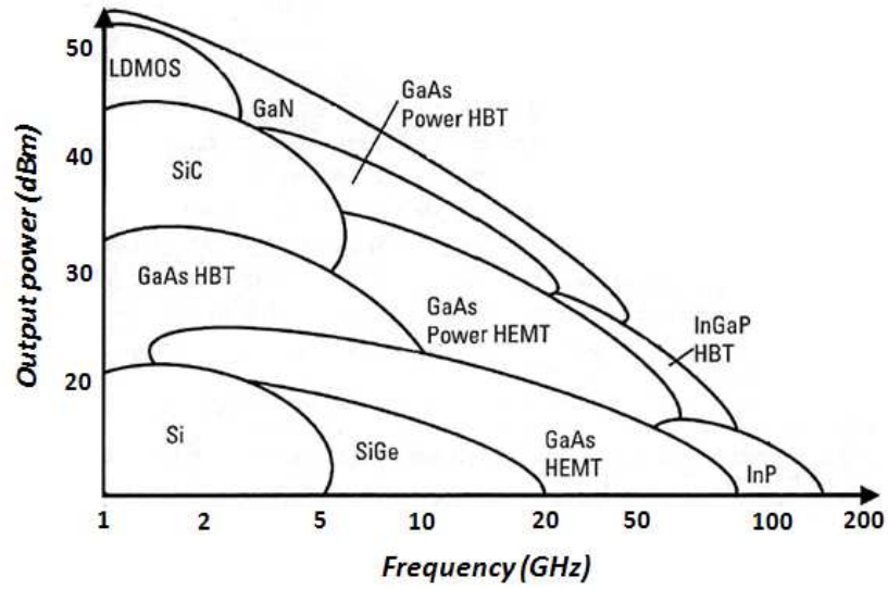
Figure 2.6 Plot of output power vs. frequency for different transistor technologies [7]
