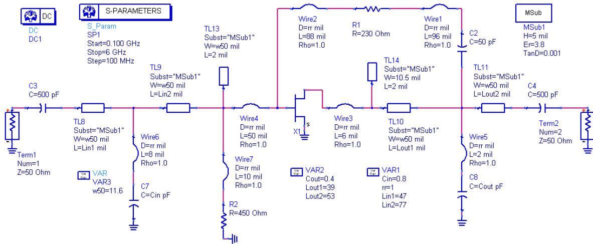
Figure 2.15 Small signal simulation schematic in ADS
