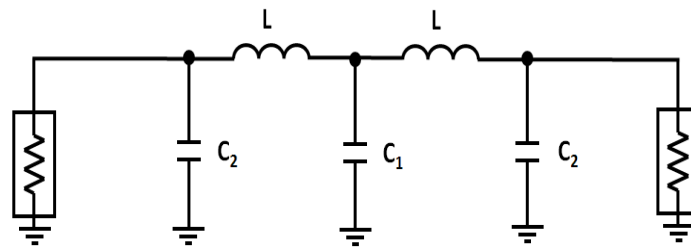
Figure 4.13 Low pass filter schematic
