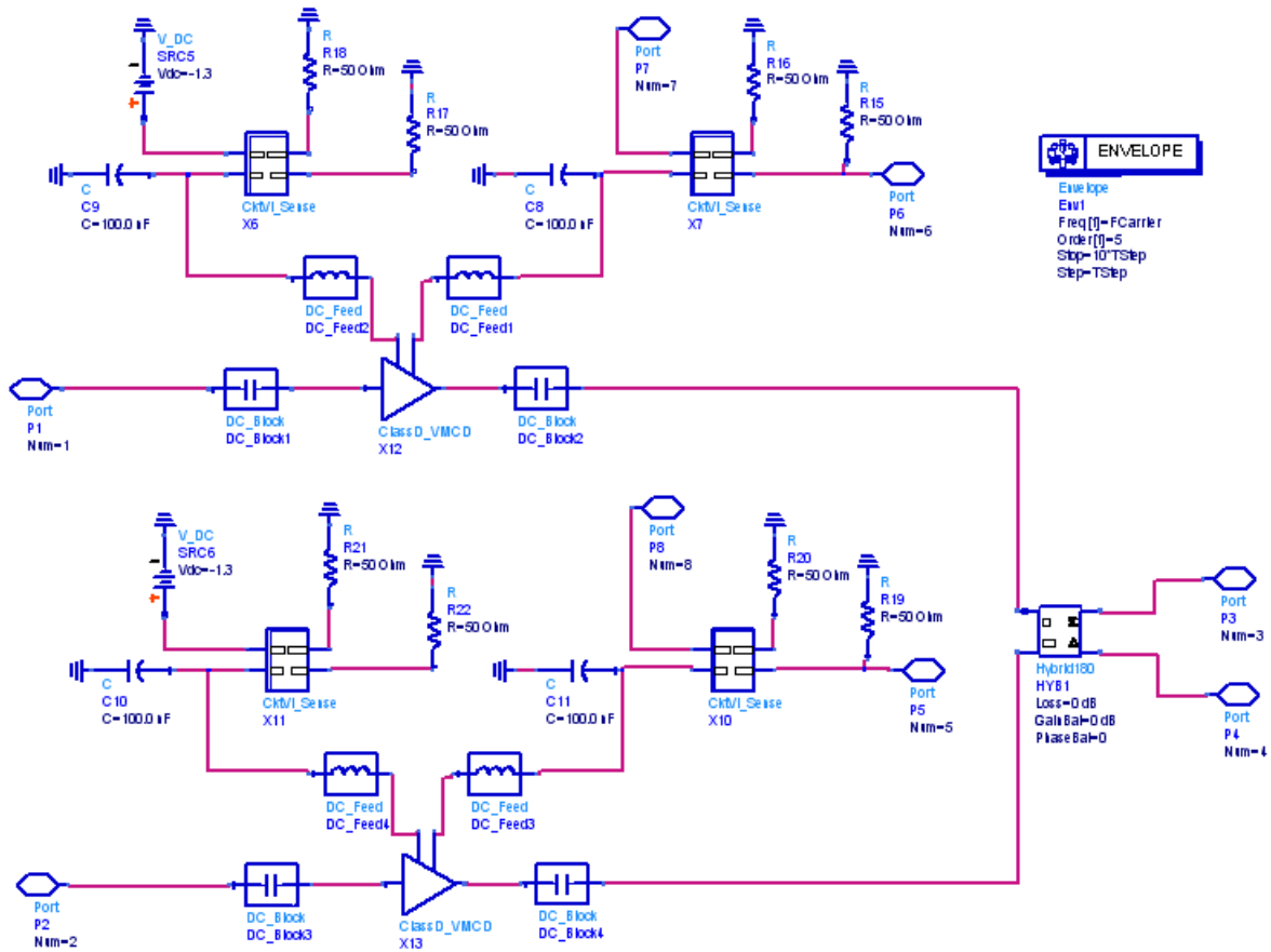
Figure D4. Sub-circuit of PA_50_T unit
