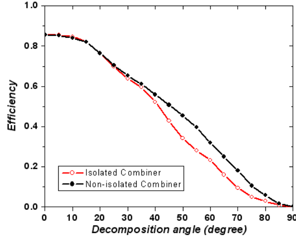
Figure 6.2 Efficiency vs. decomposition angle
