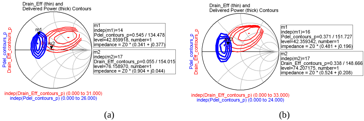
Figure 4.12 Drain efficiency and delivered power contours: (a) 200MHz; (b) 400MHz
