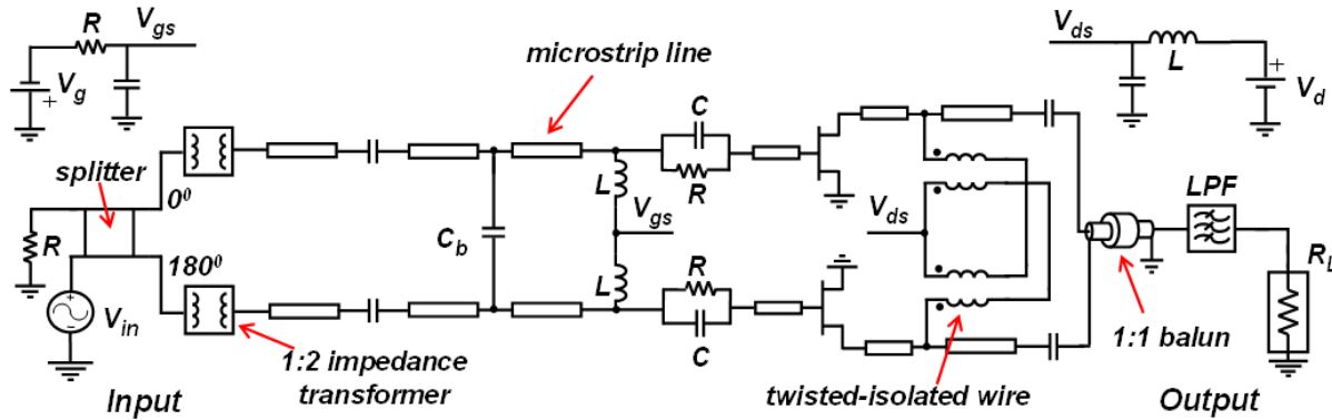
Figure 4.17 Full circuit simulation schematic
