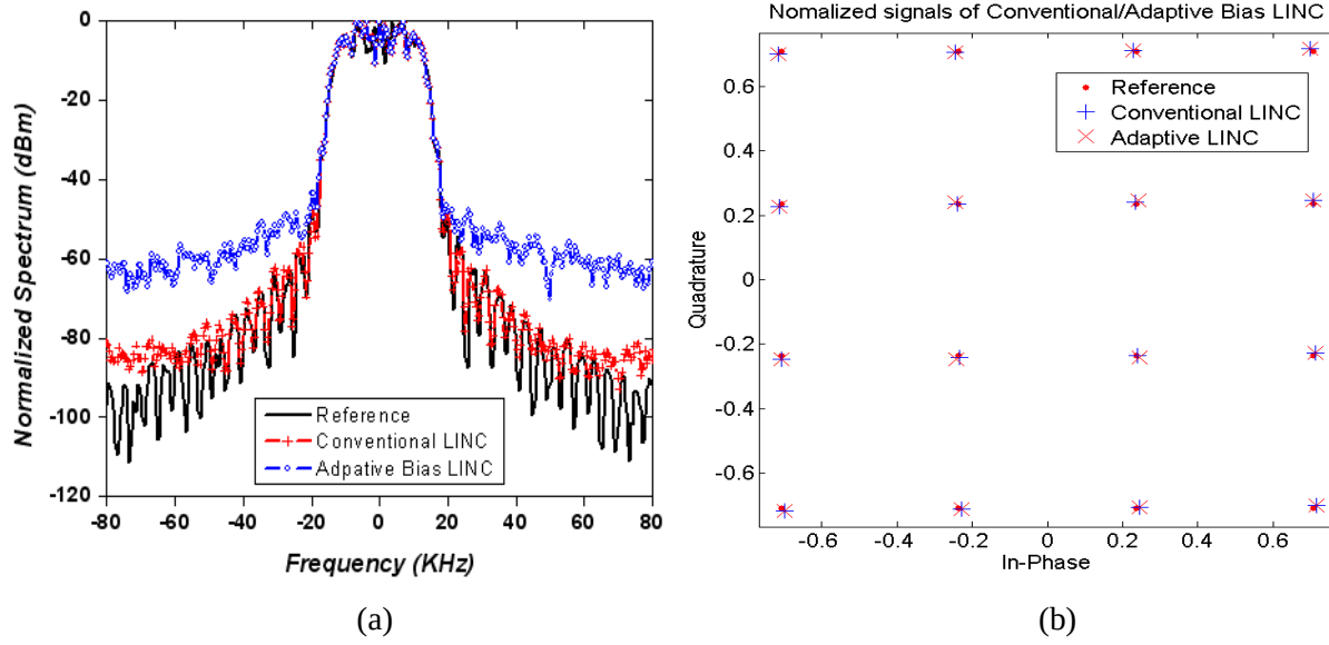
Figure 6.17 Simulation results: (a) Normalized spectrum; (b) Normalized constellation
