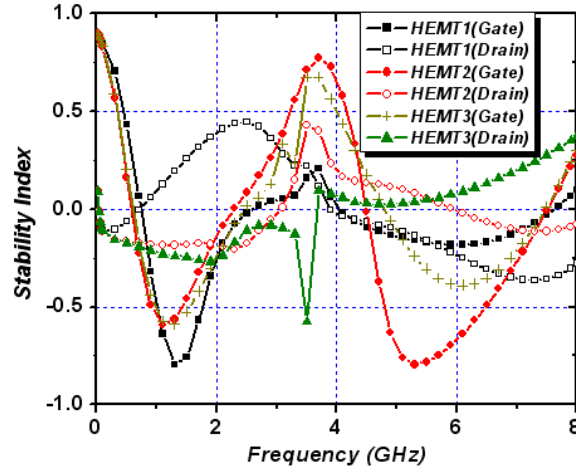
Figure 2.27 Stability indices of the optimized DPA
