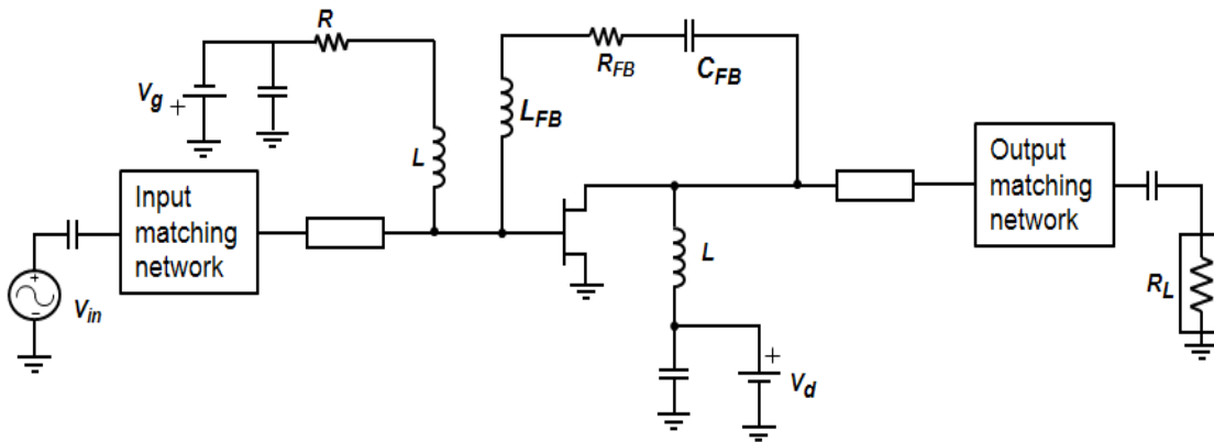
Figure 2.7 Simplified feedback amplifier
