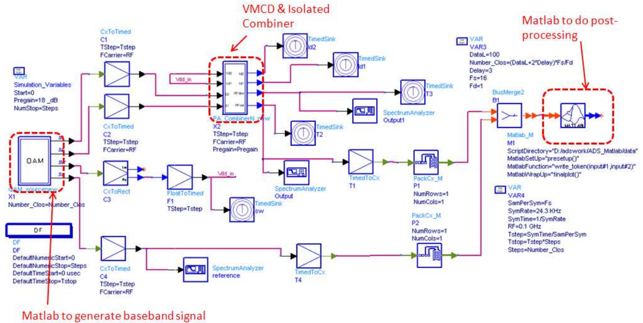
Figure 6.16 Schematic of adaptive bias LINC transmitter with GaN VMCD
