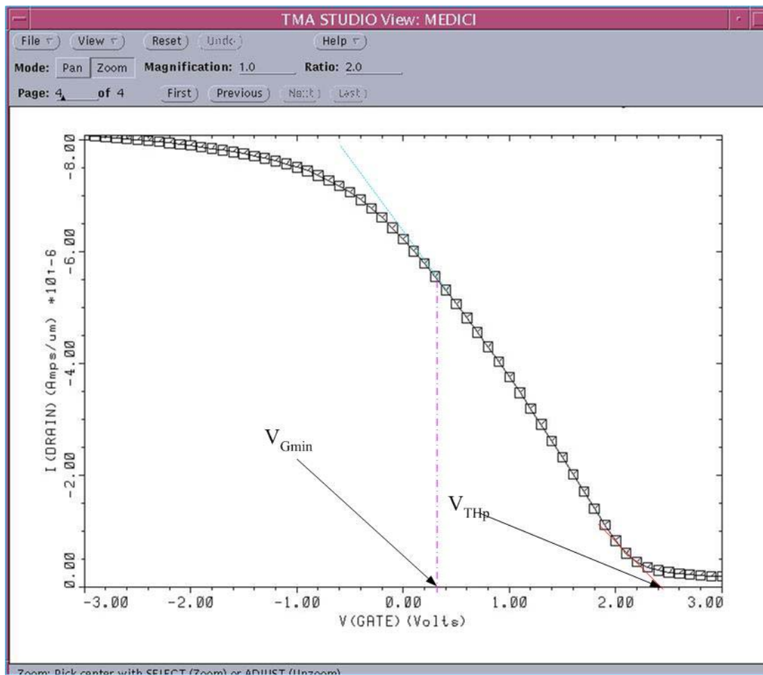
Figure 6. 1: Medici TM simulation result used to determine V_{THp} and V_{Gmin} .
