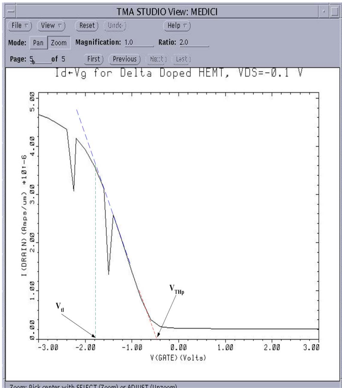
Figure 6. 6: Medici TM simulation results used to determine V_{THp} and V_d for the p-channel delta-doped SiGe MOS-gate HEMT.
