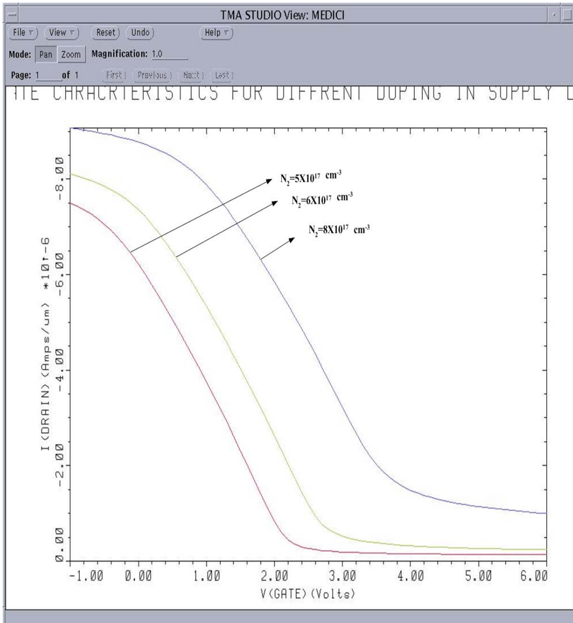
Figure 6. 3: I_{\text{D}}-V_{\text{G}} characteristics of the p-channel SiGe MOS-gate for different supply layer doping concentrations.
