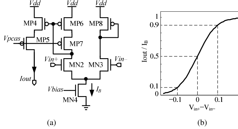
Figure 2-5: (a) Schematic of the transconductor and (b) its transfer function.
