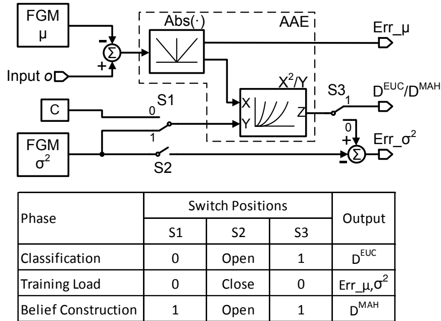
Figure 4-6: The schematic of the reconfigurable analog computation cell and the switch positions for three operation modes.
