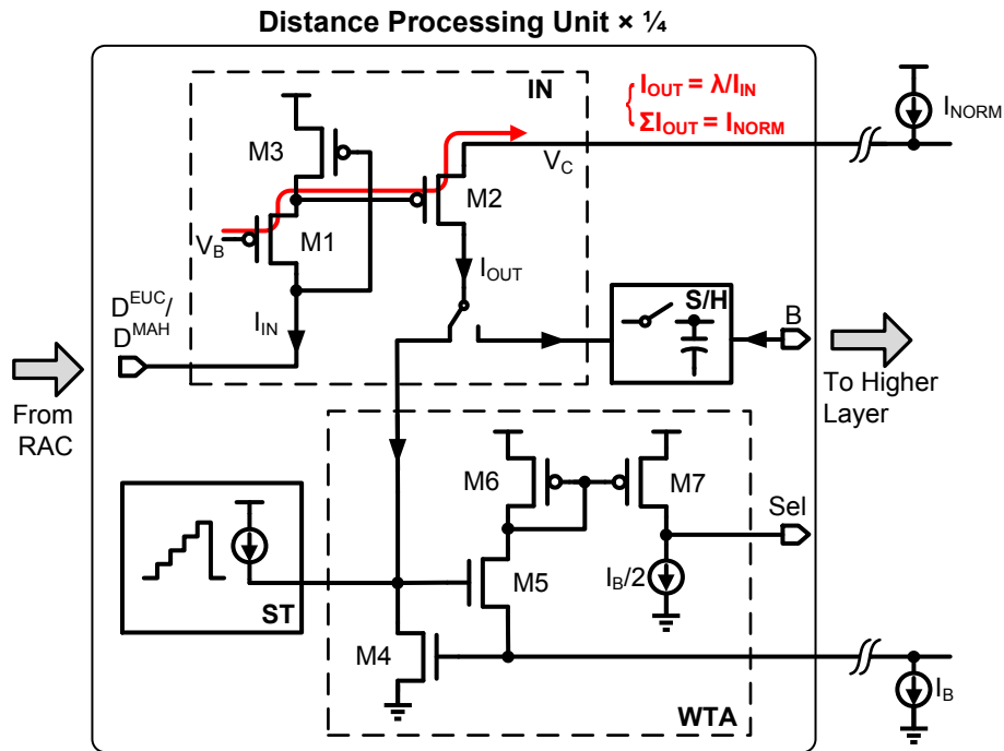
Figure 4-9: The schematic of one channel of the distance processing unit.
