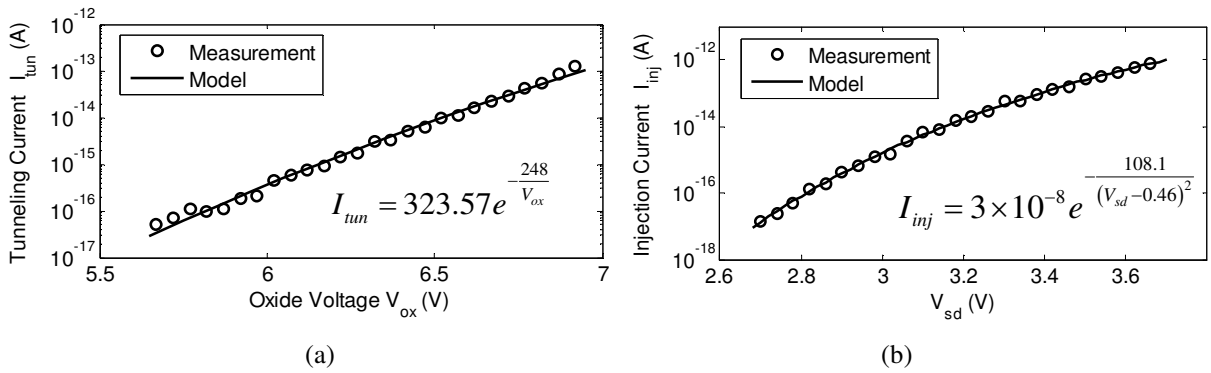
Figure 2-6: (a) Tunneling current versus oxide voltage V_{ox} . (b) Injection current versus drain-to-source voltage of the injection transistor.
