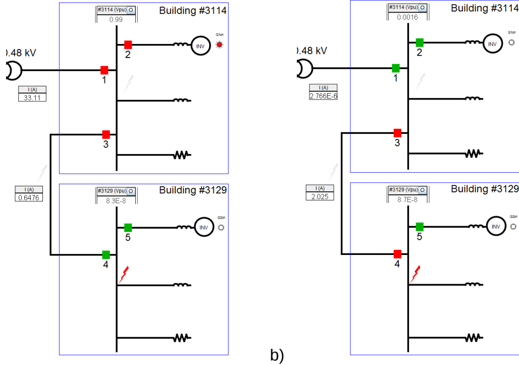
Figure 4.3 a) Fault in building #3129 while on grid. b) Fault in building #3129 while off grid.
