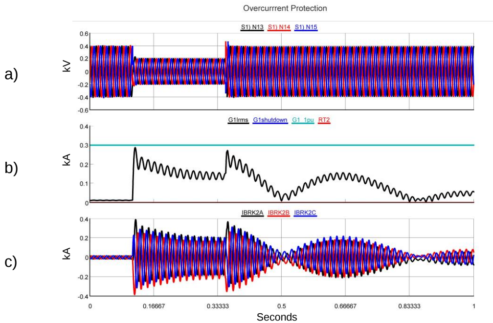
Figure 4.4 a) Building #3114 bus voltages during fault in building #3129 while on grid. b) Building #3114 inverter rms current output during fault. c) Building #3114 inverter current passing through circuit breaker 2.
