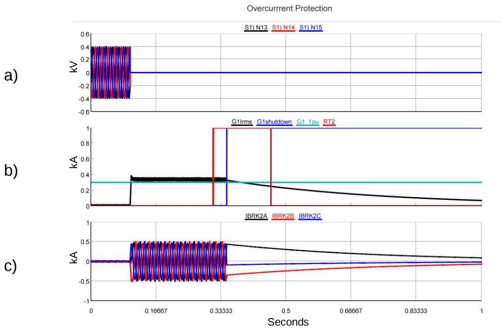
Figure 4.2 a) Building #3114 bus voltages during fault in building #3114 while on grid. b) Building #3114 inverter rms current output during fault. c) Inverter current passing through circuit breaker 2 during fault.
