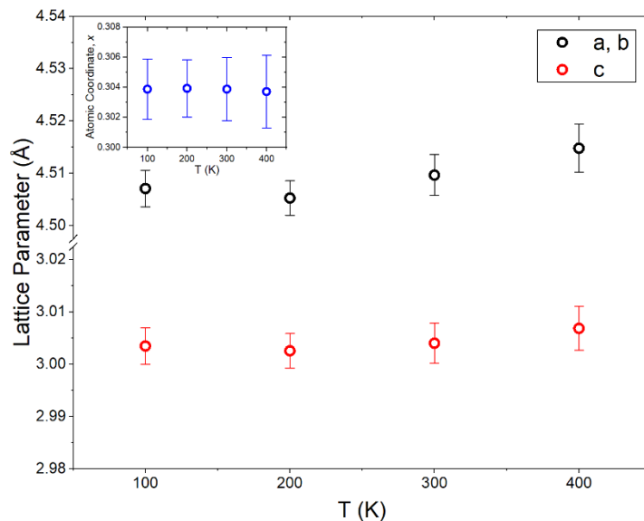
Figure 43: Temperature dependence of the lattice parameters for \text{MgD}_2 from total neutron scattering measurements. The atomic coordinates relating to the x-coordinate for the deuterium sites is shown in the inset.
