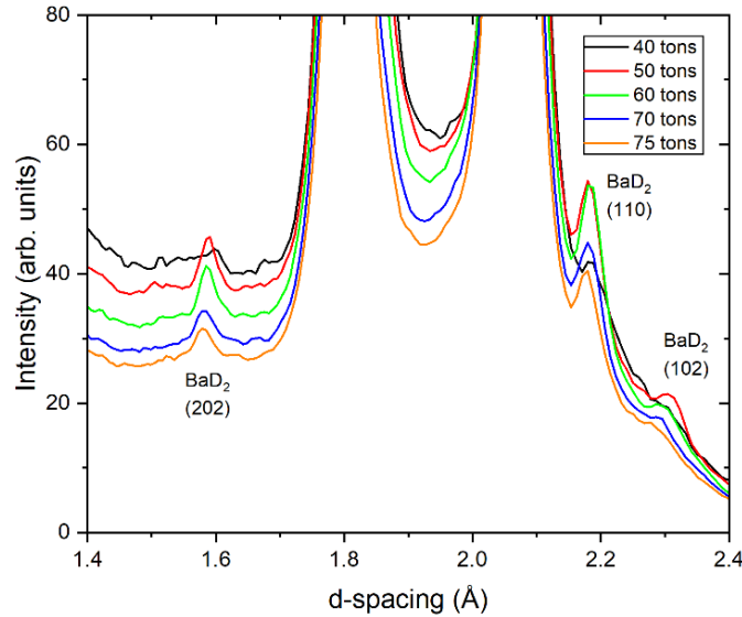
Figure 15: SNAP diffraction pattern summed over the center column of the high angle detector bank ( \sim 97^\circ - 113^\circ ) for \text{BaD}_2 in a CuBe gasket.
