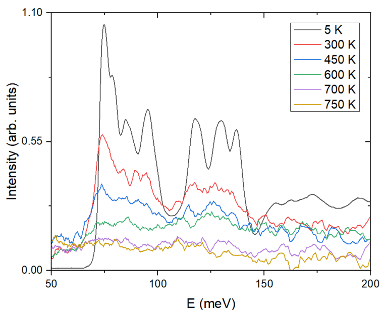
Figure 40: INS spectra from 5 K to 750 K for \text{CaH}_2 measured at VISION. Intensities are translated for clarity.
