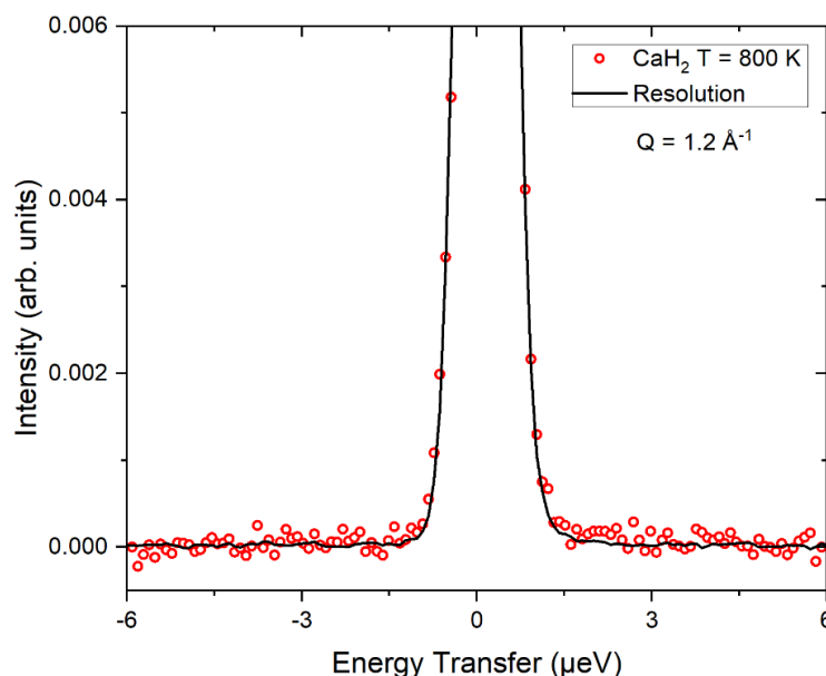
Figure 39: QENS spectra and resolution function measured at HFBS for \text{CaH}_2 at T = 800 K and Q = 1.2 \text{ \AA}^{-1} .
