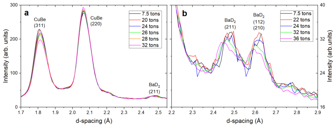
Figure 14: SNAP diffraction pattern summed over the high-angle column of the low angle detector bank ( \sim 59^\circ - 74^\circ ) for BaD 2 in a CuBe gasket.
