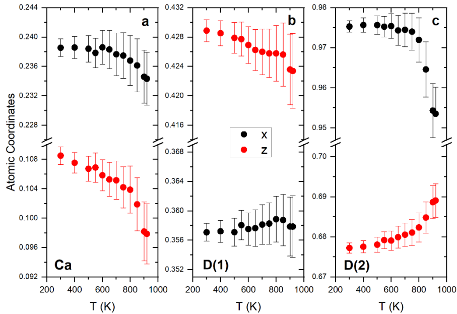
Figure 37: Atomic coordinates x and z for the (a) Ca, (b) D(1), and (c) D(2) sites for \text{CaD}_2 .
