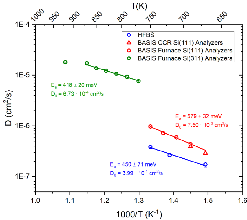
Figure 26: Arrhenius diagram for BaH 2 with diffusion coefficients calculated from QENS. Solid lines are a linear fit of the data. Activation energies and preexponential diffusion coefficients are reported.
