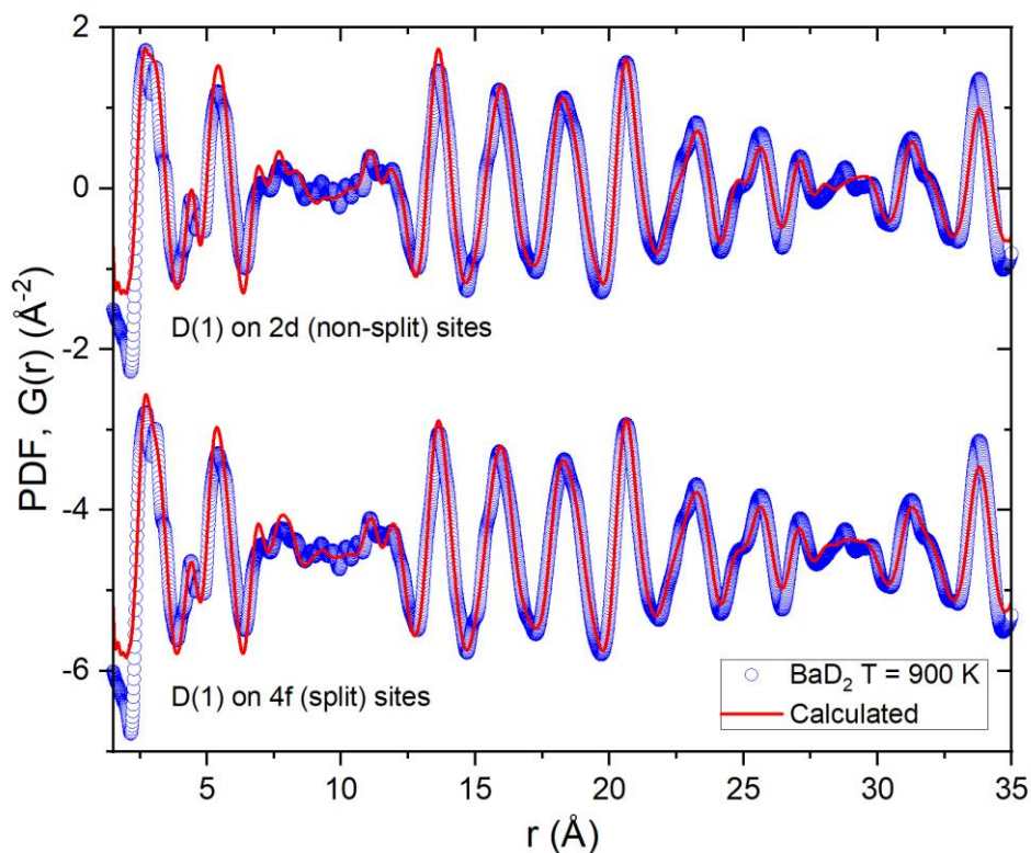
Figure 23: Comparison of G(r) for \text{BaD}_2 at 900 \text{ K} fit with models containing D(1) positioned on 2d (non-split) sites and 4f (split) sites. G(r) are translated for clarity.
