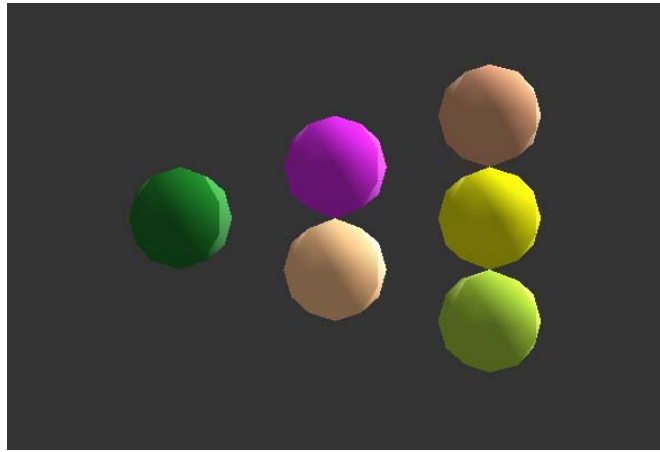
Figure 4.10 DEM Clumps technique
