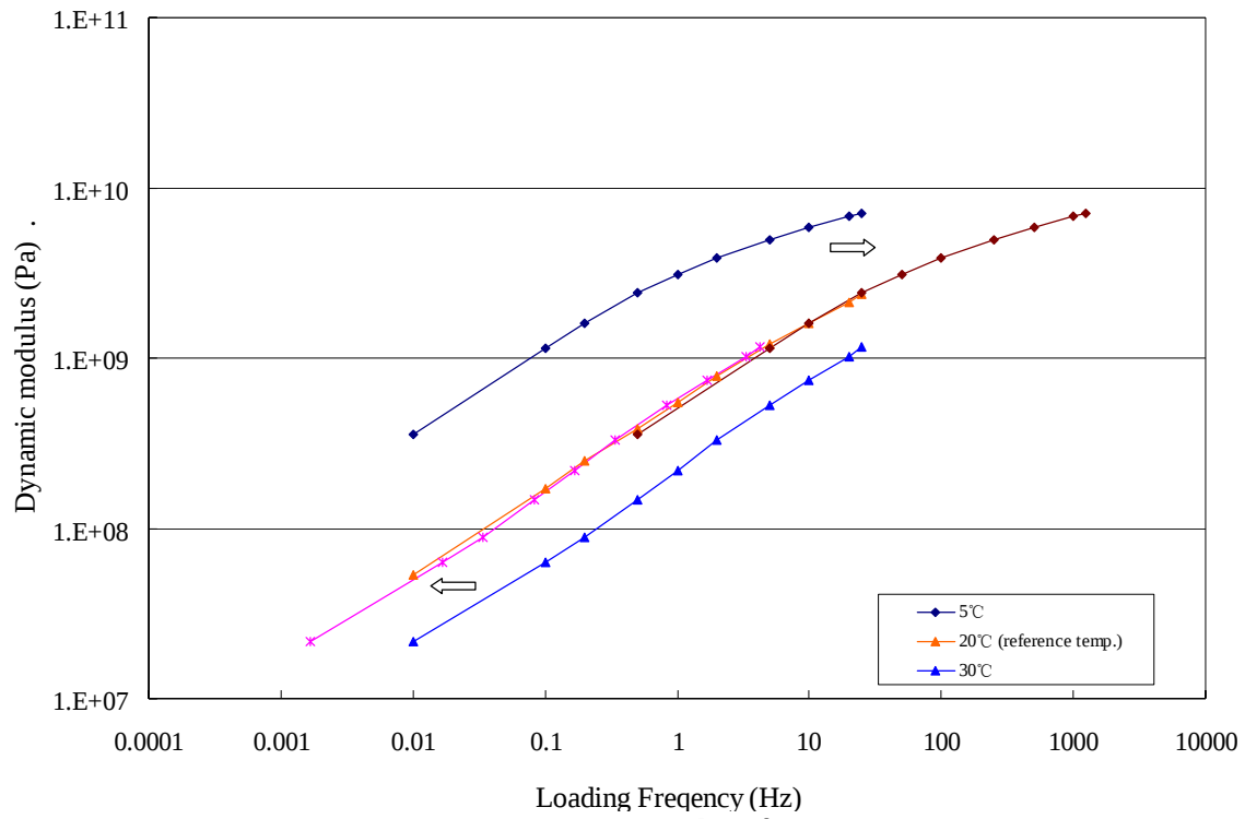
Figure 3.6 Dynamic test results of SMA mastic
