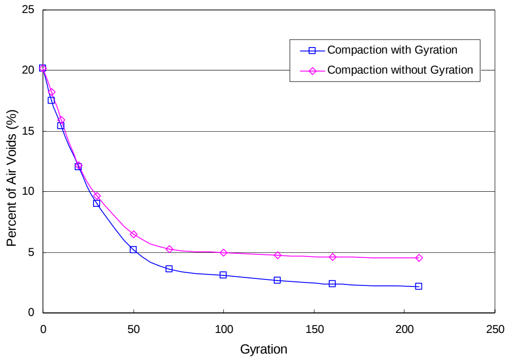
Figure 4.15 Compaction with and without Gyration
