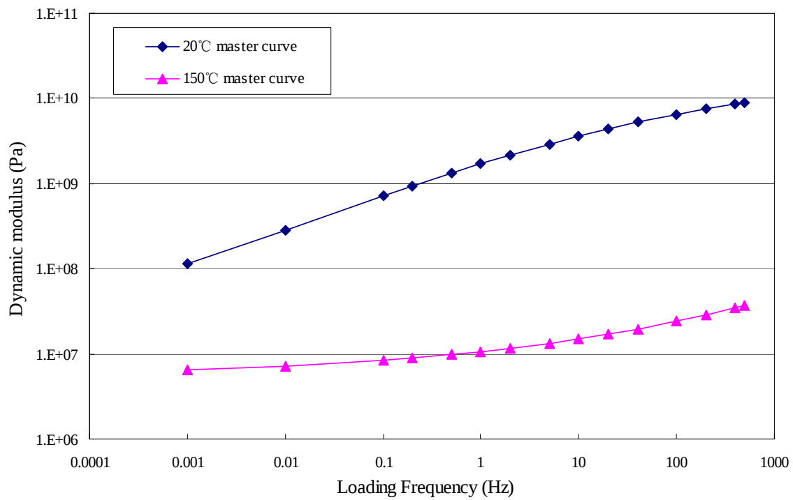
Figure 3.7 Master Curve of Superpave mastic
