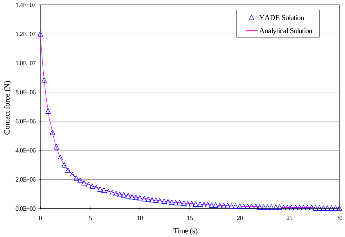
Figure 2.8 Comparison between Analytical and YADE Solution
