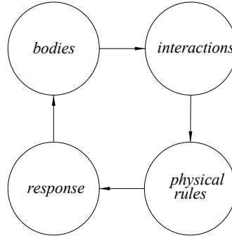
Figure 1.1 Schematics of Simulation Loop (Kozicki and Donze, 2008)
