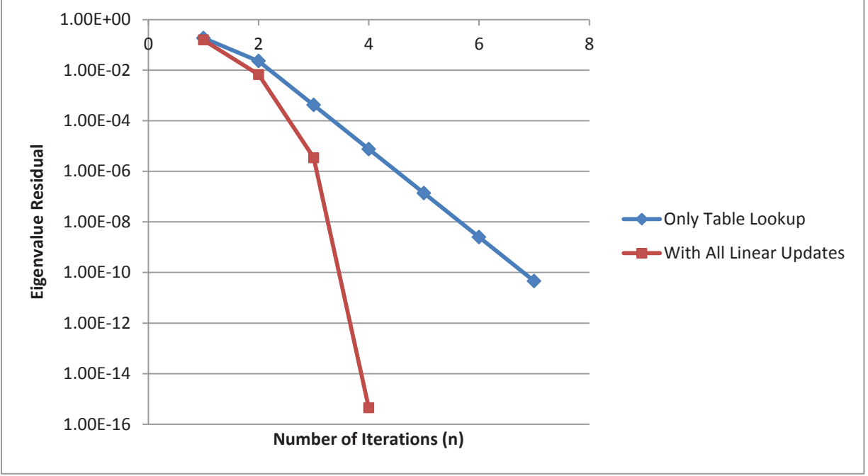
Figure 5. Convergence of a table lookup (Algorithm 6) vs the addition of a linear update
