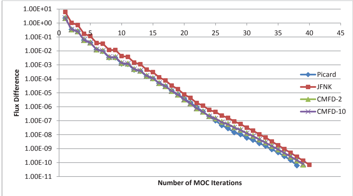
Figure 12. Convergence of the 2-norm of the flux difference for the 1D, one-group homogenous slab problem
