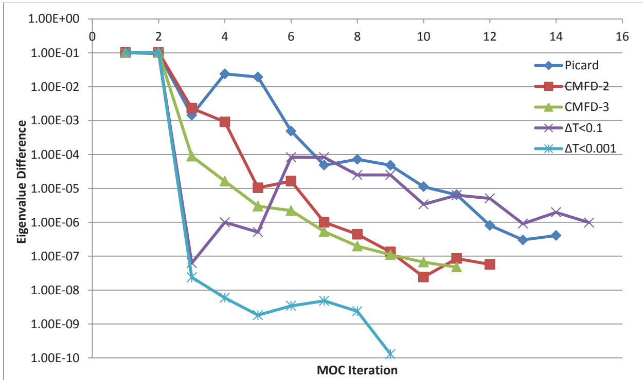
Figure 30. Comparison of the eigenvalue differences for each CMFD-Coupling implementation applied to the 3D full core problem with critical boron search enabled
