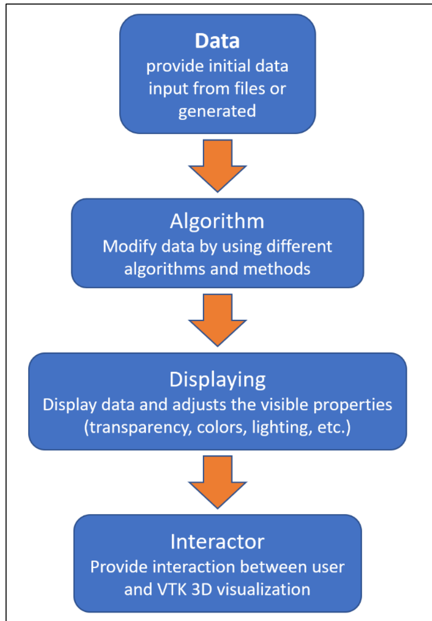
Figure 2-8: VTK pipeline.
