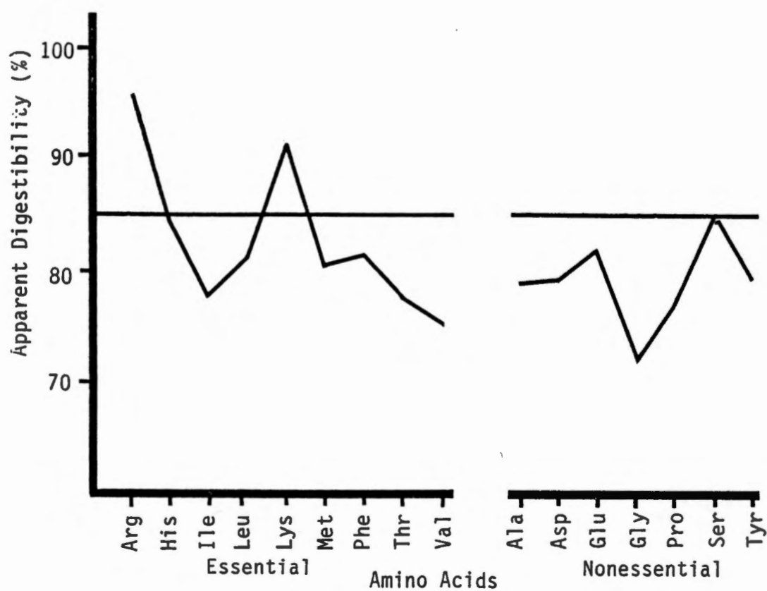
FIGURE 5. Comparison of ADCP and AAAAA values for soybean meal (DM basis).
