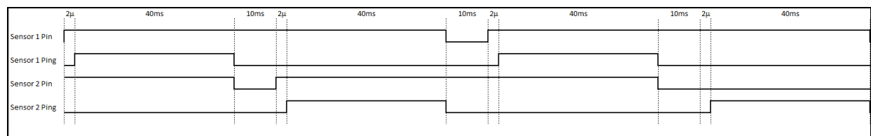
Figure 11. Timing diagram for sensors
