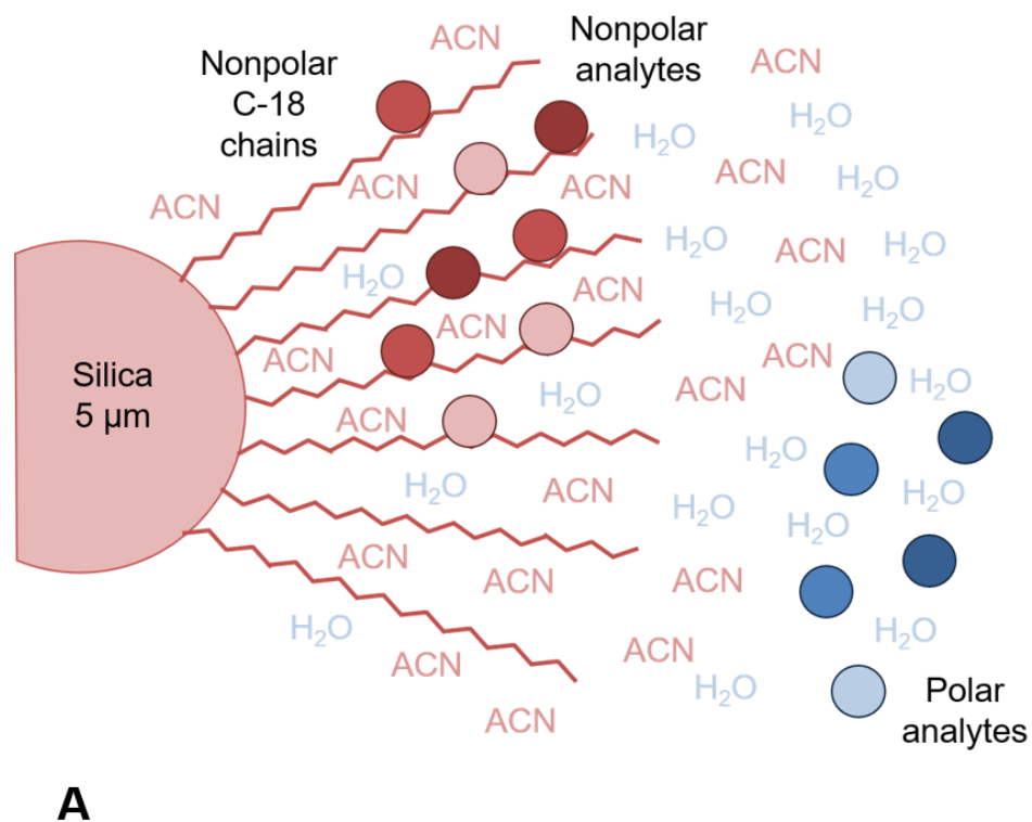
Figure 8: Schematic of (A) a C-18 RP silica bead and (B) a ZIC-pHILIC polymer bead showing the complimentary retention mechanisms where nonpolar analytes are absorbed to the C-18 chain and both polar and nonpolar analytes are partitioned into an aqueous layer formed on the surface of the zwitterionic chain.
