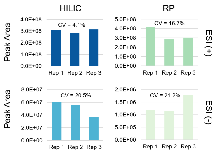
Figure 19: Integrated XIC peak areas for internal standards spiked into and extracted from triplicate soil samples (10 \mu M), prior to alignment or normalization procedures
