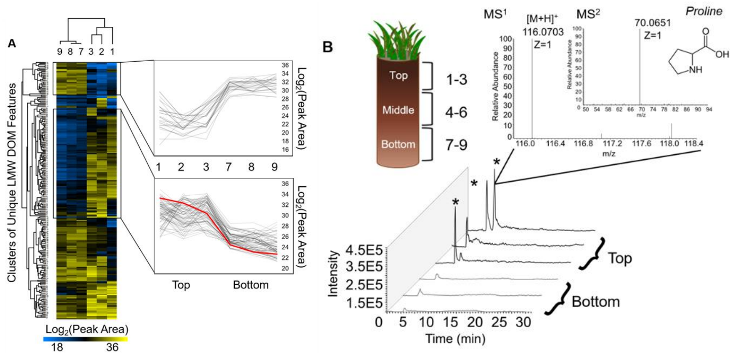
Figure 25: (a) Heatmap, or two-way hierarchically-clustered dendrogram of unique IDs and normalized \text{log}_2 peak areas for each differentially-abundant HQF detected by HILIC (+) with two clusters of differentially-abundant features called out (inset) (b) Cross-sectional diagram of the soil core with sample IDs and stacked XICs for feature highlighted in red in 25a, \text{MS}^1 , and \text{MS}^2 spectra (insets) for a feature (116.0703 m/z ) detected reproducibly by HILIC (+) at RT 6.1 min
