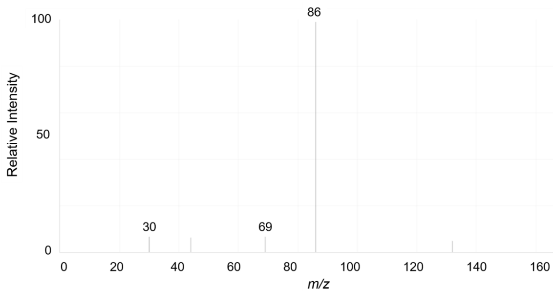
Figure 66: Corresponding database MS 2 spectrum for matched standard, alloseleucine
