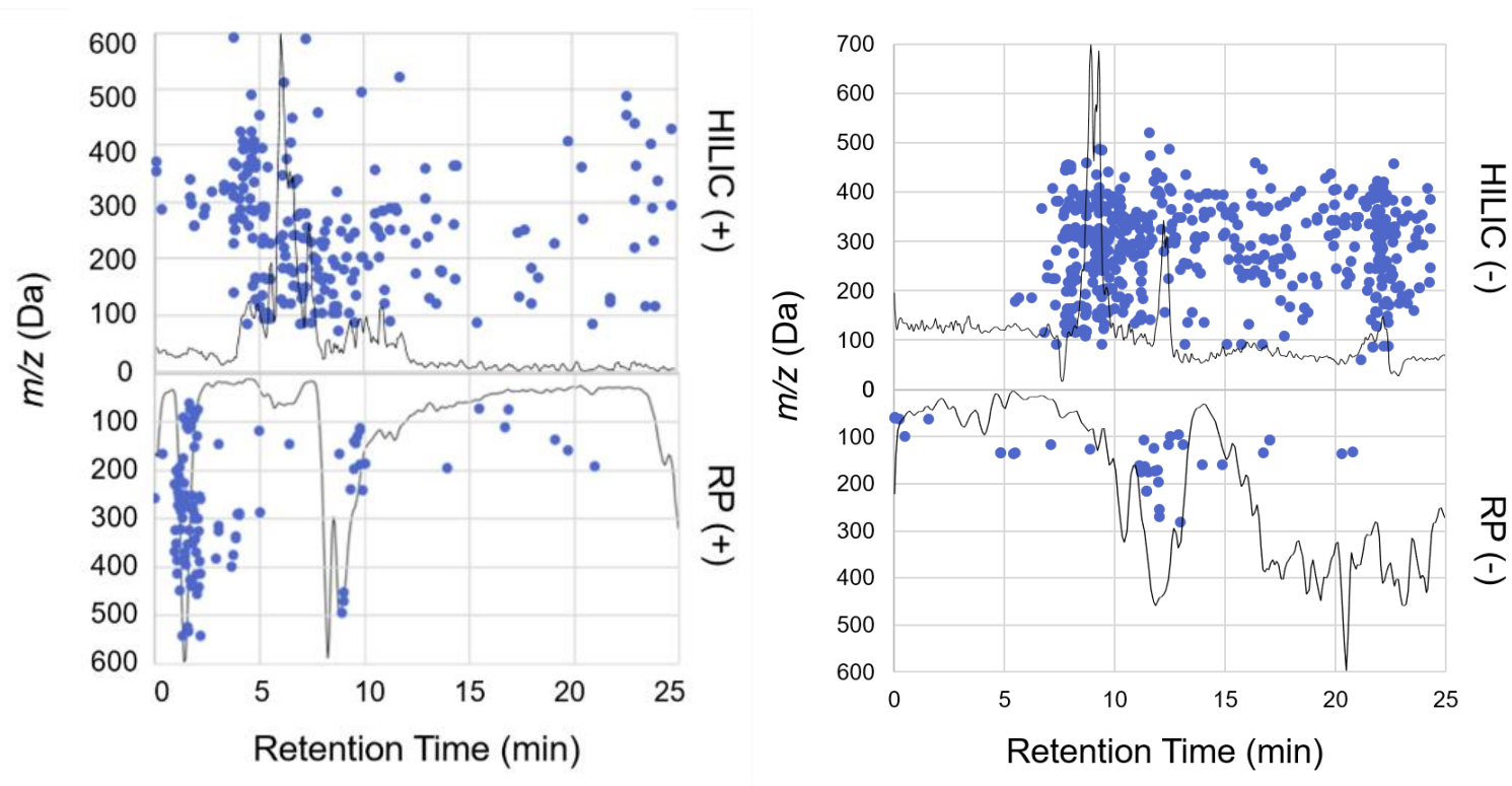
Figure 15: Scatter plots of features detected (intensity > 1.0E4, \pm 0.005 m/z ) in a single soil water extract and the elution profiles for HILIC (top) and RP (mirrored bottom) in positive-ion mode (left) and negative-ion mode (right)
