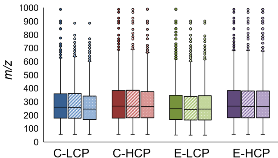
Figure 40: Distribution of m/z 's of differentially-abundant HQFs by core and depth From left to right, solid color indicates “top”, stripes indicate “middle”, and dots indicate “bottom” of the organic horizon; blue = Carex LCP, red = Carex HCP, green = Erioph LCP, and purple = Erioph HCP
