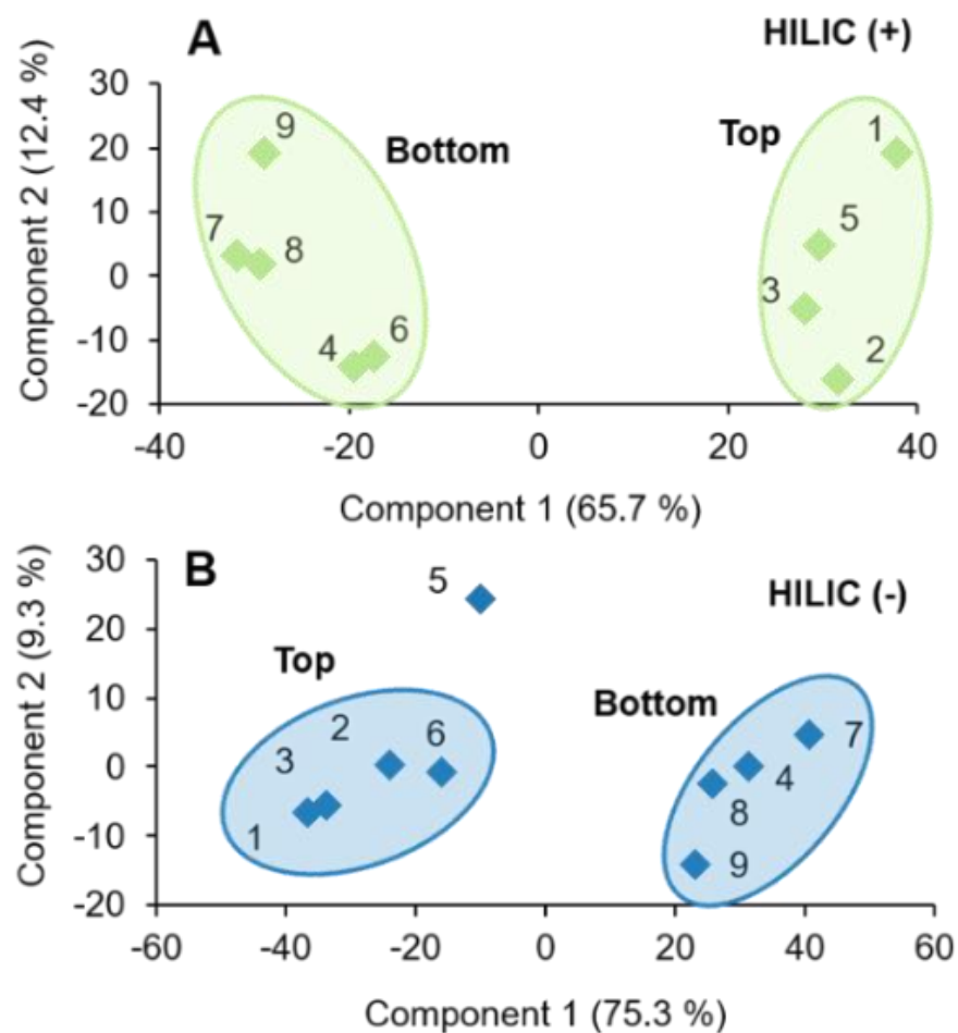
Figure 24: PCA of HQFs detected in soil water extracts analyzed by (a) HILIC (+) and (b) HILIC (-) demonstrating the sensitivity of the untargeted technique to detect subtle variations in LMW DOM with depth in these organic-rich soils
