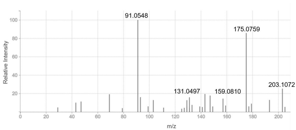
Figure 76: Corresponding database predicted MS 2 spectrum for matched compound, ethyl 2-benzylacetoacetate
