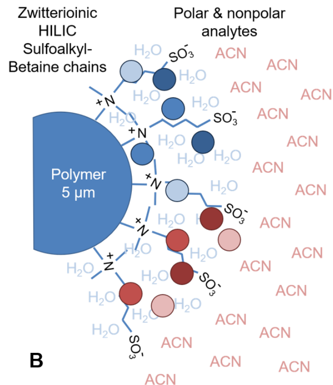
Figure 8: Schematic of (A) a C-18 RP silica bead and (B) a ZIC-pHILIC polymer bead showing the complimentary retention mechanisms where nonpolar analytes are absorbed to the C-18 chain and both polar and nonpolar analytes are partitioned into an aqueous layer formed on the surface of the zwitterionic chain.
