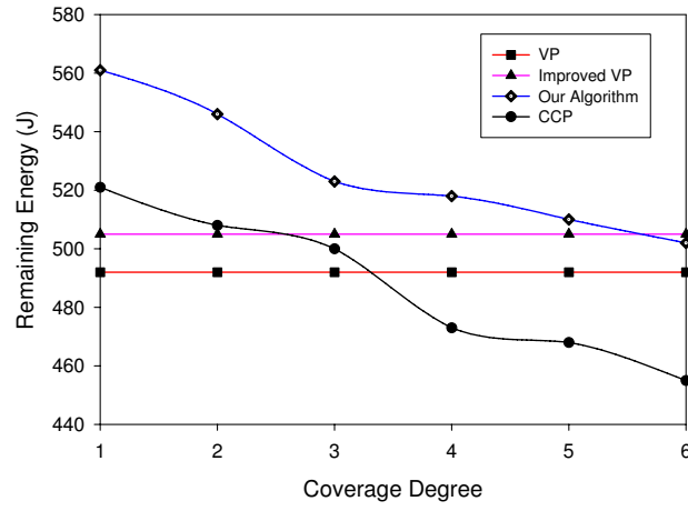
Figure 3.9: Energy Comparison with Virtual Patrol and CCP
