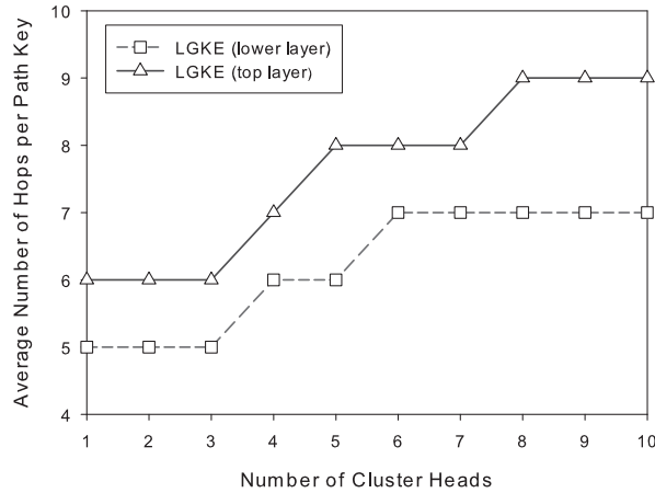
Figure 4.9: Average number of hops v.s. number of cluster heads per group. The average number of hops to establish a path key and an inter-non-neighbor-group key are given for the number of cluster heads varying from 1 to 10 in a network with 50,000 nodes with group size 100.
