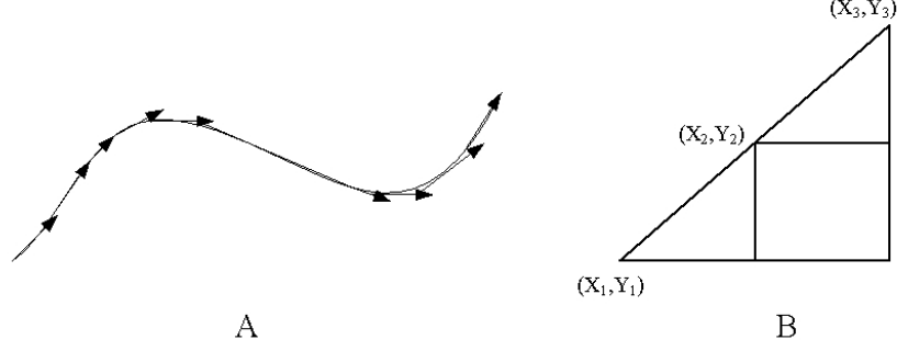
Figure 3.3: Prediction Model.
