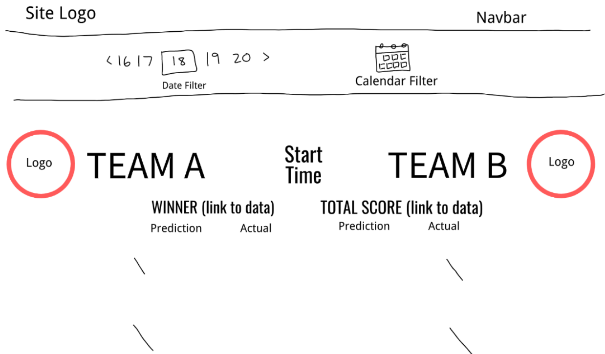
Figure 3: Dashboard Mockup
