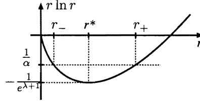
Figure 10: In the potential V(r) = \ln r
