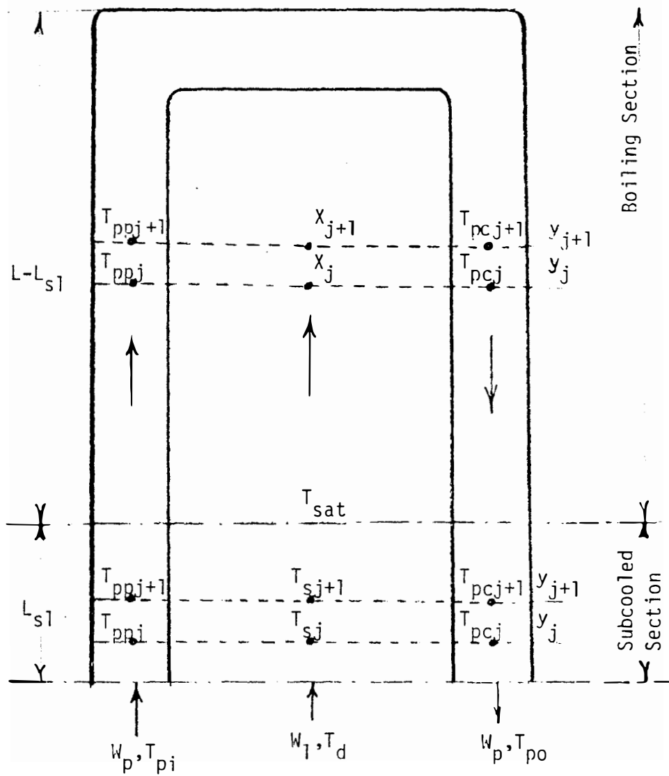
Figure IV.2 Schematic of the Effective Heat Exchange Region (Core).
