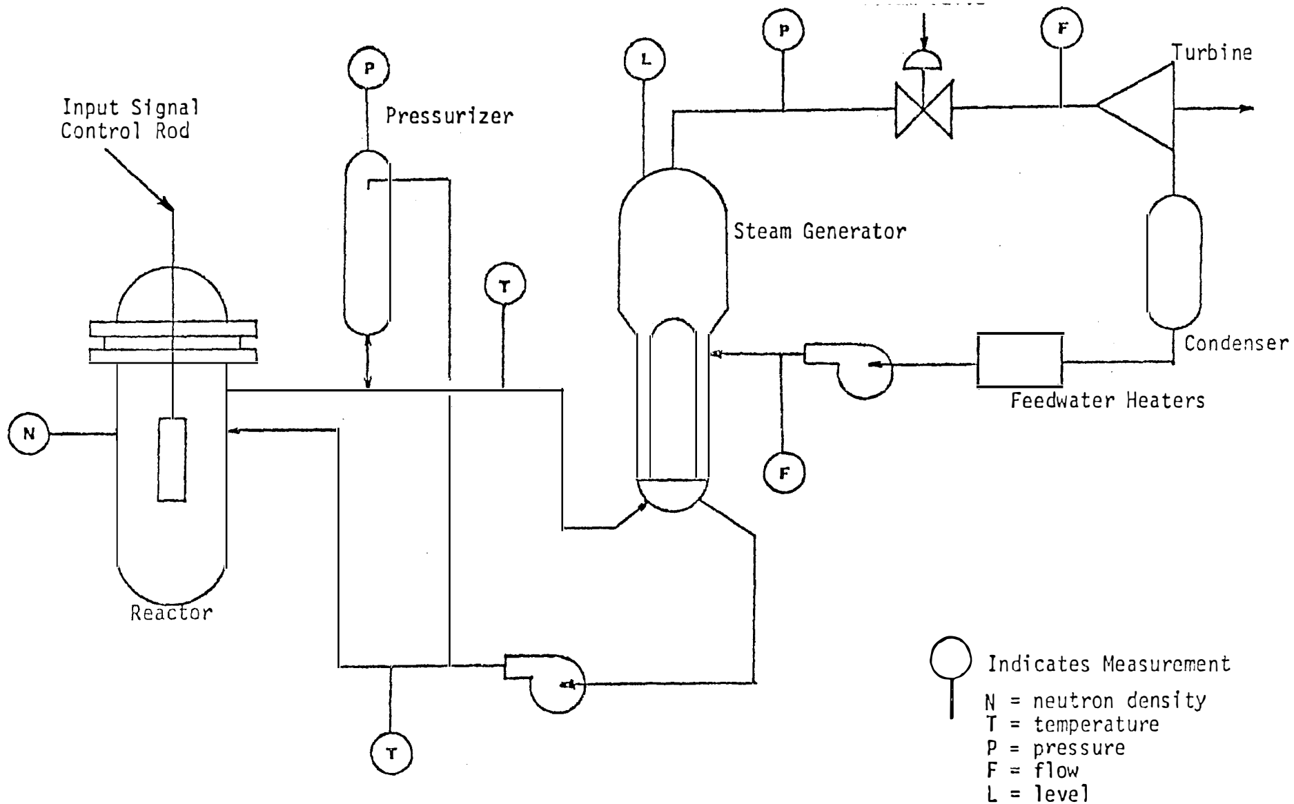
Figure V.1 Schematic of the H. B. Robinson Plant.
