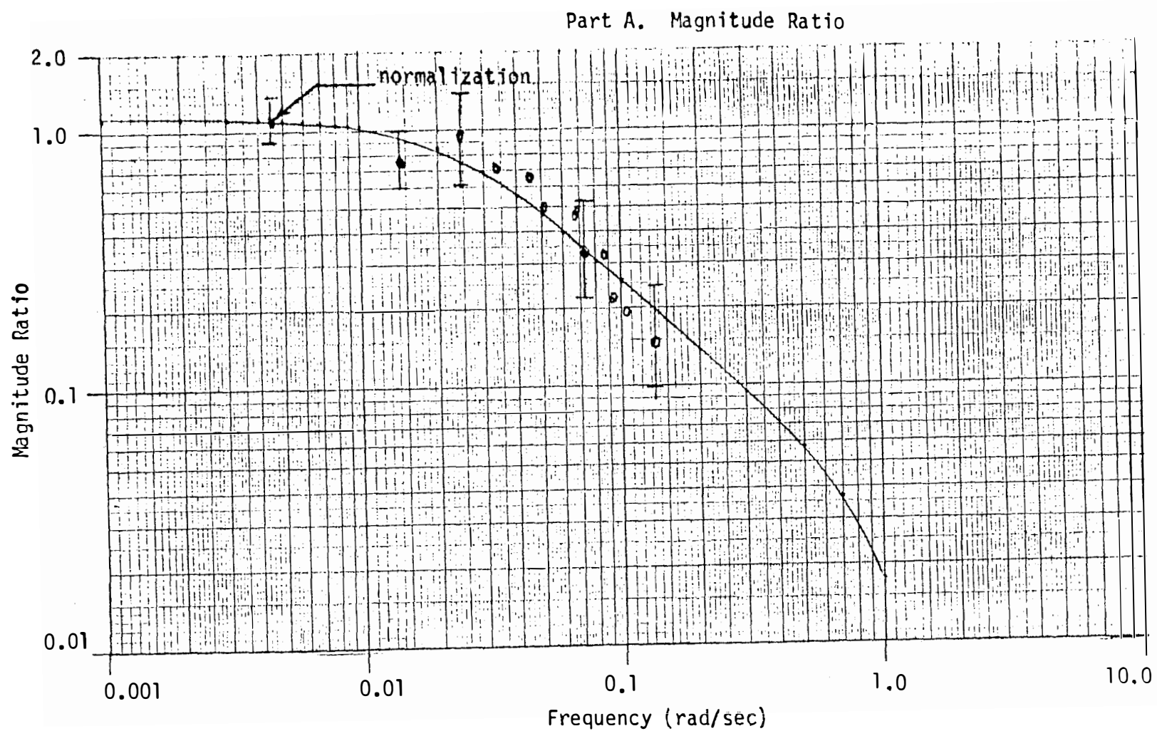
Figure V.7 Cold Leg Temperature/Steam Flow ( \delta T_{CL}/\delta W_{SO} ) Frequency Response.
