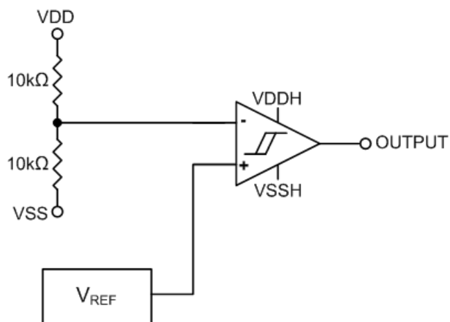
Figure 3-4: UVLO 2: V_{DD} to V_{SS} Circuit Topology
