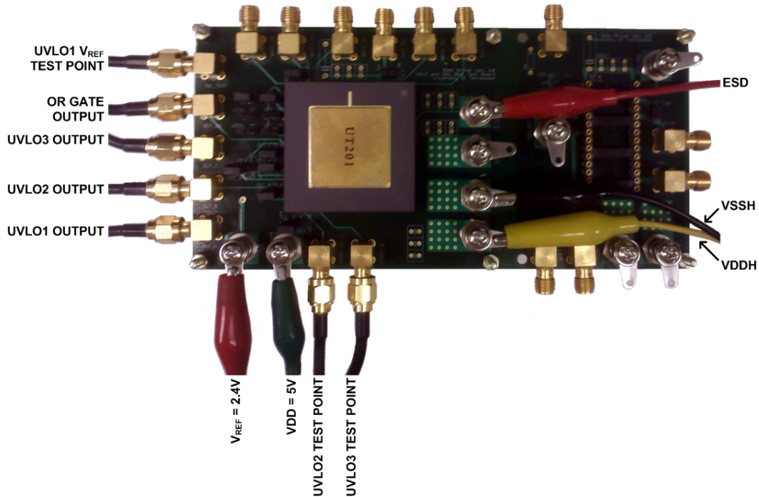
Figure 4-6: UVLO Test Set-up
