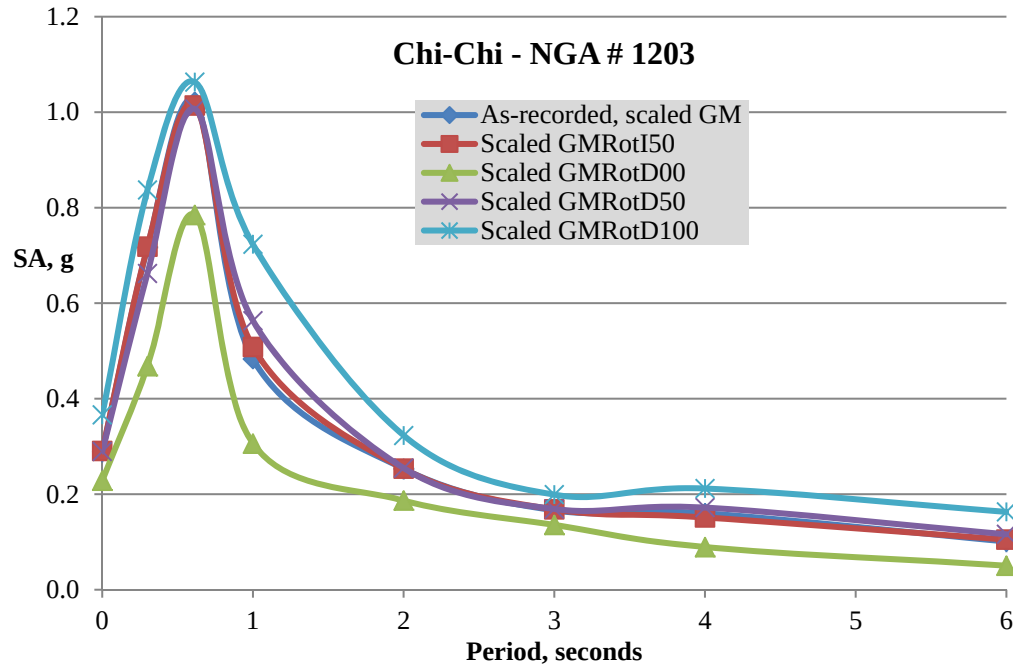
Figure D-13. GM Intensity Measures - 1203Chi-Chi
