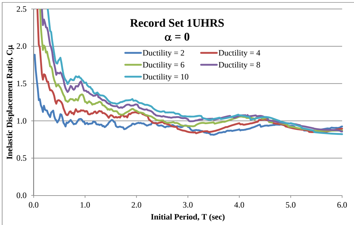
Figure F-10. Inelastic Displacement Ratio - Record Set 1UHR5 ( \alpha = 0 )
