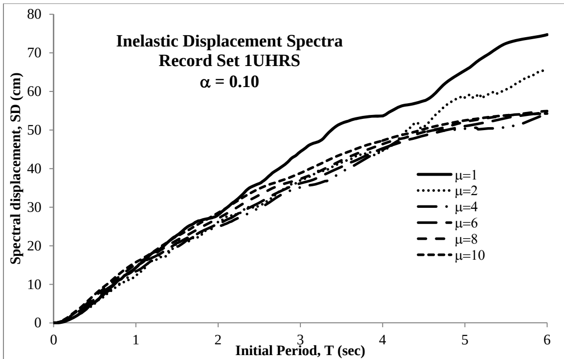
Figure F-11. Inelastic Displacement Spectra - Record Set 1UHSR ( \alpha = 0.10 )
