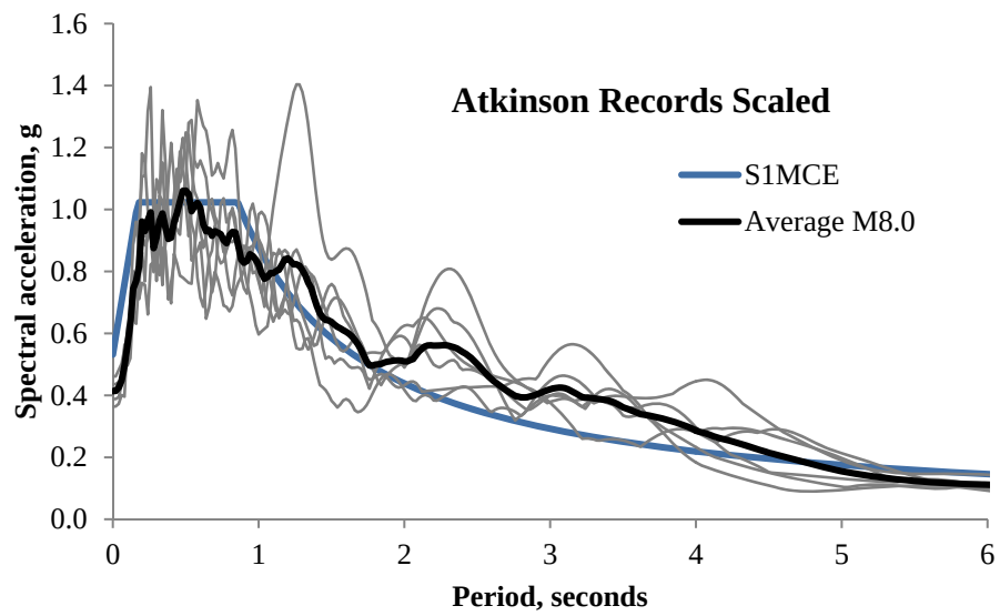
Figure E-16. Atkinson's M8.0 Records Scaled to S1MCE
