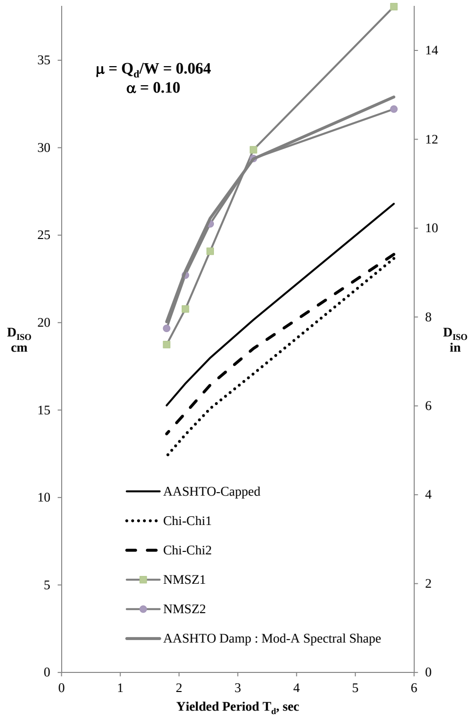
Figure G4.3-7. Proposed LRB Modifications: \mu = Q_d/W = 0.064
