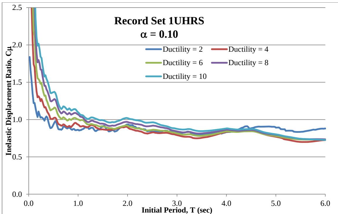
Figure F-12. Inelastic Displacement Ratio - Record Set 1UHSR ( \alpha = 0.10 )
