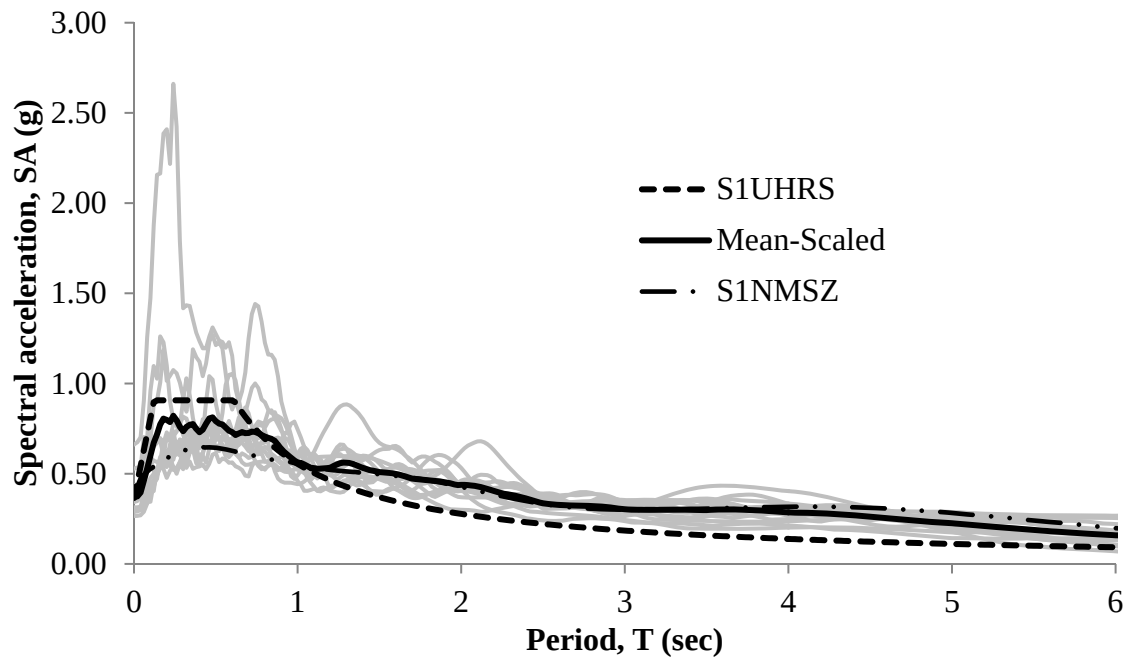
Figure 3.7-8. Acceleration Spectra - Record Set No. 1NMSZ
