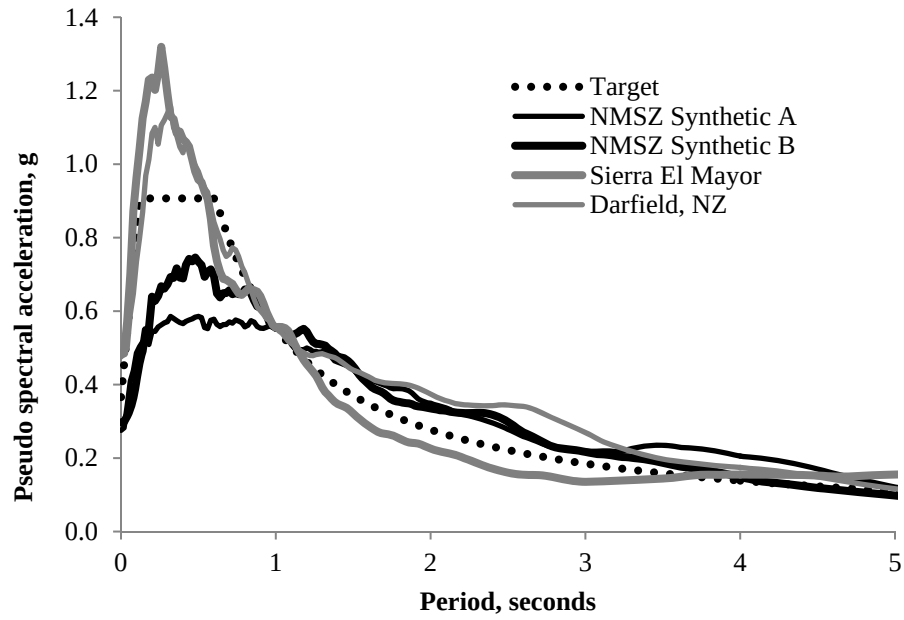
Figure G3.6-7. Site 1 NMSZ Spectra vs. Darfield Spectra - Acceleration
