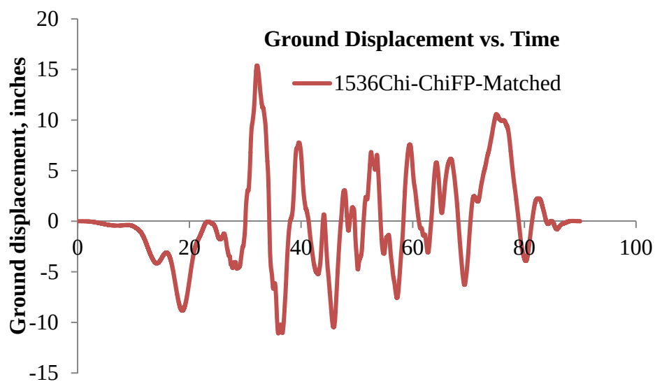
Figure 1.6.4-4. Chi-Chi Displacement History (NGA 1536FP Modified)
