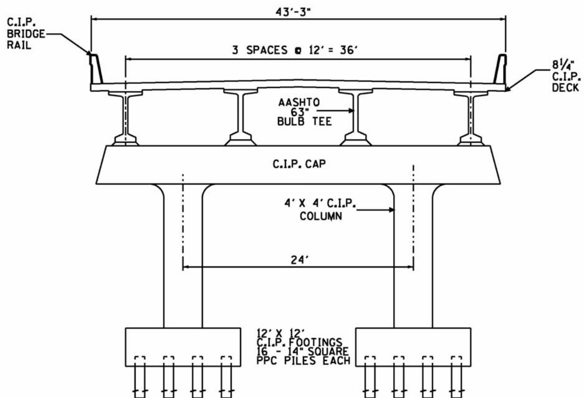
Figure G1.4-9. Cross-Section - Bridge No. 5
