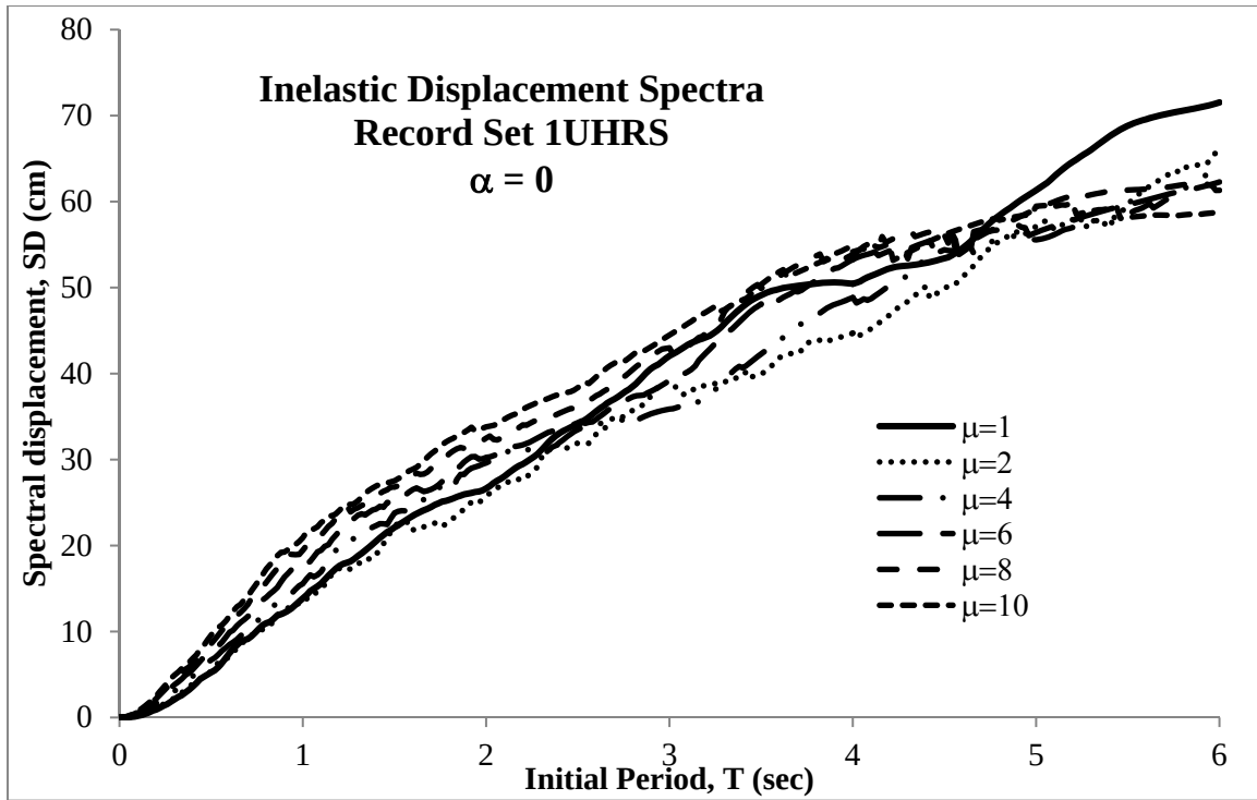
Figure F-9. Inelastic Displacement Spectra - Record Set 1UHR5 ( \alpha = 0 )
