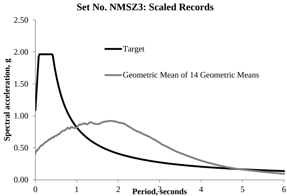
Figure G3.6-10. Acceleration Spectra - Set NMSZ-3
