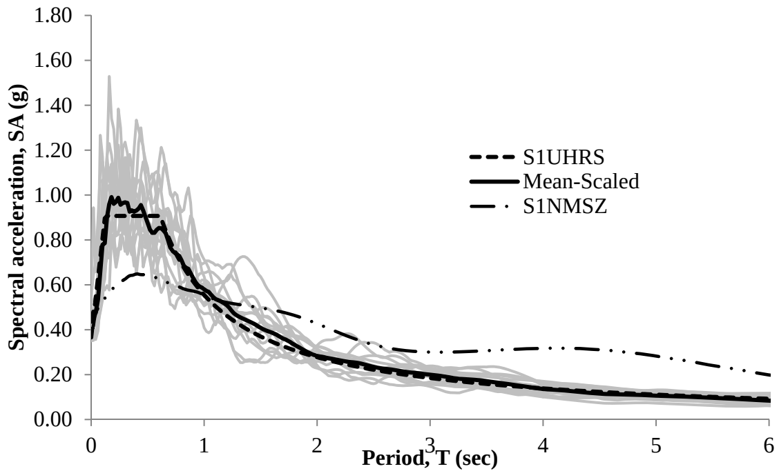
Figure 3.7-7. Acceleration Spectra - Record Set No. 1UHRS
