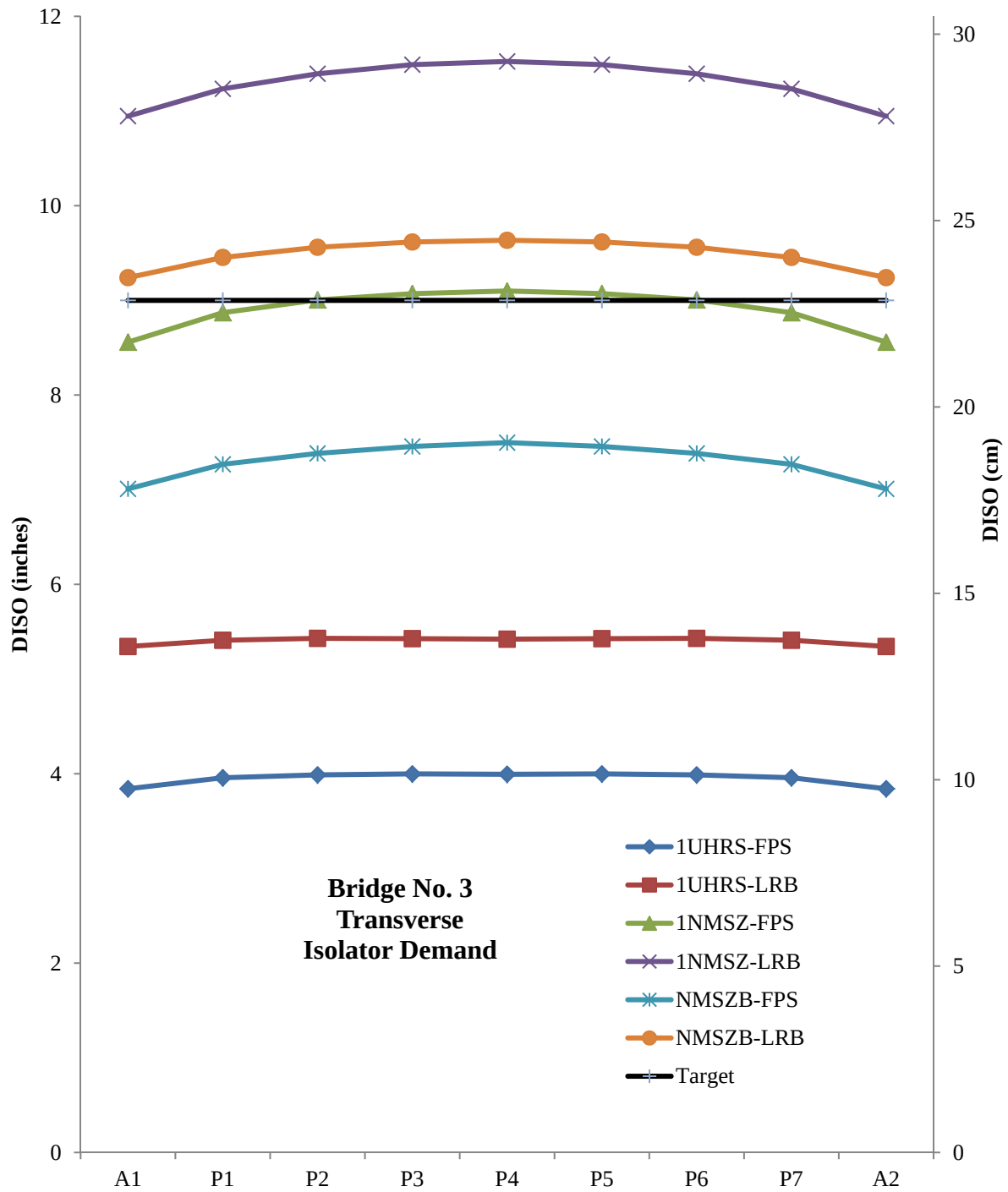
Figure G7.2.5-7. Isolator Demand - Bridge No. 3 (Transverse)
