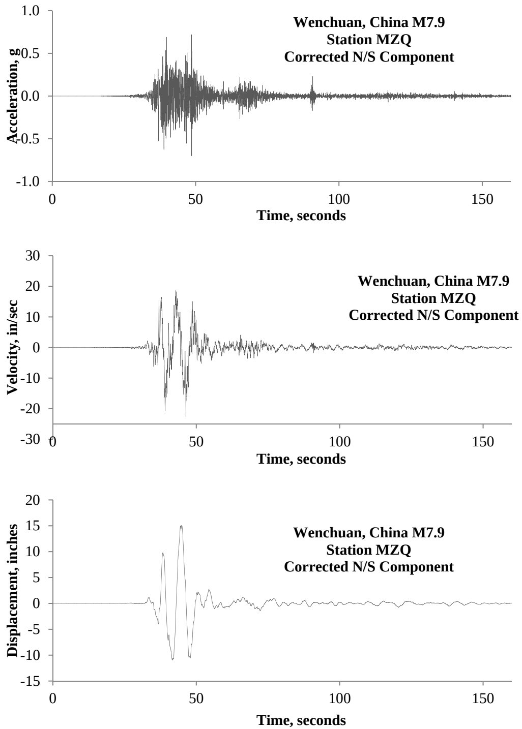
Figure G3.1.2-3. Corrected A,V,D: MZQ N/S component
