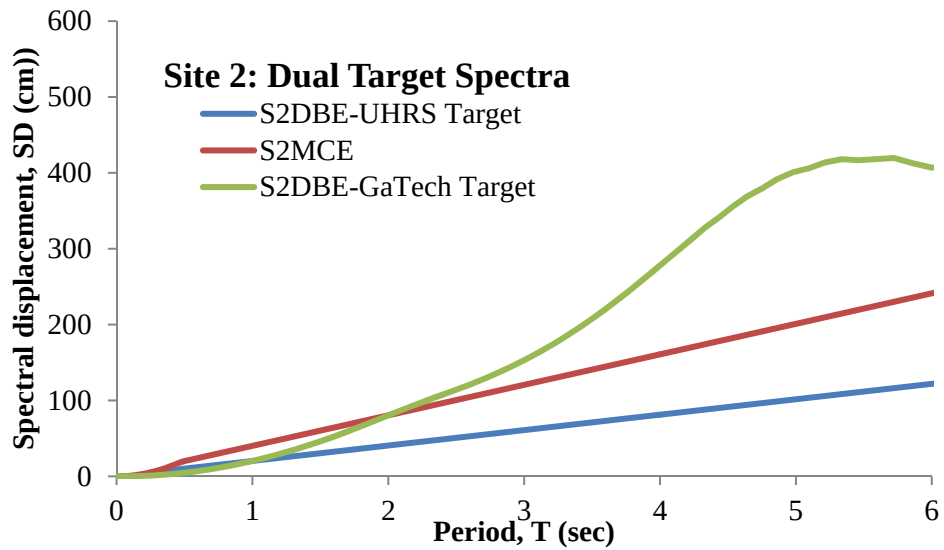
Figure 3.7-6. Dual Target Displacement Spectra - Site No. 2
