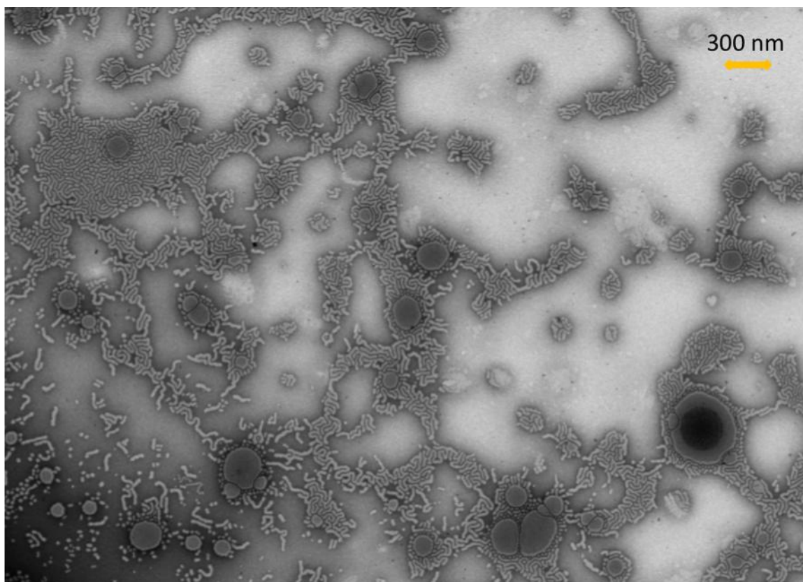
Figure 14. Electron micrograph of PEO-PCL filomicelles in water on day 11.
