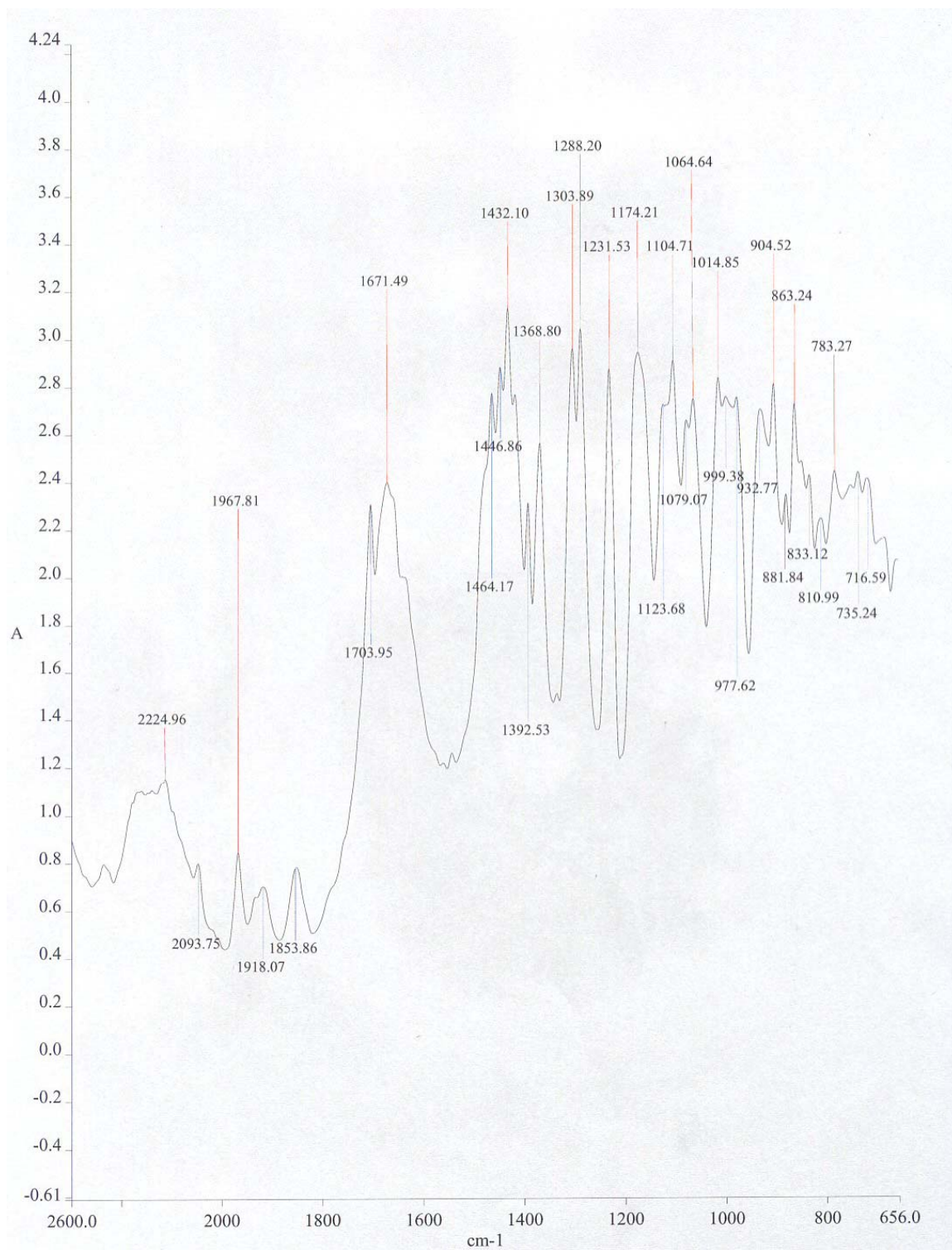
Figure 14: Average spectrum for NMMO samples. Series of distinguishing peaks between 1100 and 1475 \text{cm}^{-1}
