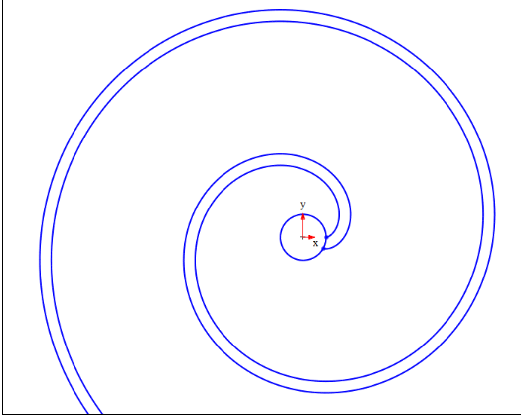
Fig. 3.4. Adjacent Involute Constant Offset. The curve with the upper origin point has \alpha = \theta where \theta_0 = 0 . The curve with the lower origin has \alpha = \theta + 1/2 where \theta_0 = -1/2 .
