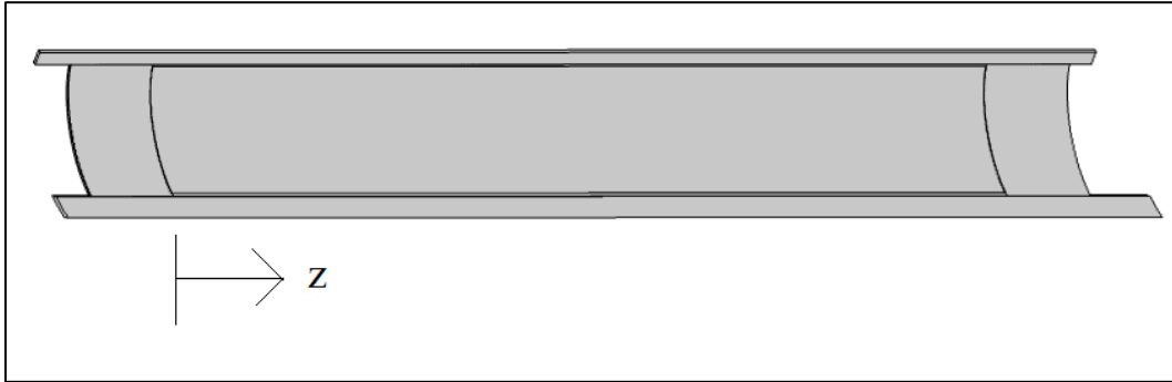
Fig. 5.3. Solid Geometry Assembly. Flow direction is in the +z -direction. The inner side plate is shown on top in this figure. The geometry in between is the fuel plate. Coolant geometry components are not pictured.
