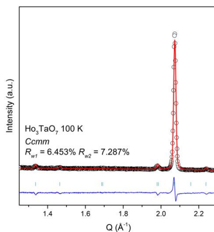
Figure 5.6: Low-Q region of POWGEN' high-resolution neutron diffraction pattern of \text{Ho}_3\text{TaO}_7 measured at 100 K (black circles) and modeled (red curve) using Ccmm space group. The blue curve represents the difference curve between measurement and the model fit, with R_{w1} and R_{w2} being the fit reliability factors. Cyan ticks indicate the expected Bragg peak positions according to the crystal structure model.
