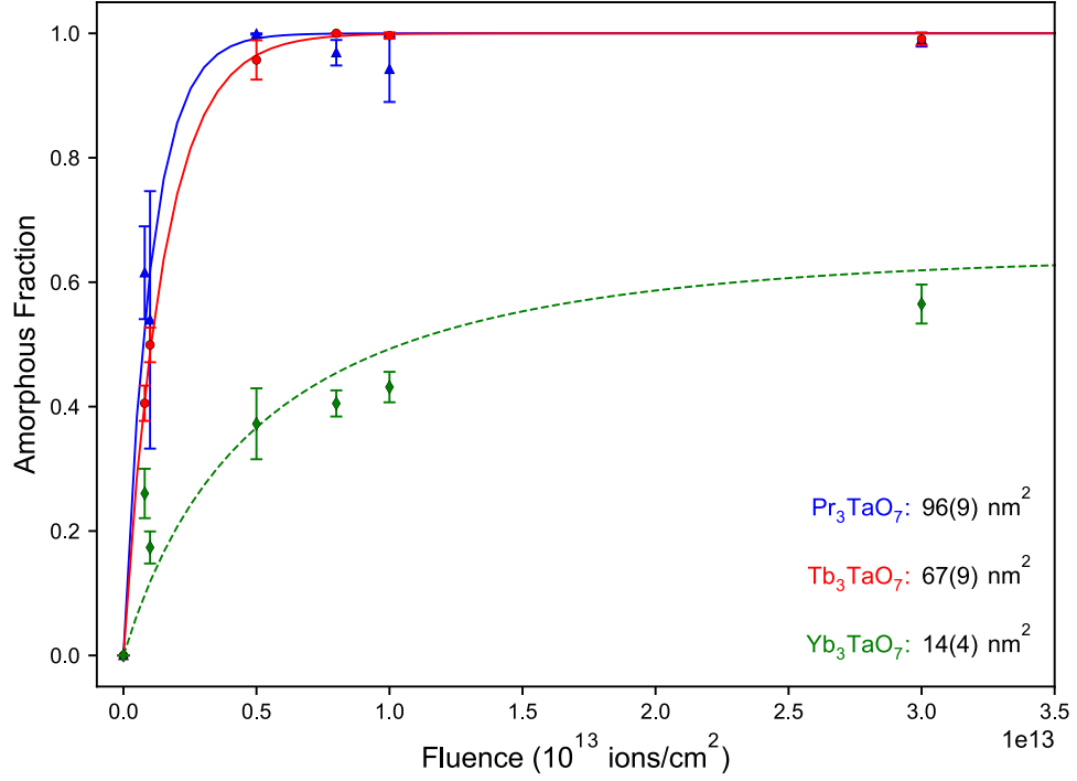
Figure 6.2: Fits of the single impact model (Eq. 3.5.) to the ion-induced amorphous fractions for Pr _3 TaO _7 , Tb _3 TaO _7 and track overlap model (Eq. 3.6.) for Yb _3 TaO _7 . Uncertainties in the amorphous fractions arise from the deconvolution of multiple XRD patterns, and uncertainties in the amorphous cross section arise from fitting of the models to the amorphous fractions.
