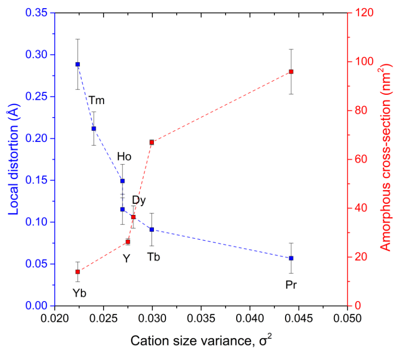
Figure 6.14: Quantified local distortion parameter for the pristine A_3BO_7 (blue datapoints, data reproduced from [45]) overlayed against the amorphous cross-section for irradiated compounds (red datapoints). Colored lines serve as guides for the eyes.
