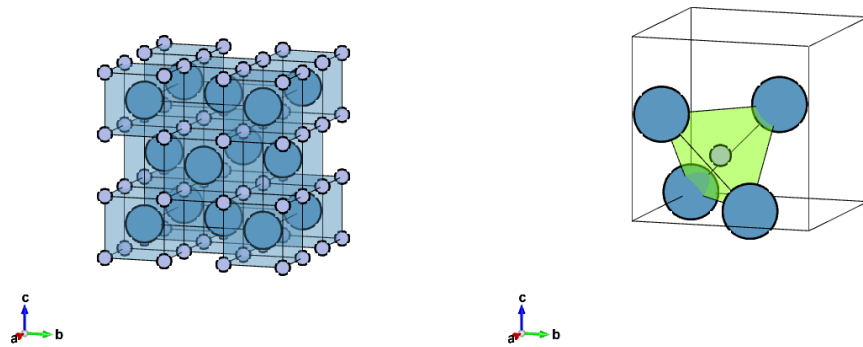
Figure 2.1: (Left) \text{CaF}_2 with Fm-3m structure. Light blue spheres are Ca cations, while light purple spheres are F anions. Light blue cubes designate \text{CaF}_8 polyhedra. (Right): \text{Ca}_4\text{F} cationic tetrahedra, shown in the light green shade, black lines designate the cubic unit cell. Ca cations shown are located at the edge and three faces of the cubic unit cell.
