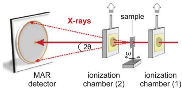
Figure 3.5: Schematics of X-ray diffraction experiment at beamline HPCAT 16-BM-D of the Advanced Photon Source. Figure is reproduced from ref [50].
