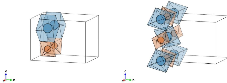
Figure 2.5: (Left): The first \text{CaO}_8\text{-SbO}_6 layer of weberite structure. \text{SbO}_6 and \text{CaO}_8 polyhedra forming chains along [100] are visible. (Right): Alternating \text{CaO}_8\text{-SbO}_6 layer of \text{Ca}_2\text{Sb}_2\text{O}_7 weberite with Imma structure. In both figures, Light blue spheres are Ca cations, brown spheres are Sb cations. In respective shades are 8-coordinated distorted cubes and 6-coordinated octahedra. Oxygen atoms are not shown.
