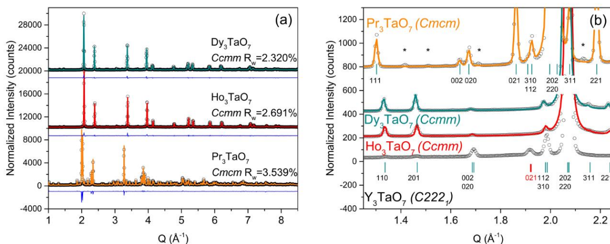
Figure 5.2: (a) Stacked high-energy synchrotron X-ray diffraction patterns for A_3TaO_7 (A = Pr, Dy, Ho) as measured (black circles) and modeled (orange, cyan and red curves). Blue curves represent the difference between measurement and calculated model (space groups Cmcm and C222_1 ). The reliability factor ( R_w ) is reported for every sample. Diffraction patterns are offset by values of 10'000 and 20'000 respectively. (b) Expanded view of the low-Q range of (a) using the same color labeling, along with diffraction data of Y_3TaO_7 (black circles), which serves as reference measurement. Cyan ticks represent diffraction conditions allowed in (top) Cmcm and (bottom) C222_1 space groups. Asterisks (*) mark the PrTaO_4 impurity phase reflections for Pr_3TaO_7 . The red tick mark at \sim 1.93 \text{\AA}^{-1} indicates the location of the (021) diffraction peak, which serves as space group distinction between C222_1 and Cmcm (and it is only allowed for C222_1 ). Diffraction patterns are offset by values of 200, 400 and 800 respectively.
