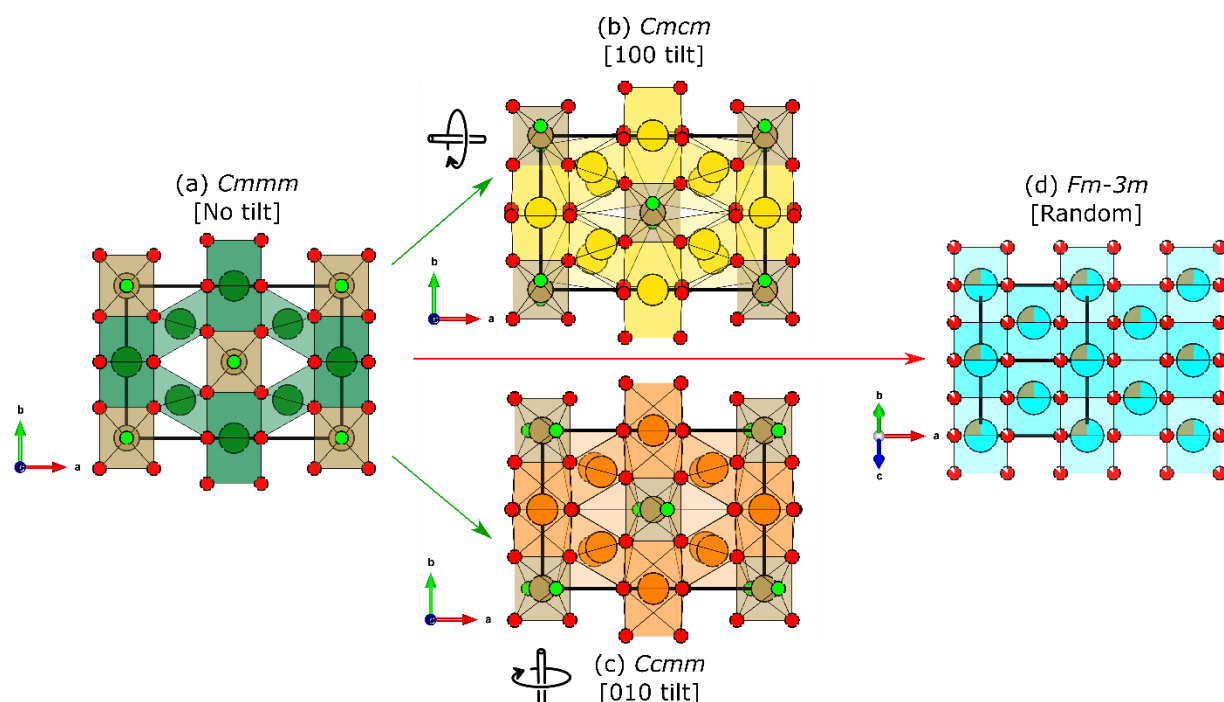
Figure 5.1: Relations among the three structural families of A_3TaO_7 weberite-type oxides (b,c,d). The structures are shown with the relation to the single c-layer parent prototype structure. Thick solid black lines represent the respective unit cells. (a) Cmmm prototype model with A-site cations shown as green spheres, (b) Cmcm structural model with large radii A-site cations shown as yellow spheres, (c) Ccmm structural model with medium radii A-site cations shown as orange spheres and (d) Fm-3m structural model with small radii A-site cations shown as cyan spheres. Oxygen anions and Ta cations are shown in all four structures as red and brown spheres, respectively. Oxygen anions highlighted as smaller lime green spheres and displaced according to different tilt systems. The tilt systems of the (a) single layer Cmmm prototype structure produce either the bilayer structure (b) Cmcm with [100] tilt, or the (c) Ccmm with [010] tilt, as represented by black loops around the rotation axes. The white sectors within red spheres in (d) denote the partial occupancy of oxygen sites in the Fm-3m model, and mixed brown/cyan spheres represents a randomization of cations across cation sites. All coordination polyhedra are shown according to the color of their respective cations. Structures are projected along their conventional directions: (a,b,c) along [001]_W and (d) [011]_F with W and F subscripts denoting the weberite-type and defect-fluorite lattices, respectively.
