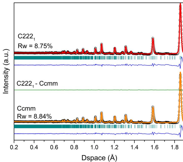
Figure 4.1: Neutron diffraction pattern of \text{Y}_3\text{TaO}_7 (NOMAD detector bank 4) as measured (black circles) and modeled using Ccmm (orange line, bottom profile) and C222_1 (red line, top profile) space groups. The blue lines represent the difference curves between the experimental data and the model fit with the R_w values being the goodness-of-fit parameter. The green line represents the difference in diffraction profiles between the C222_1 and Ccmm model, respectively.
