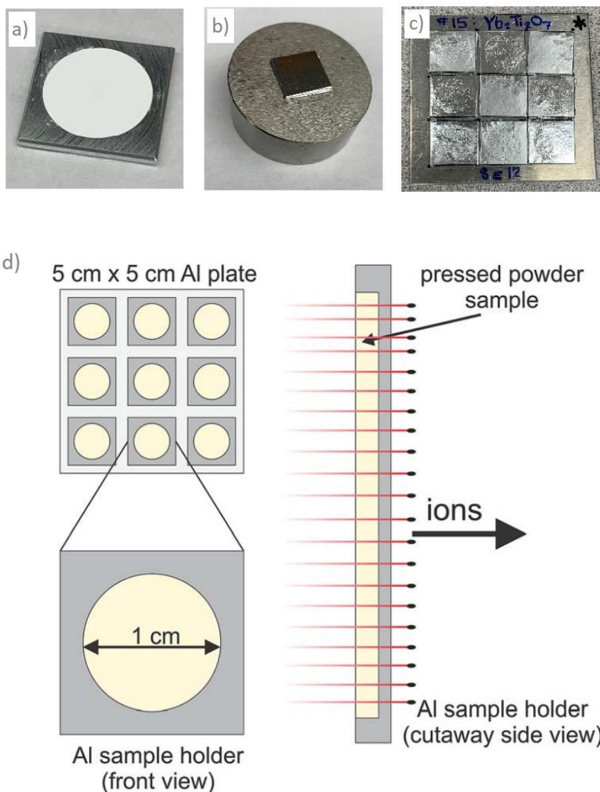
Figure 3.3: Sample holders used for larger mass ion irradiation experiments. (a) Powder sample is spread into cylindrical indentation of aluminum holder. (b) individual aluminum holder is covered in aluminum foil. (c) set of nine aluminum holders are mounted on 5×5 cm aluminum plate. (d) schematics of sample geometry for irradiation. Image taken from ref [47].
