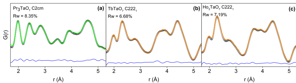
Figure 5.13: A segment of very local (1.7-5.3 Å) neutron pair distribution functions showing 1 st and 2 nd nearest neighbor correlations of weberite-type A_3\text{TaO}_7 ( A=\text{Pr, Tb, Ho} ) modelled with (a) C2cm and (b, c) C222_1 space groups, respectively. Black circles represent the experimental data while green and orange curves are fits with the respective models. Difference curves between data and models are displayed in blue.
