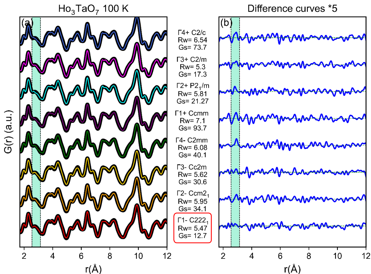
Figure 5.11: (a) Neutron pair distribution functions of weberite-type \text{Ho}_3\text{TaO}_7 measured at 100 K and modelled with 7 displacive small-box models in addition to the Ccmm long-range space group. Black circles represent the experimental data. Red, orange, gold, green, purple, cyan, magenta and royal blue lines are fits of the respective models. (b) Difference curves (multiplied by a factor 5) between as-collected data and respective models in the r -range between 1.7 – 12 Å. The turquoise shaded area enclosed by the vertical dashed lines between 2.5 and 3 Å highlights the region most sensitive to the O-O atomic correlations. The red frame around the C222_i space group highlights the best structural model to describe the PDF of \text{Ho}_3\text{TaO}_7 .
