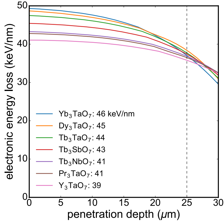
Figure 3.2: Energy loss profiles of 946 MeV ^{197}\text{Au} ions in the weberite-type compositions studied here as calculated with SRIM. Dashed vertical line denotes typical sample depth in the holder. The number given in the legend indicates the mean energy loss throughout the thickness of the sample. In all cases, the electronic energy loss (shown as colored lines) is over two orders of magnitude larger than the nuclear energy loss (not shown) throughout the sample volume.
