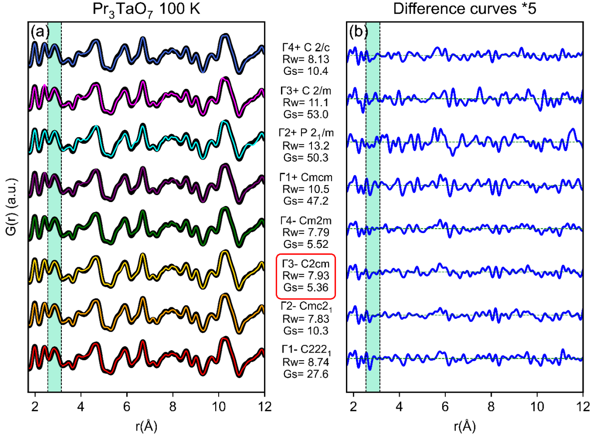
Figure 5.10: (a) Neutron pair distribution function (PDF) of weberite-type \text{Pr}_3\text{TaO}_7 measured at 100 K (black circles) and refined with the long-range Cmcm space group (purple) and with the models derived at the Brillouin zone center (red, orange, gold, green, cyan, magenta, and royal blue) of Cmcm . The four non-centrosymmetric models ( \Gamma_{1-4}^- ) are the bottom curves and the four centrosymmetric models ( \Gamma_{1-4}^+ ) are the top curves. (b) Difference curves (multiplied by a factor 5) between as-collected data and respective models in the r -range between 1.7 – 12 Å. The turquoise shaded area enclosed by the vertical dashed lines between 2.5 and 3 Å highlights the region most sensitive to the O-O atomic correlations. The red frame around the C2cm space group highlights the best structural model to describe the PDF of \text{Pr}_3\text{TaO}_7 .
